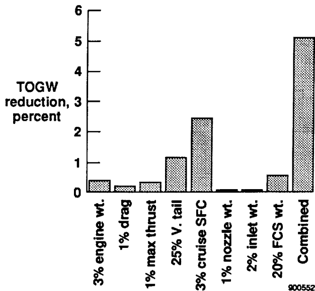
Figure 10. Effect of integrated control technology improvements on generic HSCT TOGW.
