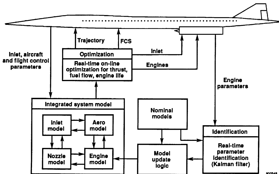
Figure 6. Conceptual HSCT performance-seeking control block diagram.
