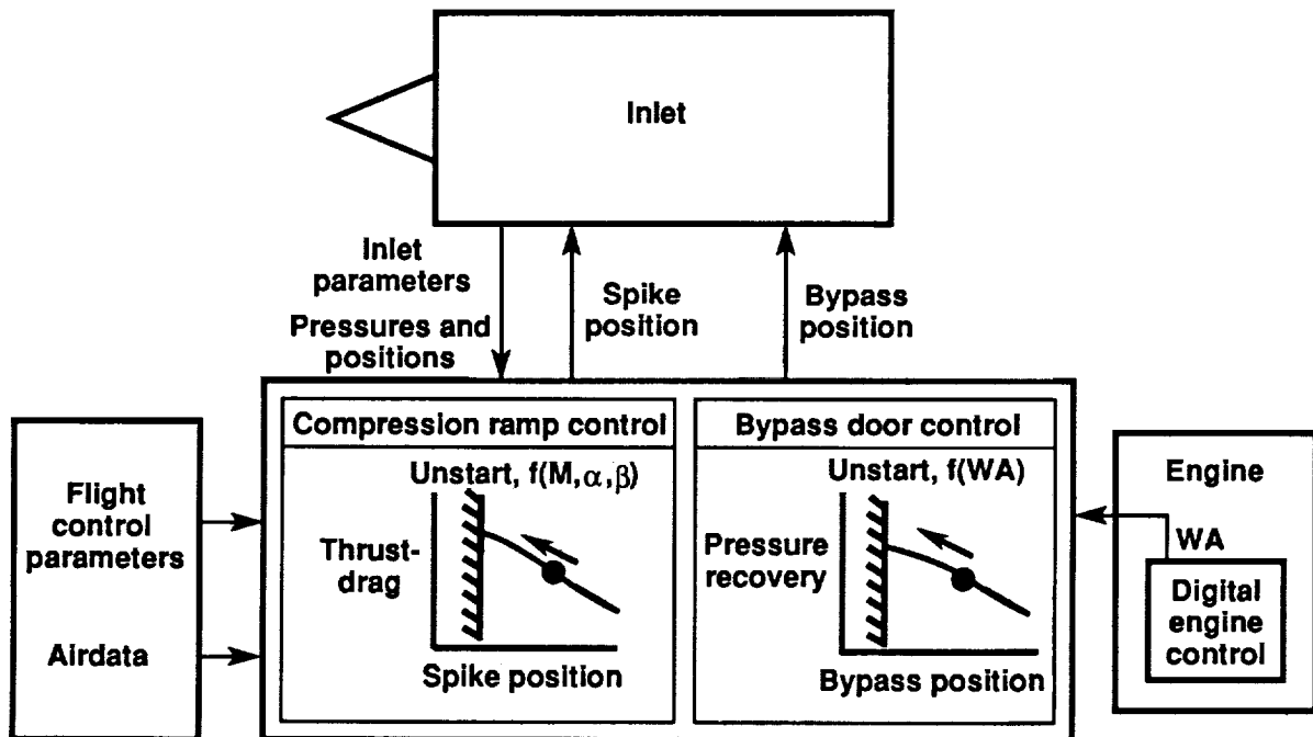
Figure 4. Conceptual integrated inlet-engine-flight-control mode.
