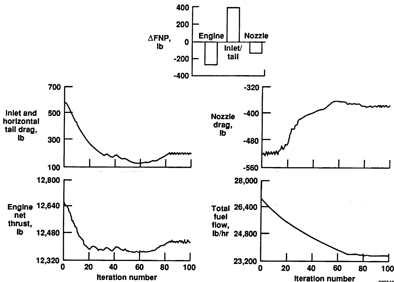
Figure 7. Predicted performance-seeking control optimization for minimum fuel flow at constant thrust, F-15 HIDECA airplane, Mach 1.9, 45,000 ft, power level angle = 120.
