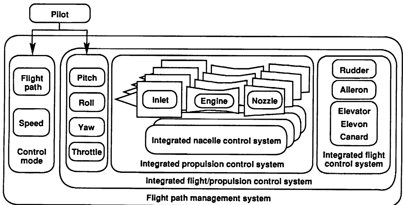
Figure 2. High-speed civil transport integrated control concept.
