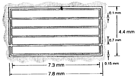
Fig. 7. Drawing of an evaporation mask used to fabricate HgI 2 detector arrays.
