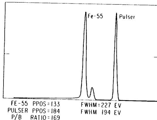
Fig. 2. ^{55}Fe X-ray spectrum obtained with a HgI_2 detector at room temperature and a cooled FET transistor at -30^\circ C . The spectrum from an electronic pulser is also shown at higher energy.
