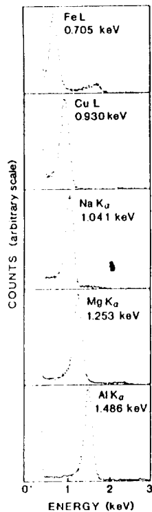
Fig. 4. Composite of low-energy X-ray spectra.
