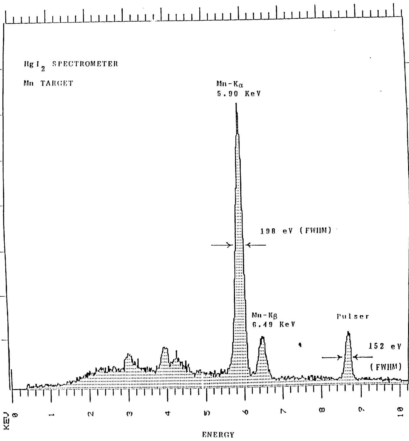
Figure 1. X-ray spectrum obtained with HgI 2 detector from manganese target
