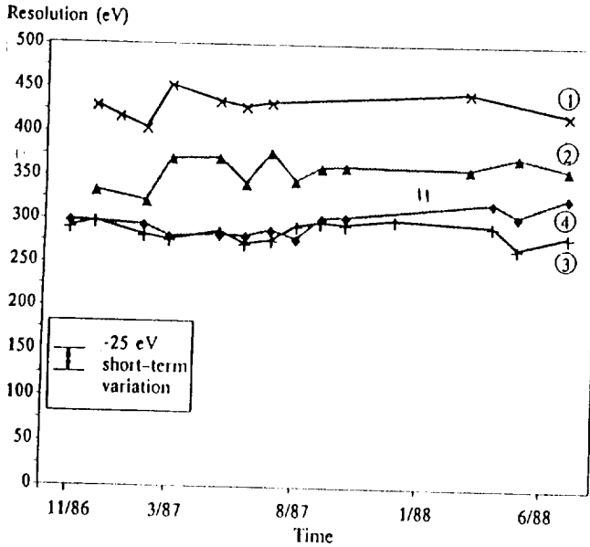
Figure 4. The long-term energy resolution variation for four tested HgI 2 detectors. The energy resolution (FWHM) was measured for the Mn k α line. Curves 1 to 4 correspond to detectors in chambers #1 to #4, respectively.
