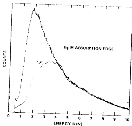
Fig. 2. Two X-ray pulse height spectra of bremsstrahlung radiation from carbon targets. The two spectra were obtained with different HgI 2 detectors.
