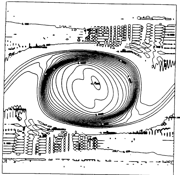
Figure 58: Plot of product concentration contours, Ze = 20 , t^* = 2.25 .
