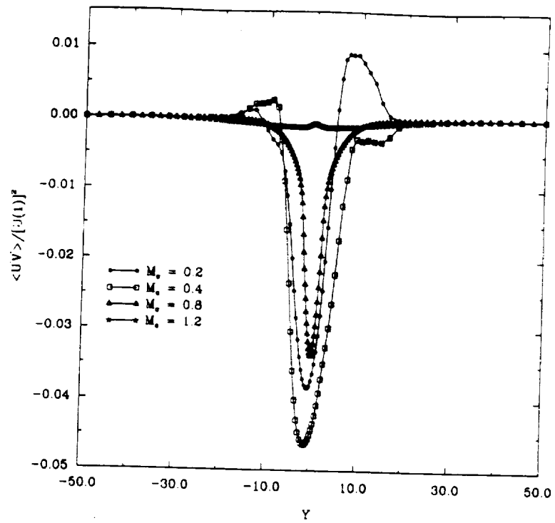
Figure 10: Profiles of normalized Reynolds stress for different values of the convective Mach number at time t^* = 8 .
