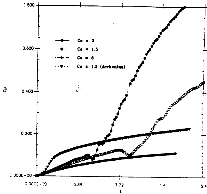
Figure 34: Normalized product thickness versus normalized time for various values of the heat release parameter.
