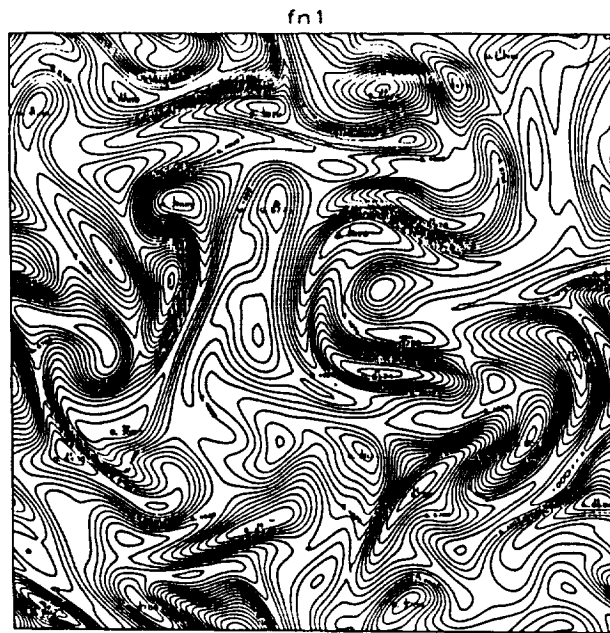
Figure 3. Contour plot of species A concentration for high compressible case.
