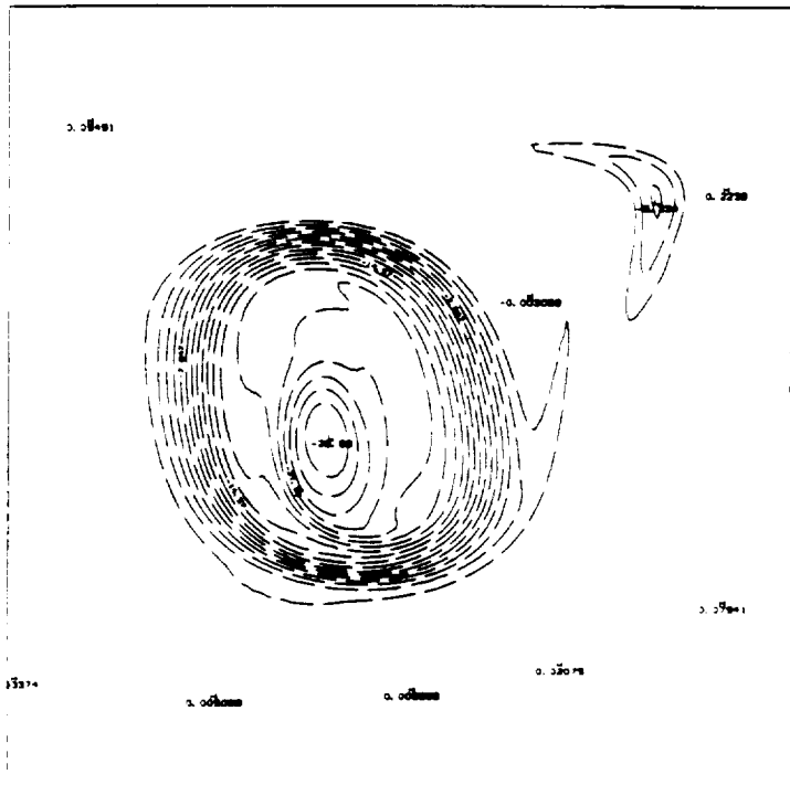
Figure 25: Plot of vorticity contours at time t^* = 8 , C_e = 0
