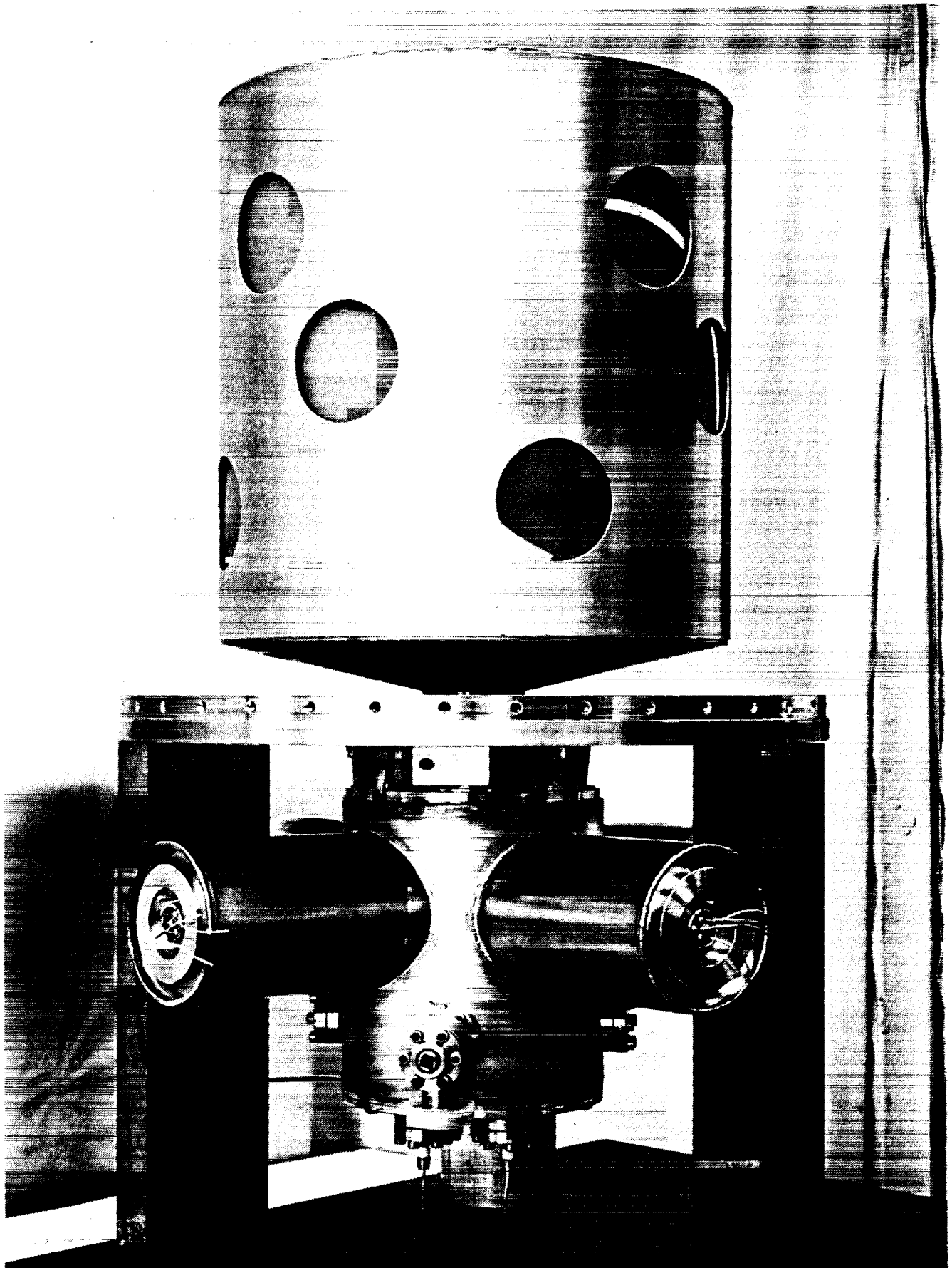
Figure 2 Vacuum Manifold with Sorption Pump Enclosures (Lower half of photo)
