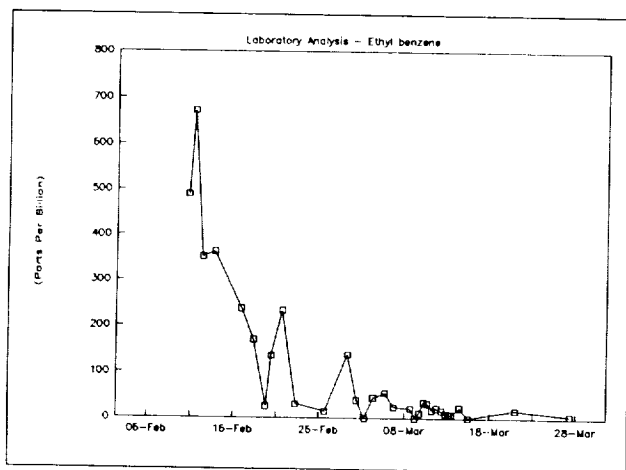
Figure 9. Ethyl benzene levels during the Test Module human closure March 8-13, 1989 including unmanned closure phases pre- and post-human habitation.
