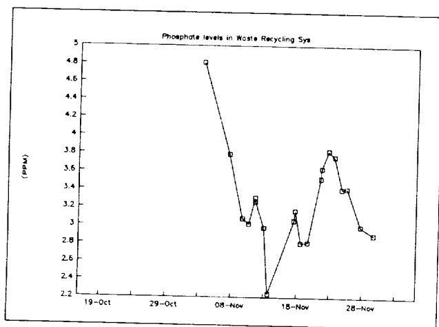
Figure 14. Phosphate levels in aquatic plant/microbial waste recycling system during Test Module human closure November 2-23, 1989 including unmanned closure phases post-human habitation.
