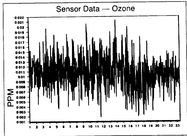
Figure 4. Ozone levels during Test Module human closure November 2-23, 1989.
