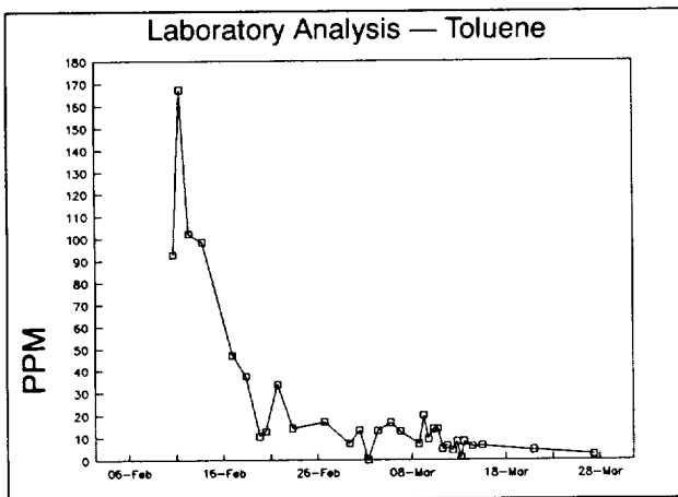
Figure 7. Toluene levels during Test Module human closure March 8-13, 1989 including unmanned closure phases pre- and post-human habitation.
