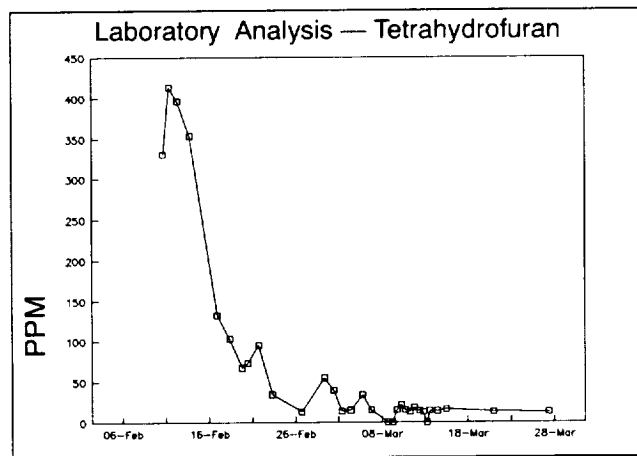
Figure 8. Tetrahydrofuran levels during Test Module human closure March 8-13, 1989 including unmanned closure phases pre- and post-human habitation.
