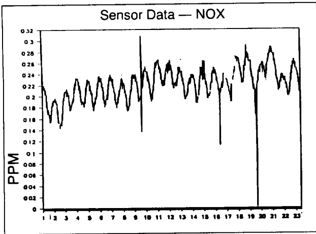
Figure 3. NOx levels during Test Module human closure November 2-23, 1989.
