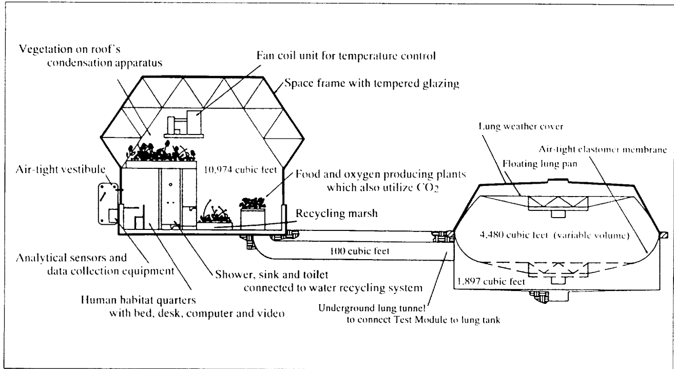
Figure 1. Biosphere 2 Test Module System Schematic. Surface area for plant growth area includes mezzanine platforms and areas within hollows of the space frame. (Copyright 1987. Space Biospheres Ventures.)
