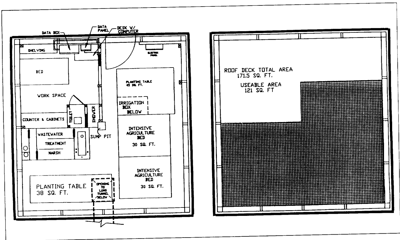
Figure 12. Biosphere 2 Test Module Floor Plan (excluding lung) during the "Human in Ecosystem" experiments conducted in September 1988, March 1989, and November 1989. (Copyright 1988, Space Biospheres Ventures.)
