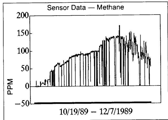
Figure 6. Methane levels during Test Module human closure November 2-23, 1989 including unmanned closure phases pre- and post-human habitation.
