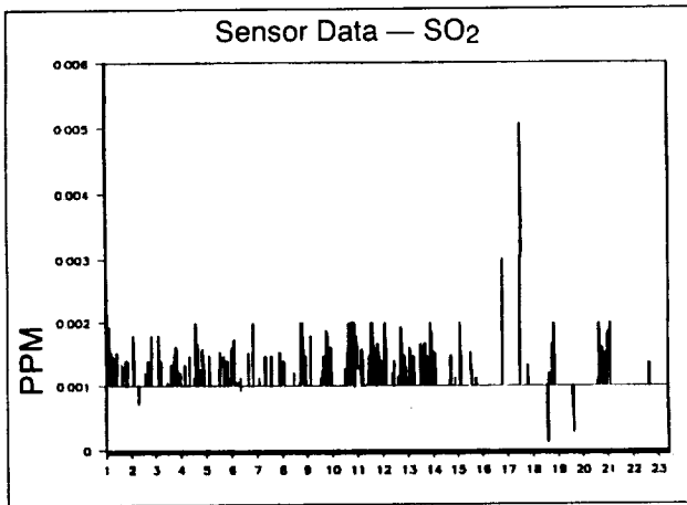
Figure 5. Sulfur dioxide levels during Test Module human closure November 2-23, 1989.
