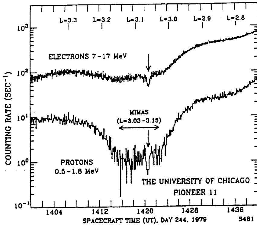
Figure 15: The "Mimas" microsignature as observed inbound in the "7-17 MeV electron" and "0.5-1.8 MeV proton" counting rates from the University of Chicago experiments on Pioneer 11 [Simpson et al. , 1980a,b]. Increases in both rates on each side of the Mimas sweeping region are most likely due to background from high energy protons. This feature was also detected in the Pioneer 11 data of Van Allen et al. [1980a,b,c]. No corresponding feature was detected outbound.
