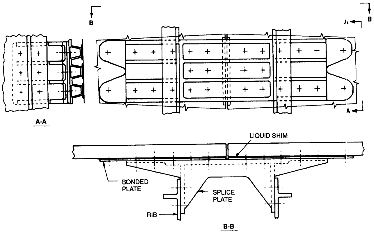
FIGURE 56. TWO-RIB CONCEPT
