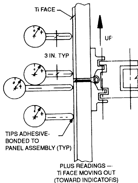
FIGURE 14. TENSION TEST FOR LARGE SLIDING-JOINT PANEL ASSEMBLY (24 BY 30 IN.) AT COLD (-65°F) CONDITION (WITH ADDITIONAL RIB CONSTRAINT)
