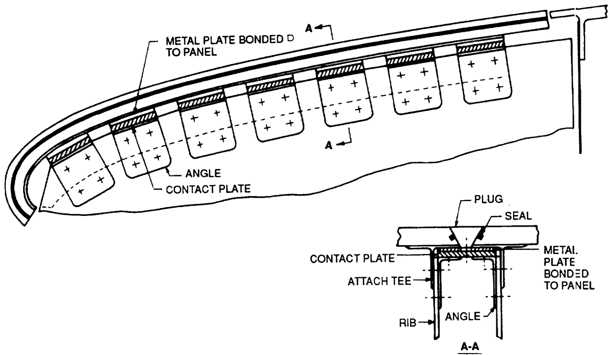
FIGURE 57. EXPANSION CONCEPT
