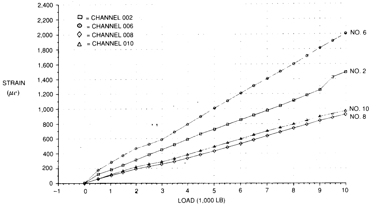
FIGURE 156. COMPOSITE FLANGE TENSION TEST AT -65°F — STRAIN GAGE READINGS
