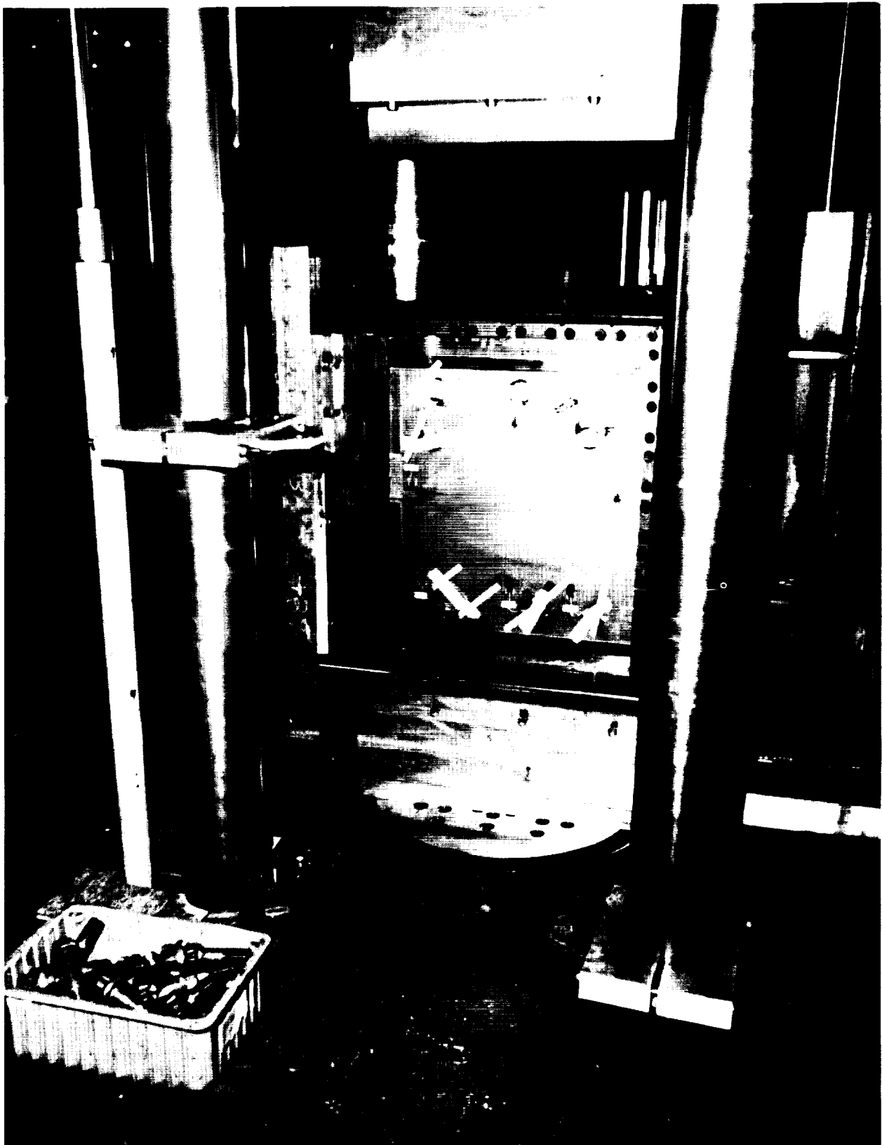
FIGURE 118. CLOSE-UP OF TEST SETUP FOR COMPRESSION TEST OF LARGE SLIDING-JOINT PANELS — ROOM TEMPERATURE CONDITION — TITANIUM SIDE
