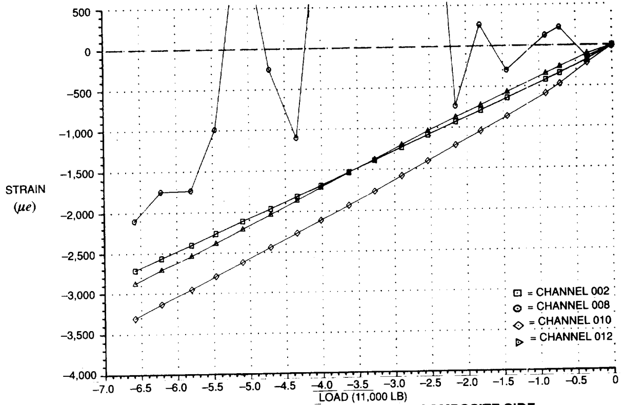
FIGURE 25. COLD COMPRESSION ( -65^{\circ}F ) — COMPOSITE SIDE, LARGE SLIDING JOINT — STRAIN GAGE READING
