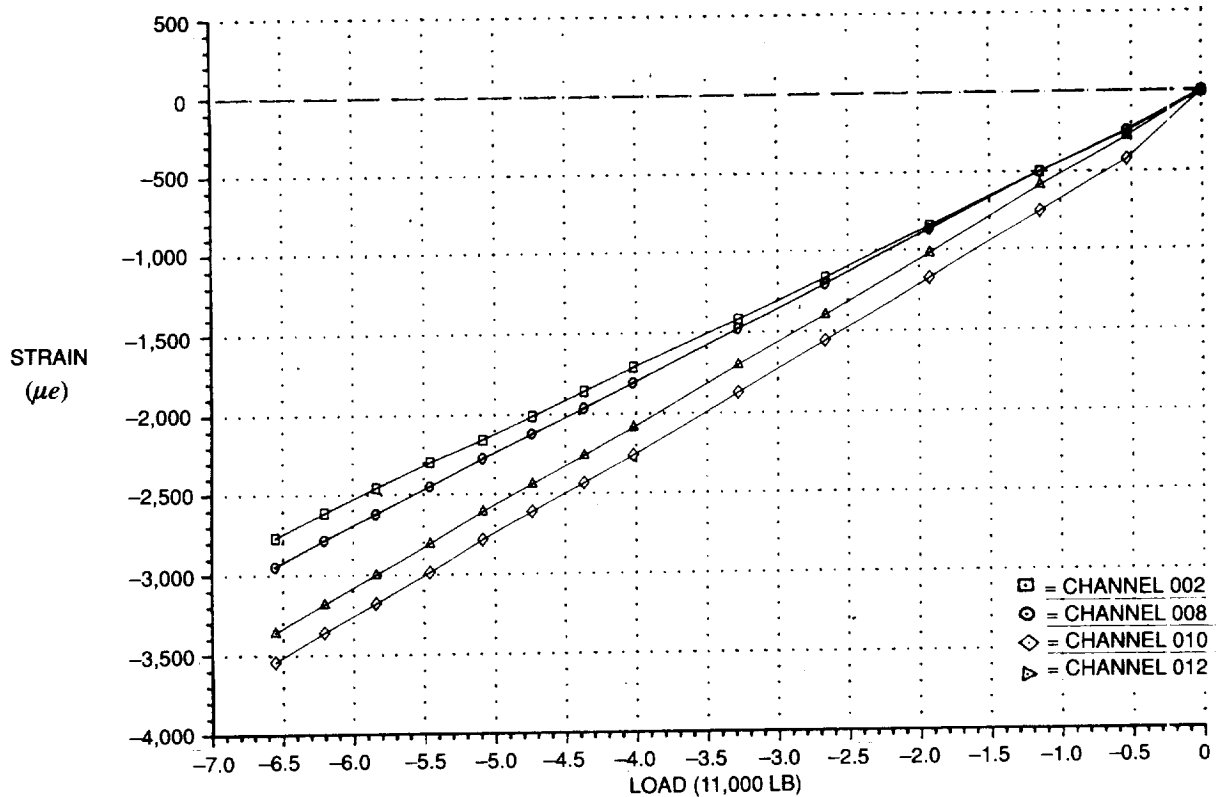
FIGURE 22. ROOM TEMPERATURE COMPRESSION TEST — COMPOSITE SIDE, LARGE SLIDING JOINT — STRAIN GAGE READING
