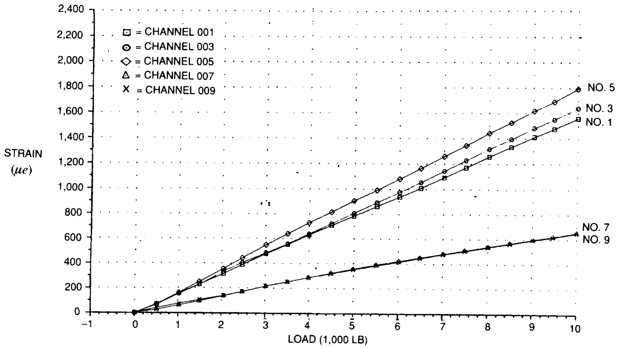
FIGURE 152. COMPOSITE FLANGE TENSION TEST AT ROOM TEMPERATURE — STRAIN GAGE READINGS
