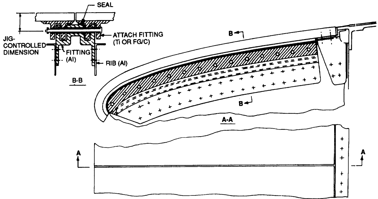
FIGURE 48. SLIDING CONCEPT
