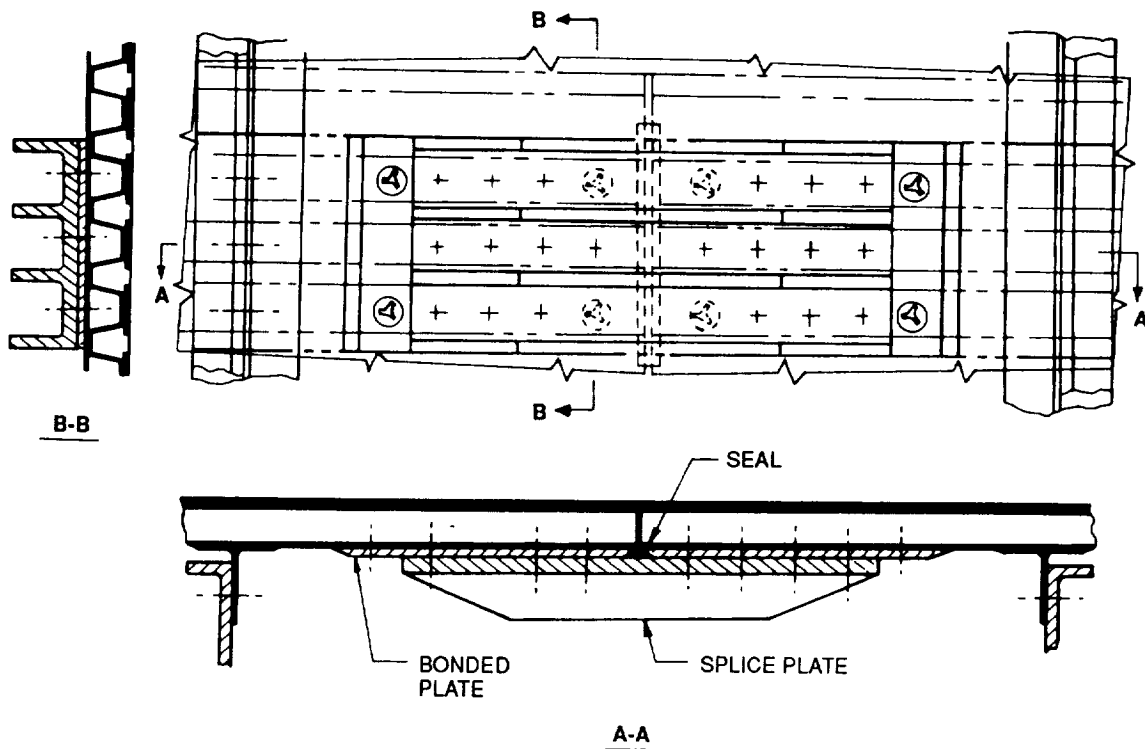
FIGURE 59. BEAM CONCEPT
