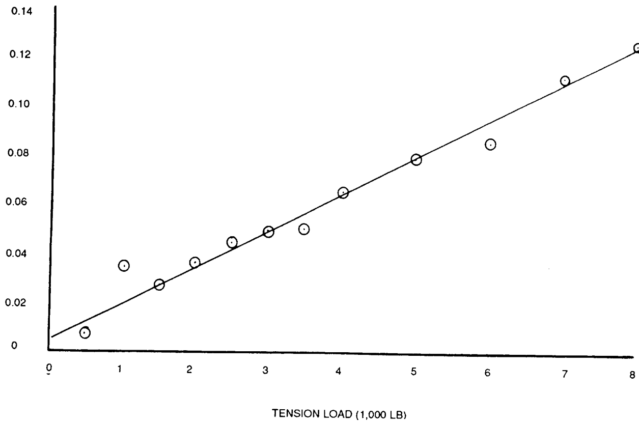
FIGURE 98. BOWING OF SLIDING JOINT IN TENSION
