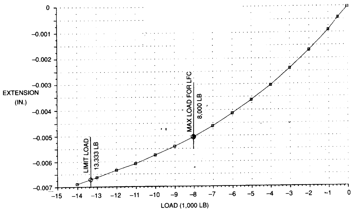
FIGURE 34. MODIFIED JOINT COMPRESSION LFC TEST AT -65^{\circ}\text{F} — EXTENSOMETER READINGS
