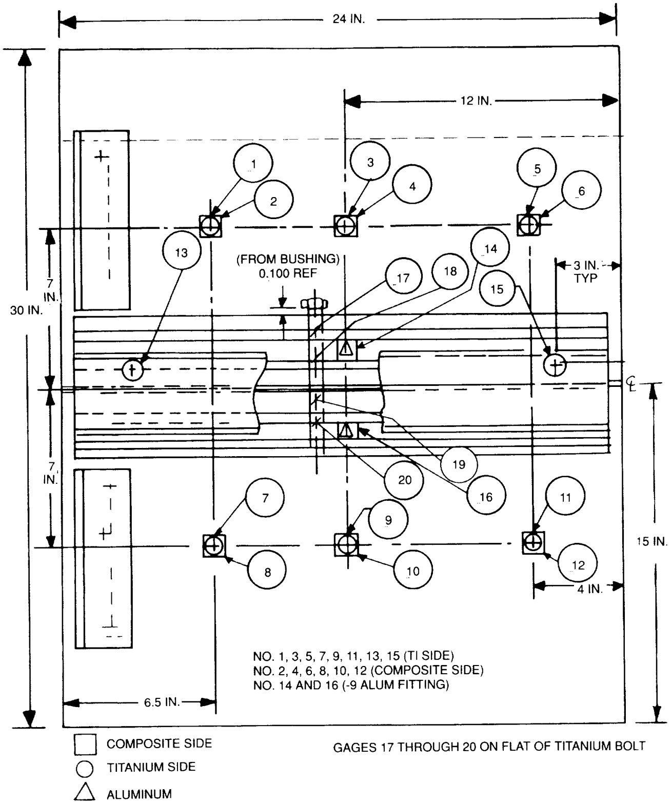
FIGURE 142. STRAIN GAGE PLACEMENT FOR TENSION TEST OF THE LARGE SLIDING-JOINT PANEL
