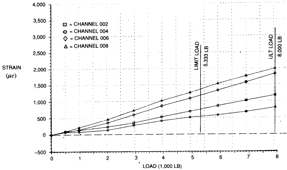
FIGURE 46. MODIFIED JOINT TENSION TEST AT -65^{\circ}\text{F} — STRAIN GAGE READINGS
