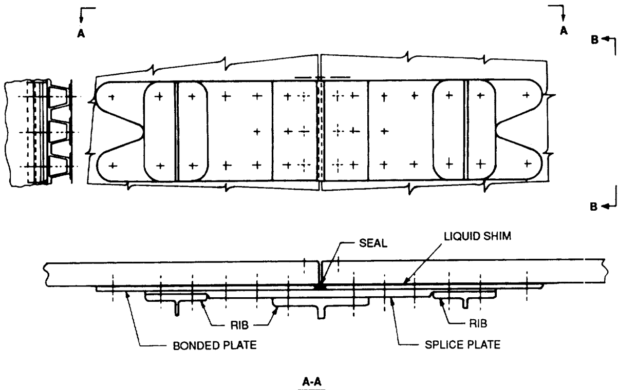
FIGURE 49. THREE-RIB CONCEPT
