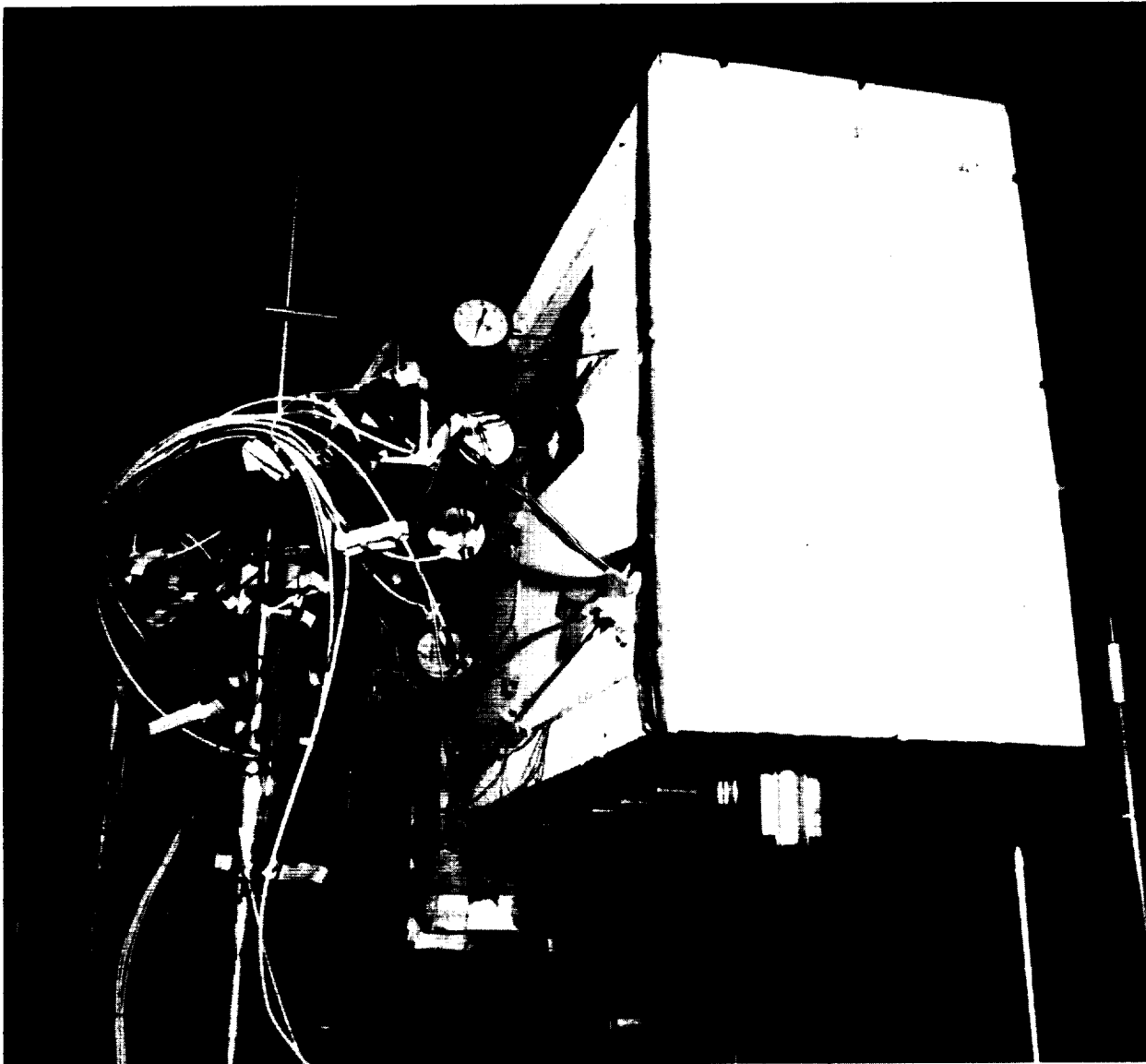
FIGURE 138. VIEW SHOWING DIAL GAGES PENETRATING THROUGH THE ENVIRONMENTAL BOX TO MEASURE THE PANEL DEFLECTIONS
