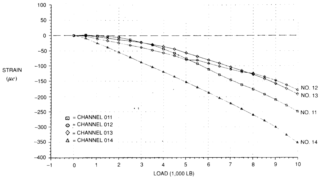
FIGURE 157. COMPOSITE FLANGE TENSION TEST AT -65°F — STRAIN GAGE READINGS
