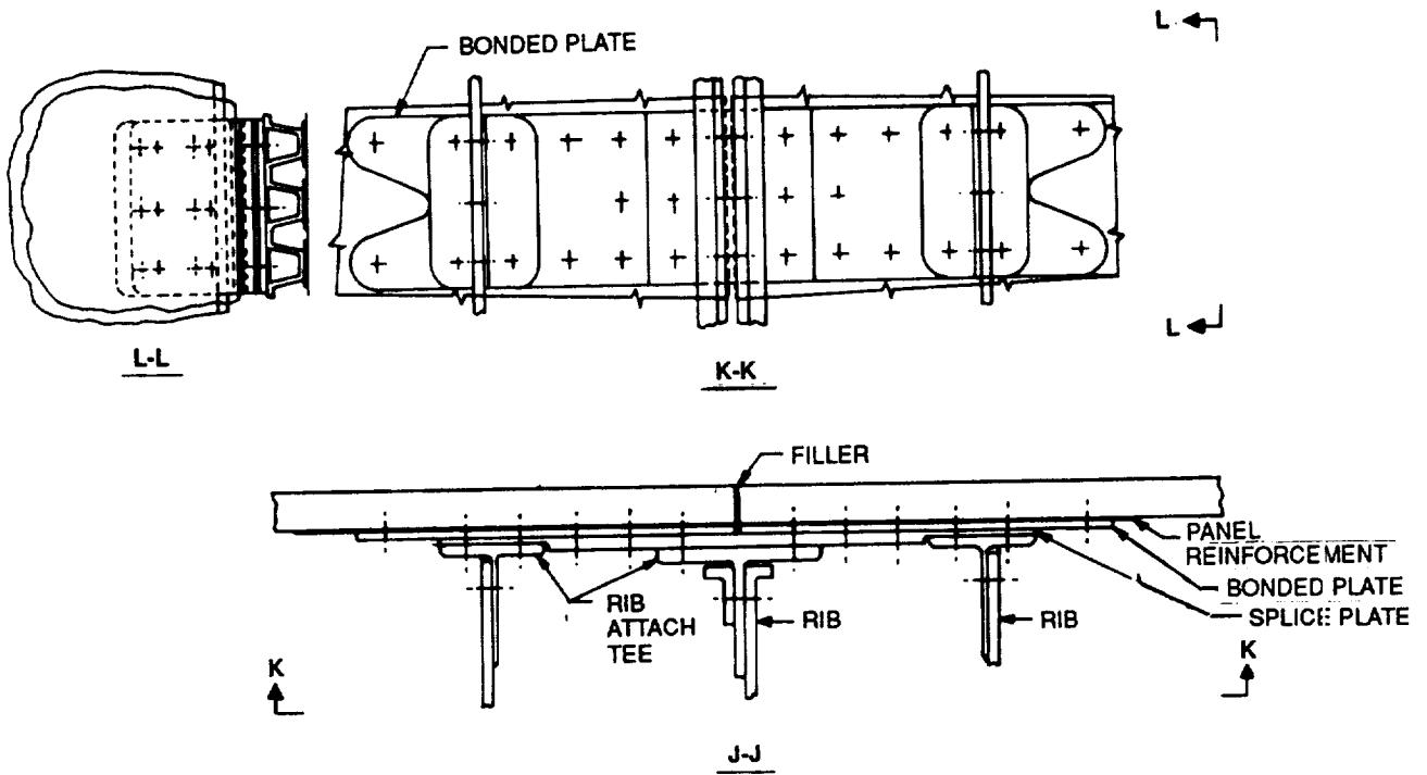
FIGURE 64. THREE-RIB CONCEPT
