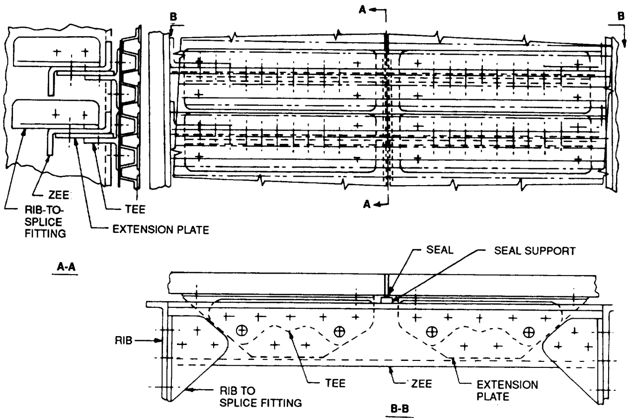
FIGURE 58. BLADE CONCEPT
