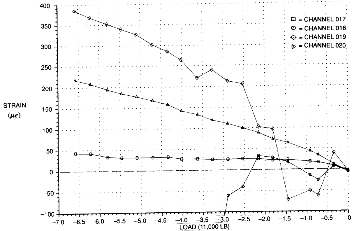
FIGURE 26. COLD COMPRESSION ( -65^{\circ}F ) — TITANIUM BOLT, LARGE SLIDING JOINT — STRAIN GAGE READING
