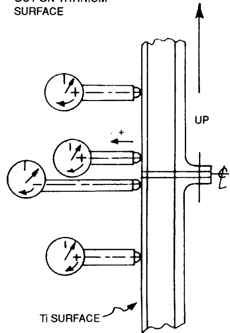
FIGURE 168. DIAL GAGE READINGS FOR MODIFIED JOINT PANEL IN COMPRESSION AT -65°F
