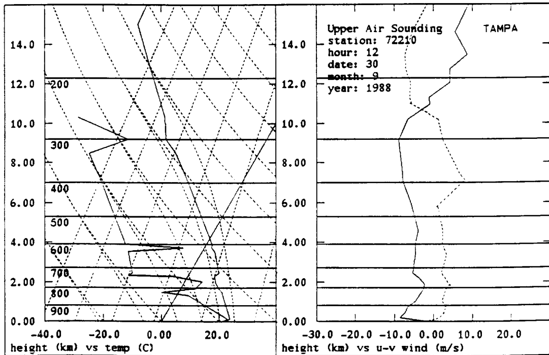
Figure 11: Skew T diagrams for the 12 Z West Palm Beach (A) and Tampa, Florida, (B) soundings on 30 September 1988. In the graph of horizontal air velocity vs. altitude, the east component, u , is the solid line and the north component, v , is the dashed line.
