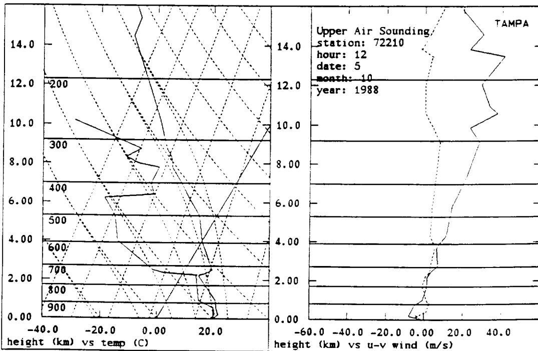
Figure 18: Skew T diagrams for the 13 Z West Palm Beach (A) and 12 Z Tampa, Florida, (B) soundings on 5 October 1988. In the graph of horizontal air velocity vs. altitude, the east component, u , is the solid line and the north component, v , is the dashed line.
