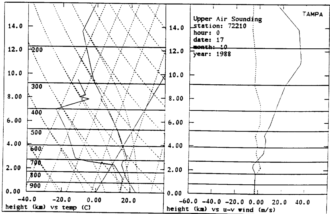
Figure 53: Skew T diagrams from the 0 Z West Palm Beach (A) and Tampa, Florida, (B) soundings on 17 October 1988. In the graph of horizontal air velocity vs. altitude, the east component, u , is the solid line and the north component, v , is the dashed line.
