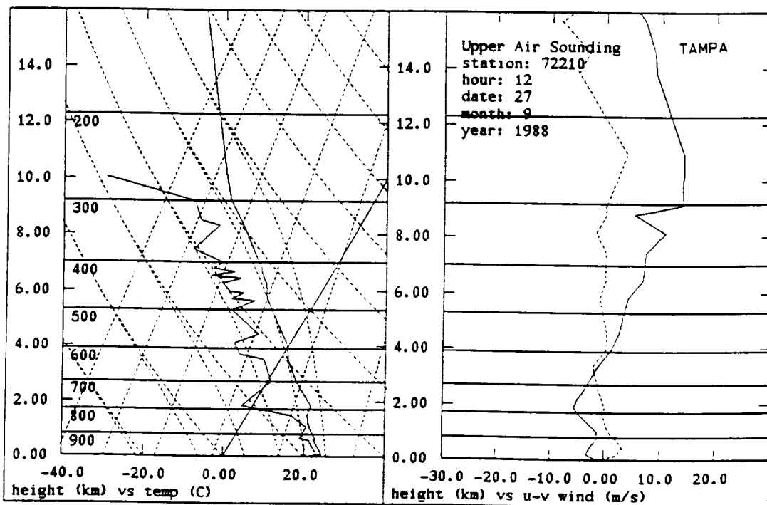
Figure 50: 27 September 1988 West Palm Beach and Tampa, Florida, skew T diagrams. In the graph of horizontal air velocity vs. altitude, the east component, u , is the solid line and the north component, v , is the dashed line.
