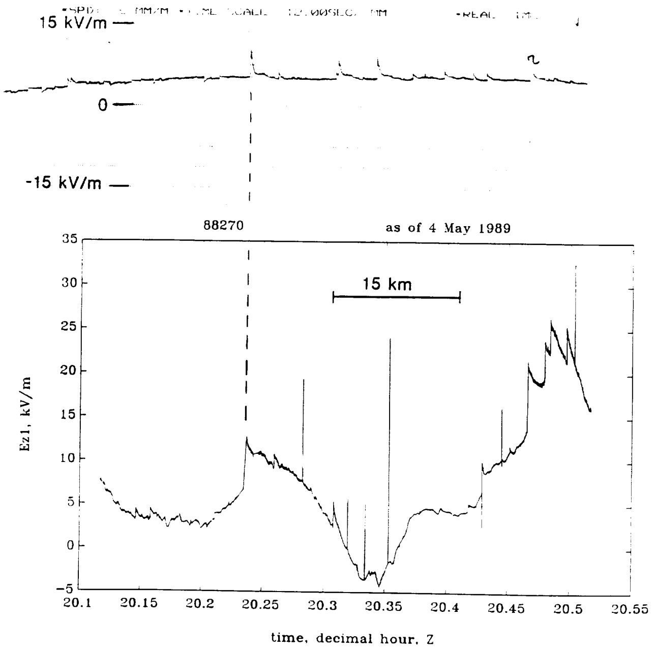
Figure 43: E_z vs. time at KSC field mill 10 (upper trace) and at SPTVAR (lower trace) on 26 September 1988 from 2006 to 2030 Z. The indicated \Delta E due to lightning at 2014:12 (dashed vertical line) is 6.0 kV/m at SPTVAR and 5.6 kV/m at mill 10.
