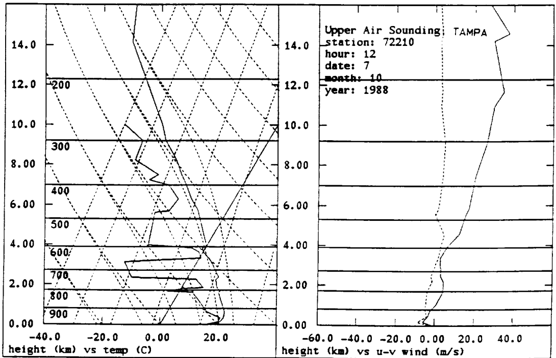
Figure 28: 12 Z skew T diagrams for West Palm Beach (A) and Tampa, Florida, (B) on 7 October 1988. In the graph of horizontal air velocity vs. altitude, the east component, u , is the solid line and the north component, v , is the dashed line.
