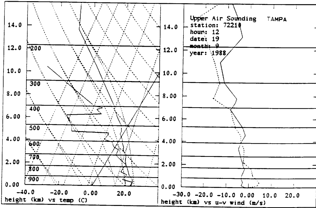
Figure 31: 12 Z West Palm Beach (A) and Tampa, Florida, (B) skew T diagrams for 19 September 1988. In the graph of horizontal air velocity vs. altitude, the east component, u, is the solid line and the north component, v, is the dashed line.
