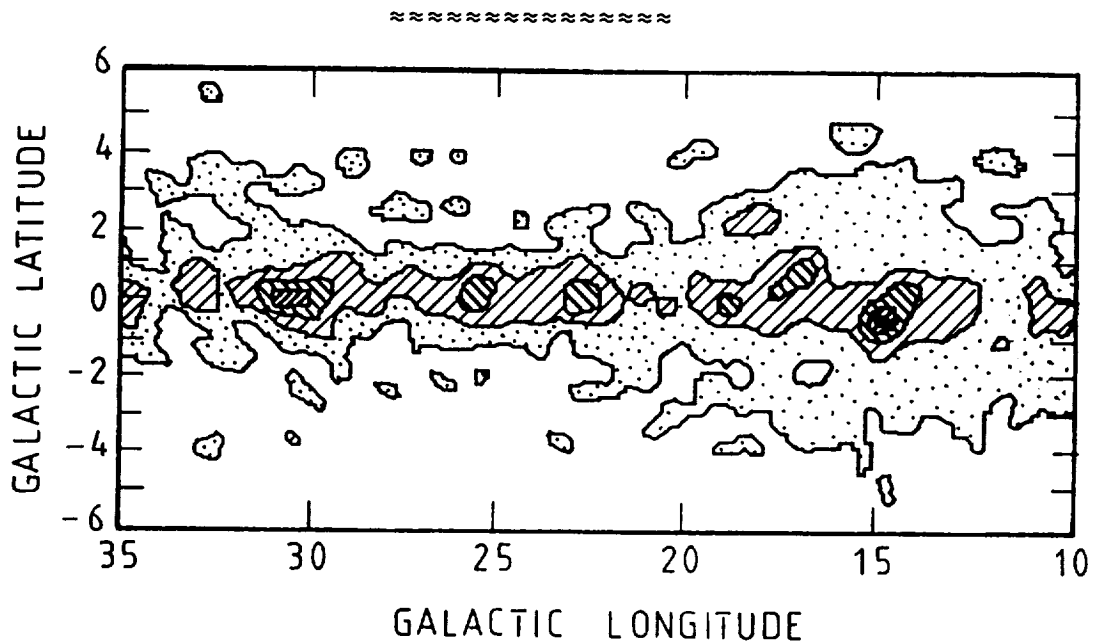
Figure 1 : Isophote map of the 3.3\mu\text{m} feature's intensity in galactic coordinates. The resolution is (\Delta l \times \Delta b) = (0.74^\circ \times 0.90^\circ) . The first level and the step are equal to 6 \cdot 10^{-8} \text{ W/m}^2/\text{sr} and the r.m.s. noise fluctuation is 1.2 \cdot 10^{-8} \text{ W/m}^2/\text{sr} .
