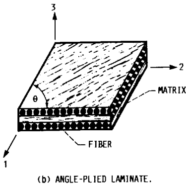
FIGURE 1. - TYPICAL COMPOSITE GEOMETRY.
