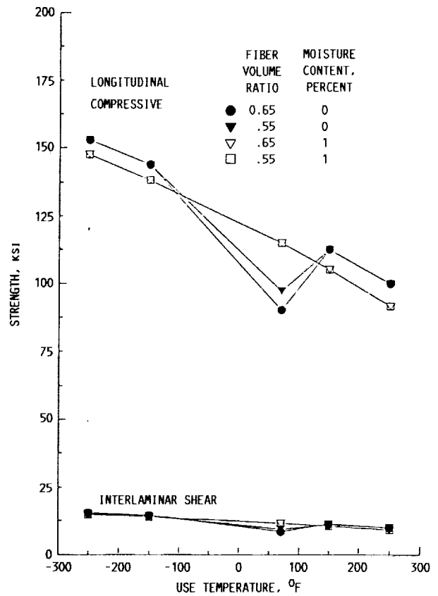
FIGURE 22. - STRENGTH OF THE COMPOSITE VERSUS THE USE TEMPERATURE AT DIFFERENT FIBER VOLUME RATIO AND MOISTURE CONTENT:
