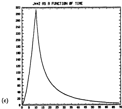
Fig. 5 — Global quantities versus time. (a) logarithm of kinetic energy ( 1/2 \langle |v|^2 \rangle ). (b) magnetic energy ( 1/2 \langle |B|^2 \rangle ). (c) mean square electric current ( 1/2 \langle |j|^2 \rangle ). (d) mean magnetic Lundquist number
