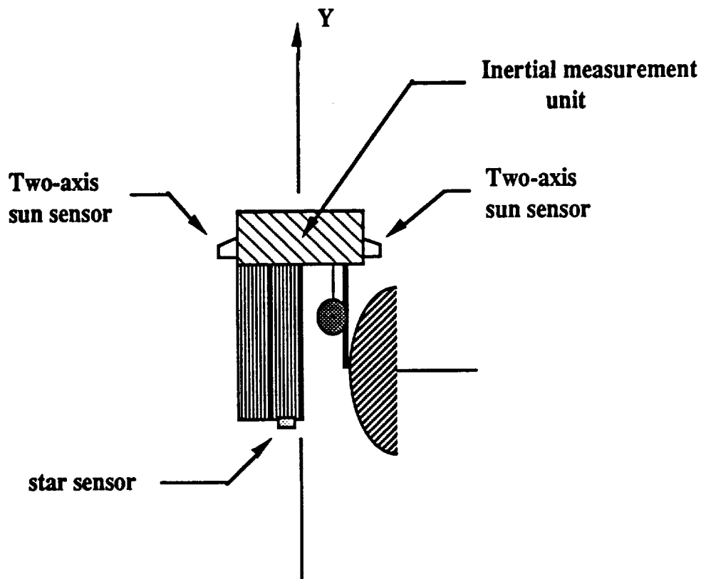
Figure 4 Sensor placement
