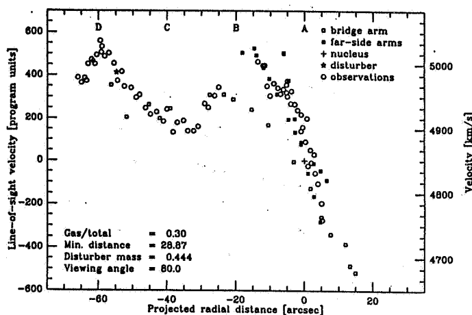
Fig. 4. The best-fit rotation curve with the observations.
