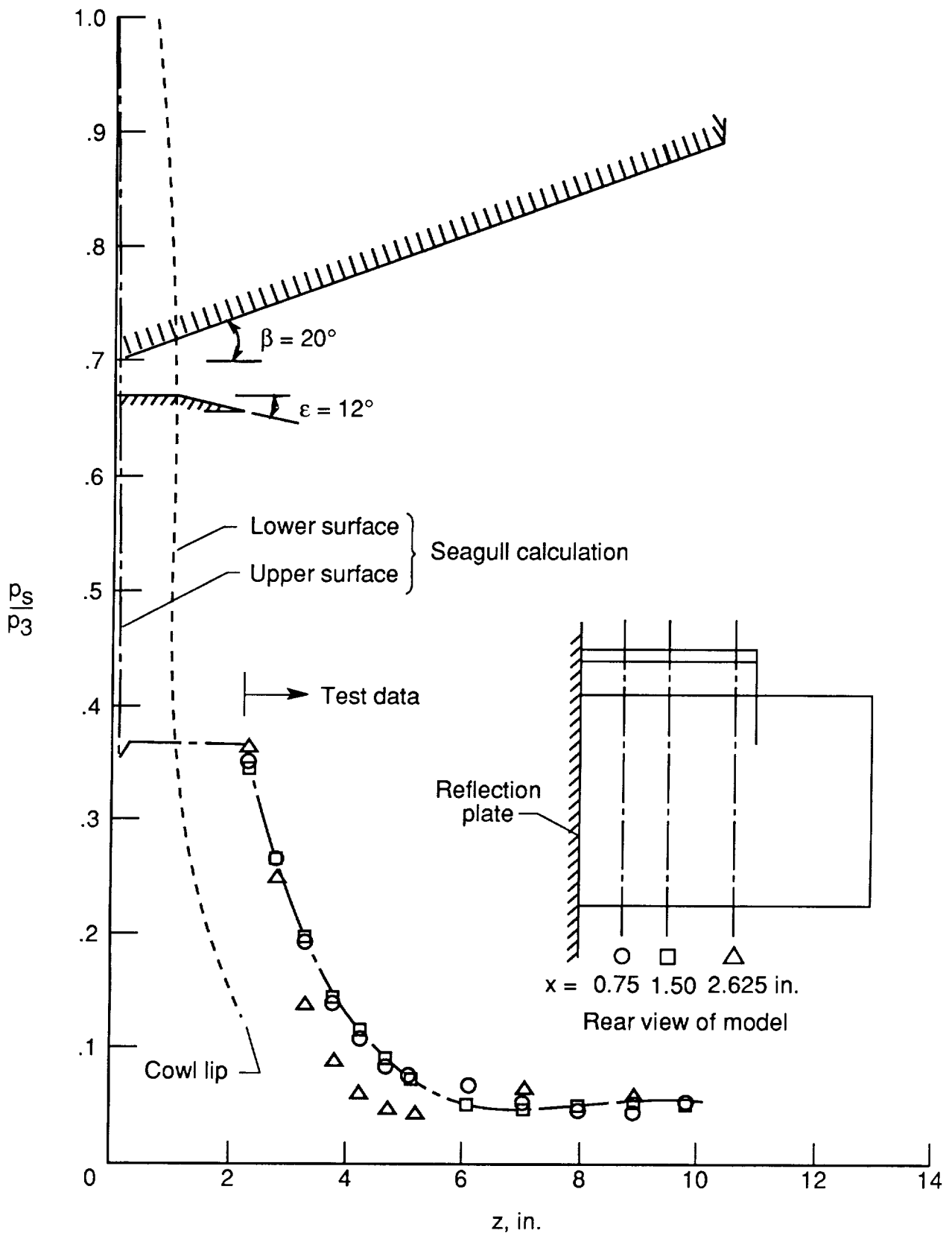
Figure 13. Pressure distributions from Seagull for complete nozzle and measured data for external surface of configuration V. p_3 = 4.731 psia; p_4/p_\infty = 2.655 .
