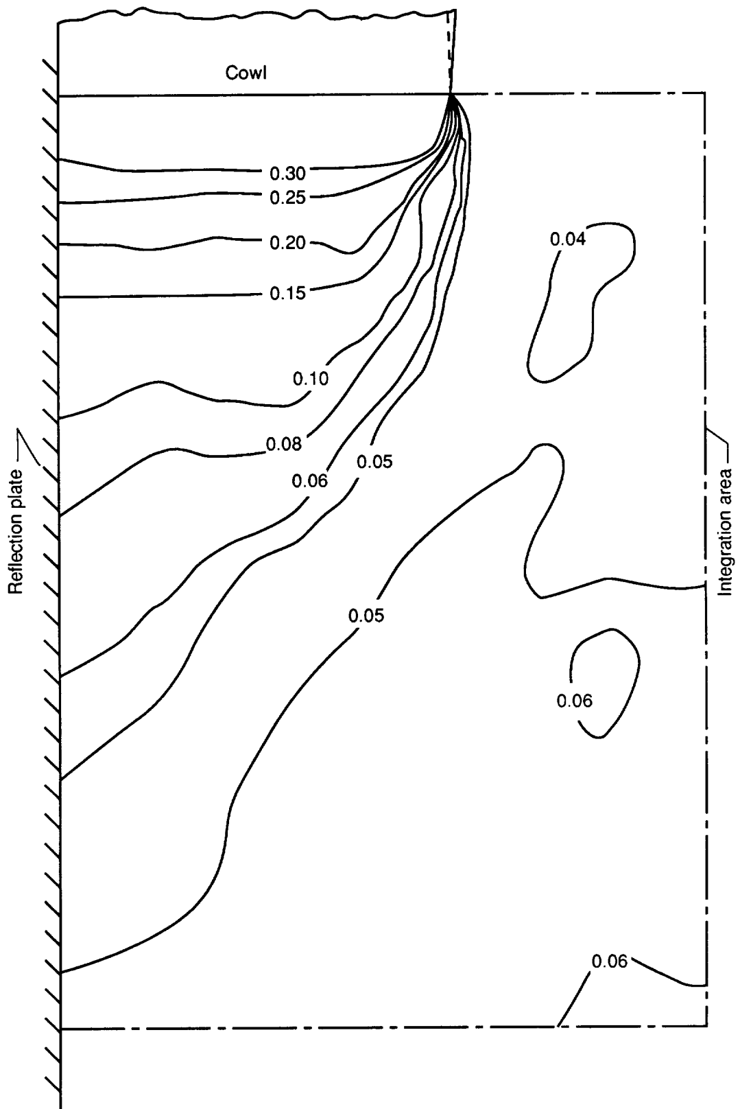
(c) Isobars of p_s/p_3 . Figure 8. Concluded.
