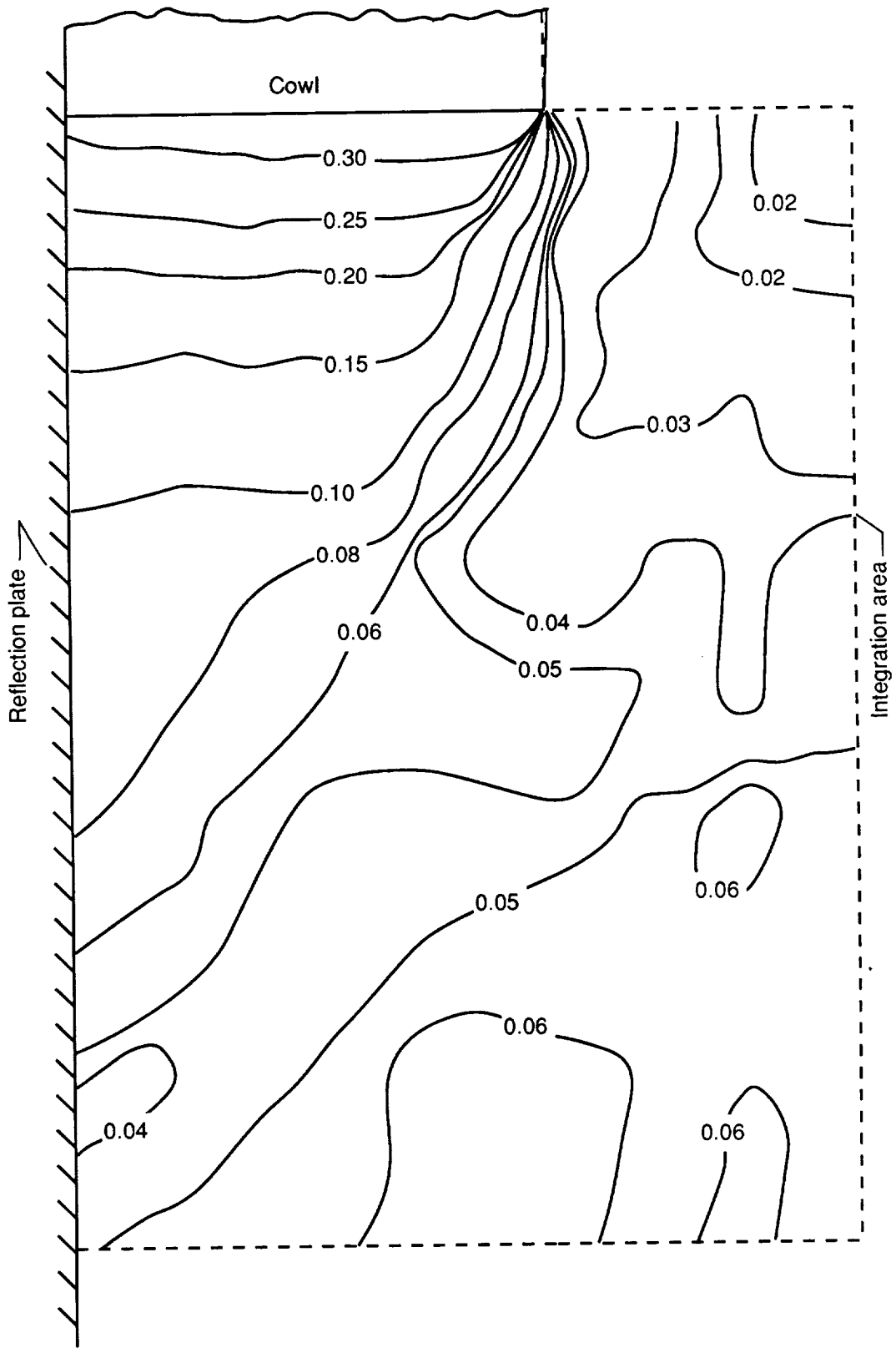
(c) Isobars of p_s/p_3 . Figure 10. Concluded.
