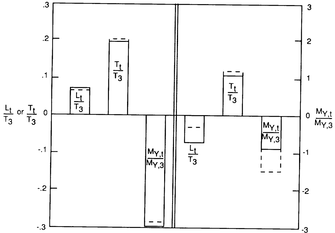
(b) Configurations V-A and V-E (with fence).
