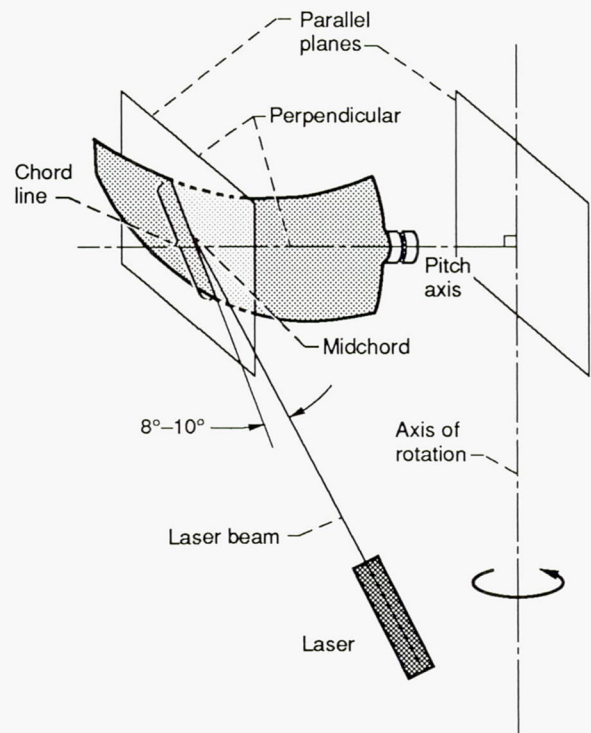
Figure 13.—Final orientation of laser beam with respect to blade chord.
