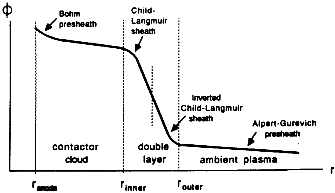
Figure 1 Schematic radial potential profile for collisionless unmagnetized double layer. The Bohm presheath is described in Ref. [12] and [13], and the Alpert-Gurevich presheath in Ref. [14].
