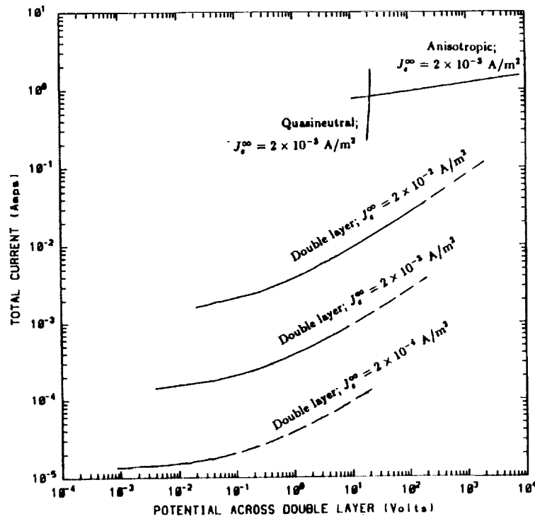
Figure 4 Total current vs. potential drop for the collisionless double layer model, the isotropic quasineutral model [4] and the anisotropic contactor model.
