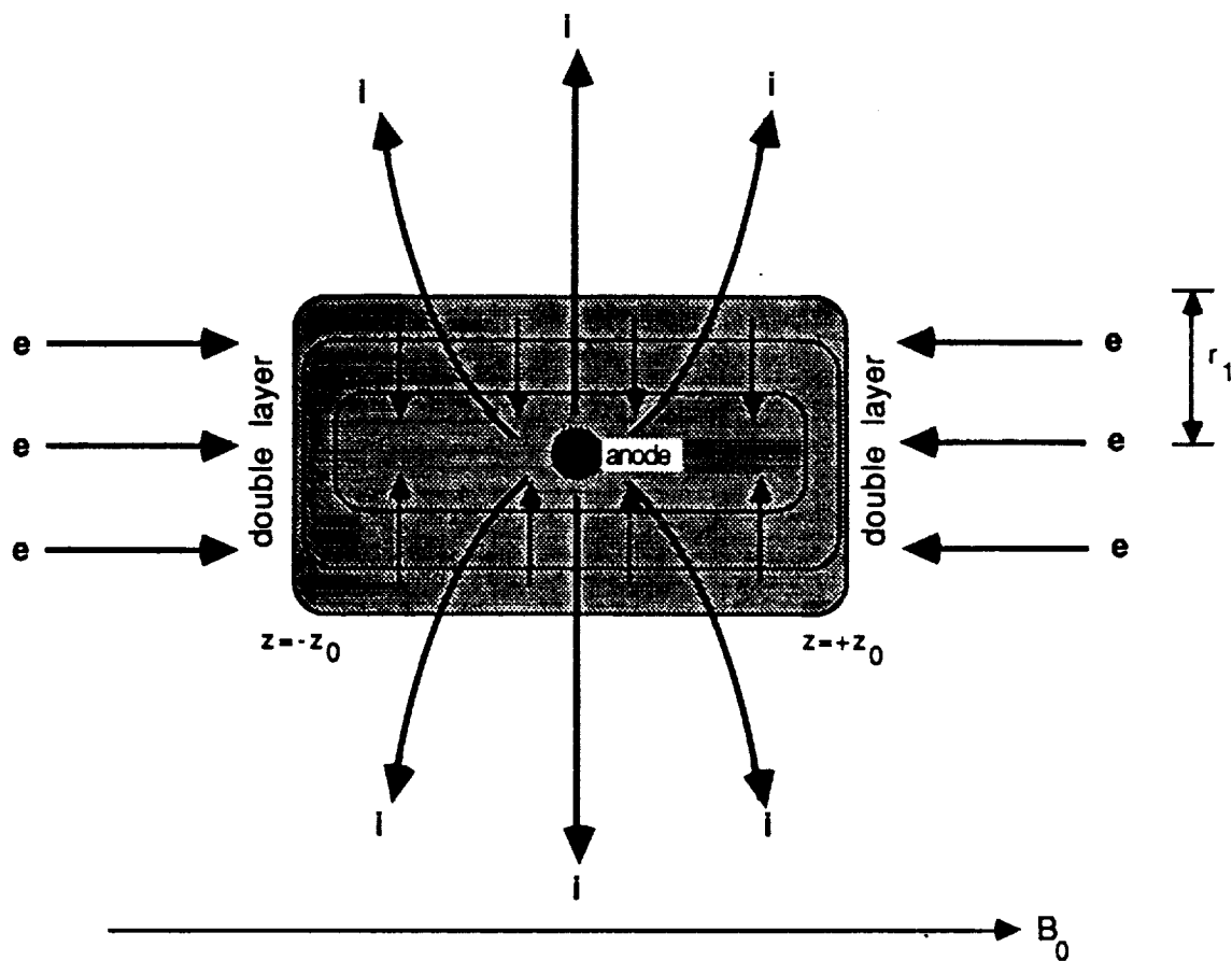
Figure 5 Schematic picture of the anisotropic contactor model, showing equipotential contours and the flow of ions and electrons.
