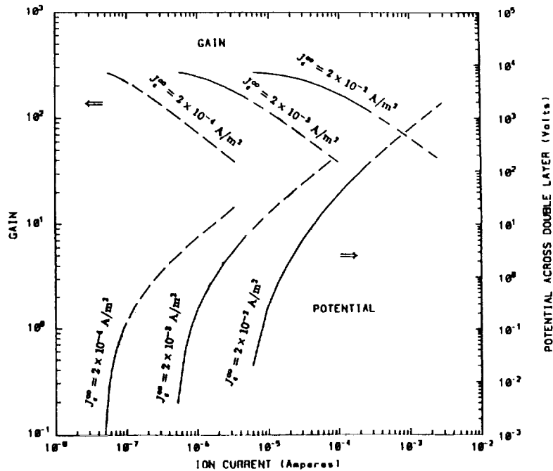
Figure 2 Gain and lower limit on potential drop, as functions of the emitted argon ion current and the electron saturation current, for collisionless double layer with space charge limited current, marginally satisfying the Parker-Murphy condition with a 10 cm anode radius, using Eq. (20) and Eq. (21), and Fig. 5 of Ref. [9].
