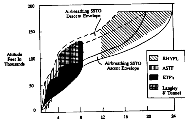
Fig. 2. Ground Test Facility Capability
