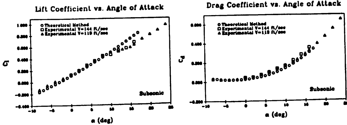
Fig. 11. Wind Tunnel Data
