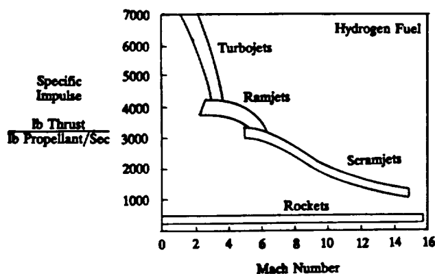
Fig. 1. Propulsion System Operating Regimes
