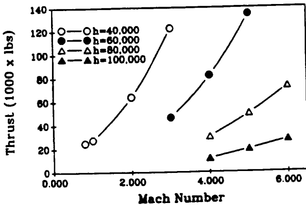
Fig. 7a. Turbofanramjet Performance
