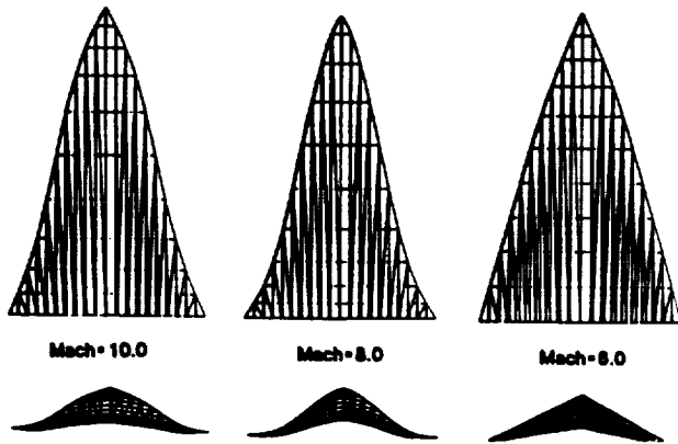
Fig. 9. Waverider Comparison
