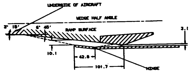
Fig. 8b. Scramjet Inlet M = 10.0
