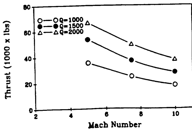
Fig. 7b. Scramjet Performance
