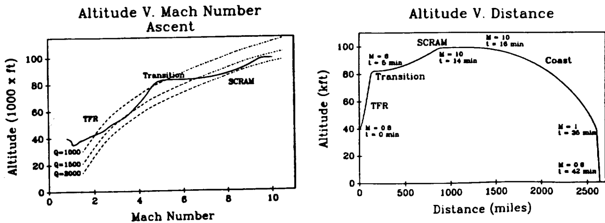
Fig. 13. Flight Profile
