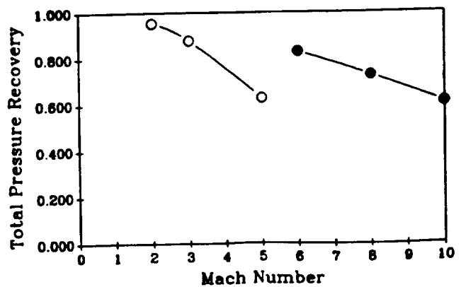
Fig. 8c. Inlet Pressure Recovery
