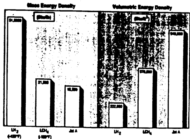
Fig. 6a. Fuel Comparison
