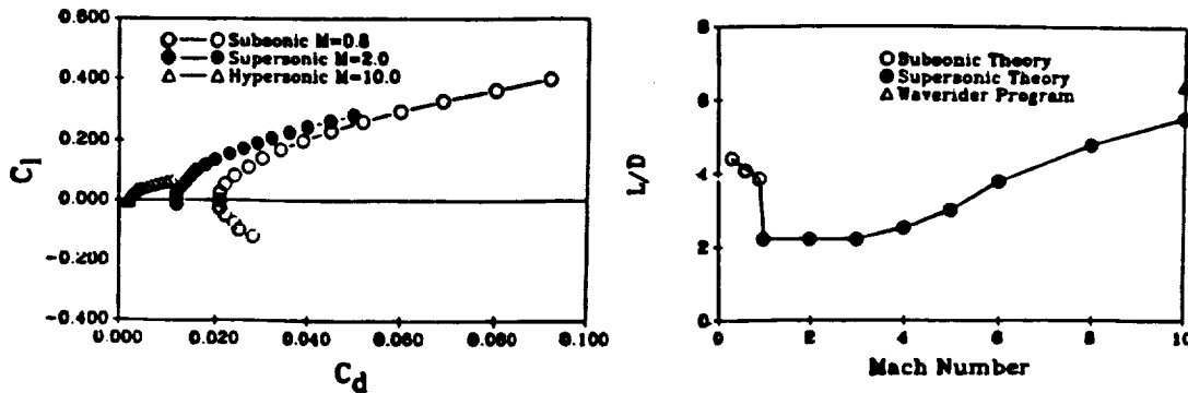
Fig. 10. Theoretical Aerodynamics
