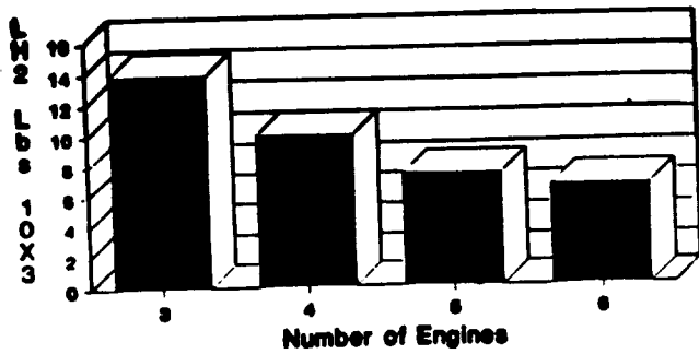
Fig. 6b. Number of Engines vs. Fuel Weight for Scramjet Operation
