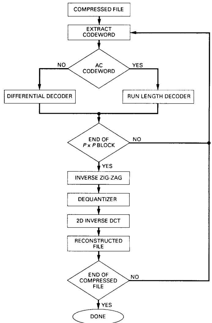
Fig. 3. Baseline decompressor for Huffman coding.
