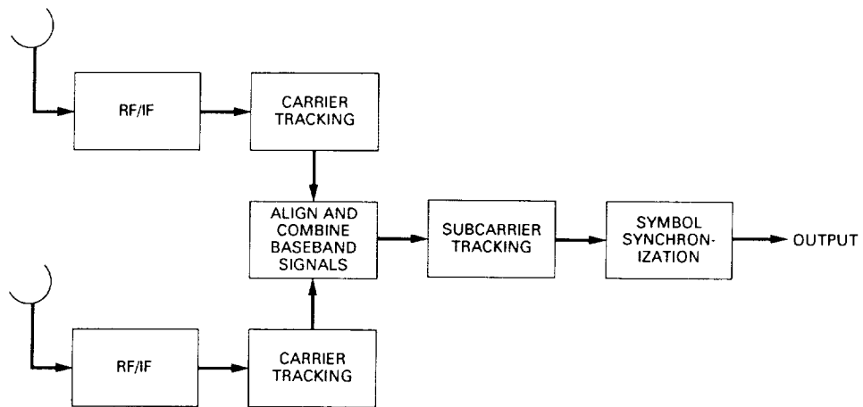
Fig. 6. Baseband combining.
