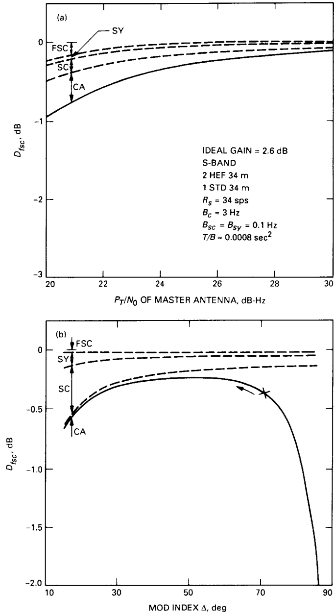
Fig. 11. The D_{fsc} versus: (a) P_T/N_0 for \Delta = 65.9 deg, and (b) \Delta for P_T/N_0 = 25 dB-Hz.
