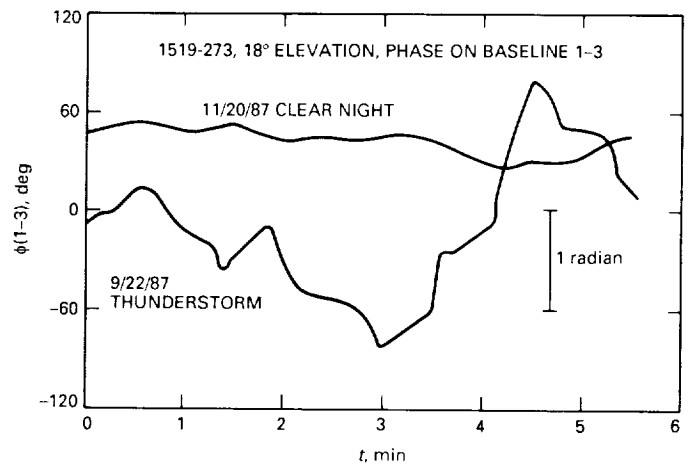
Fig. 16. Very Large Array thunderstorm data at 8.4 GHz.
