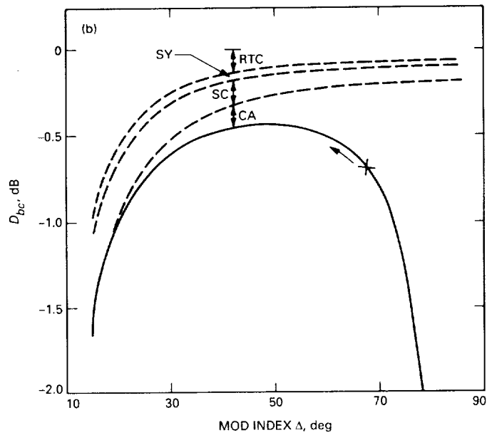
Fig. 7. The D_{bc} versus: (a) P_T/N_0 for \Delta = 65.9 deg, and (b) \Delta for P_T/N_0 = 25 dB-Hz.
