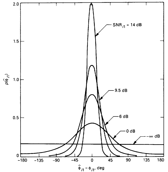
Fig. 10. The probability distribution of measured phase as a function of \hat{\phi} - \phi for a number of signal-to-noise ratios.
