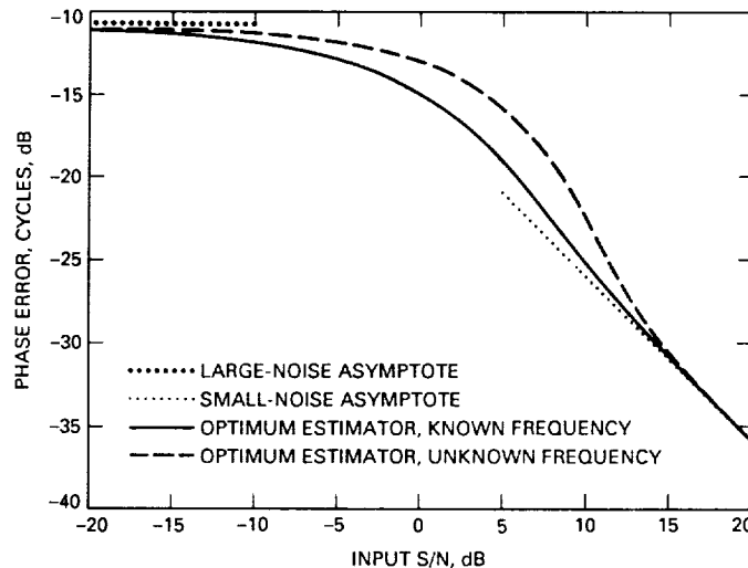
Fig. 3. Phase-error performance of the optimum estimator for the case of unknown constant frequency. The small-noise asymptote comes from Eq. (96) of [2].
