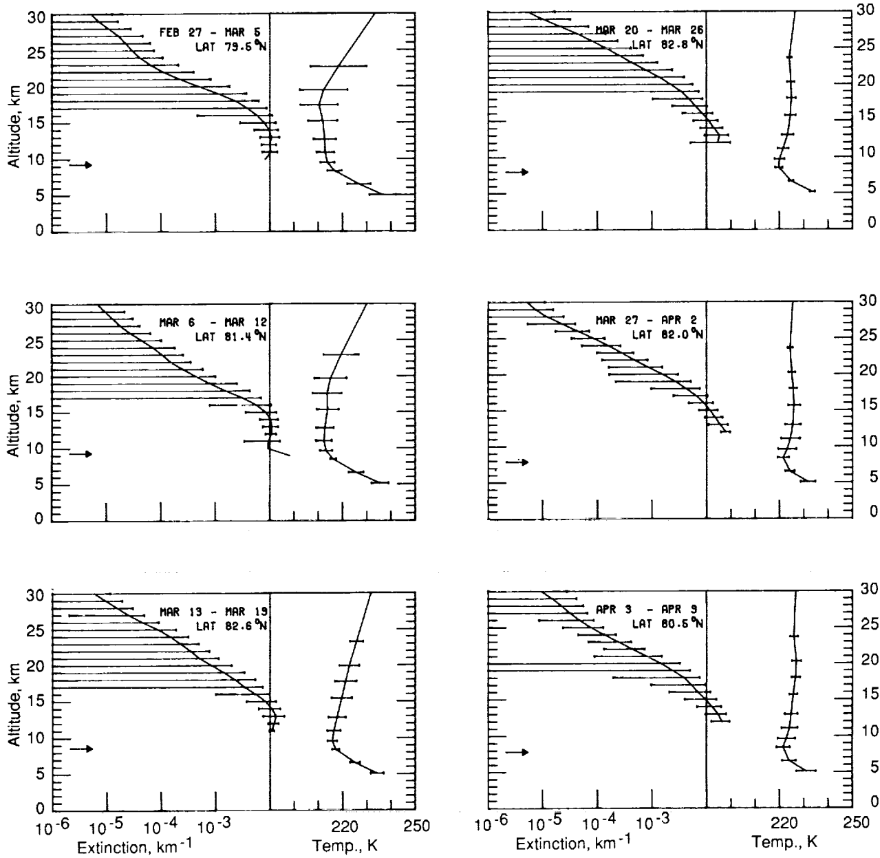
Figure 5. Arctic extinction and temperature profiles for February 27 to April 9, 1983.
