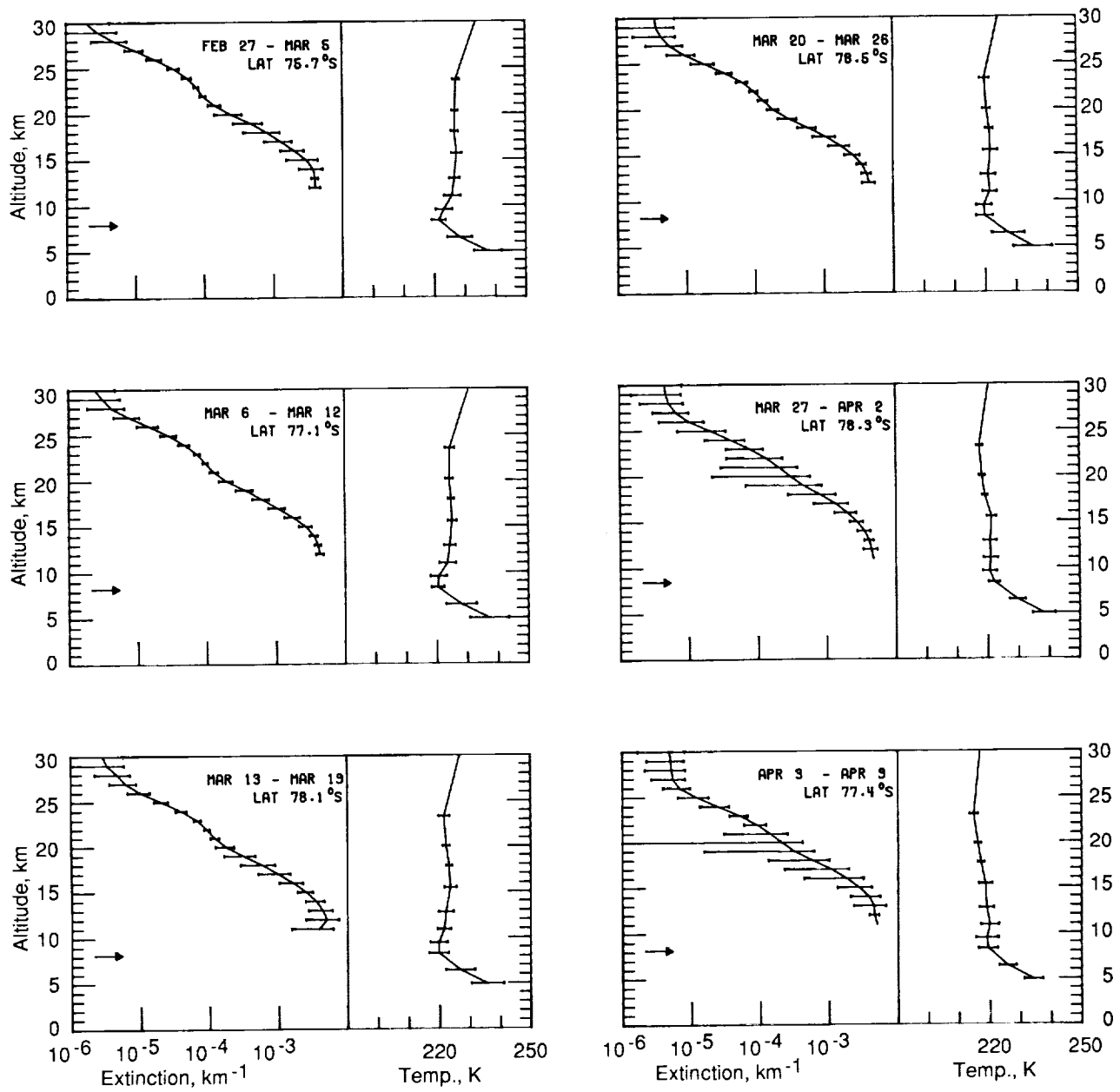
Figure 10. Antarctic extinction and temperature profiles for February 27 to April 9, 1983.
