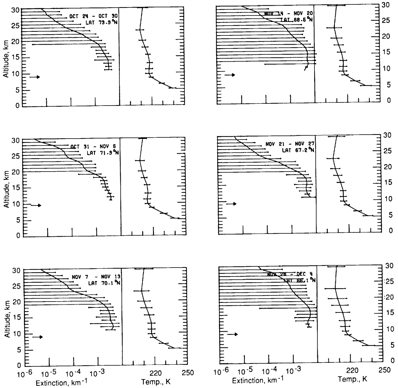
Figure 2. Arctic extinction and temperature profiles for October 24 to December 4, 1982.
