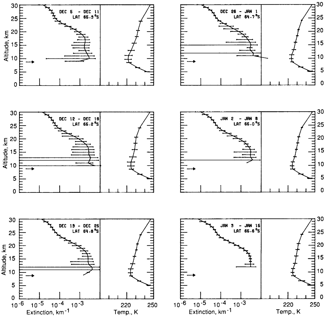
Figure 8. Antarctic extinction and temperature profiles for December 5, 1982, to January 15, 1983.
