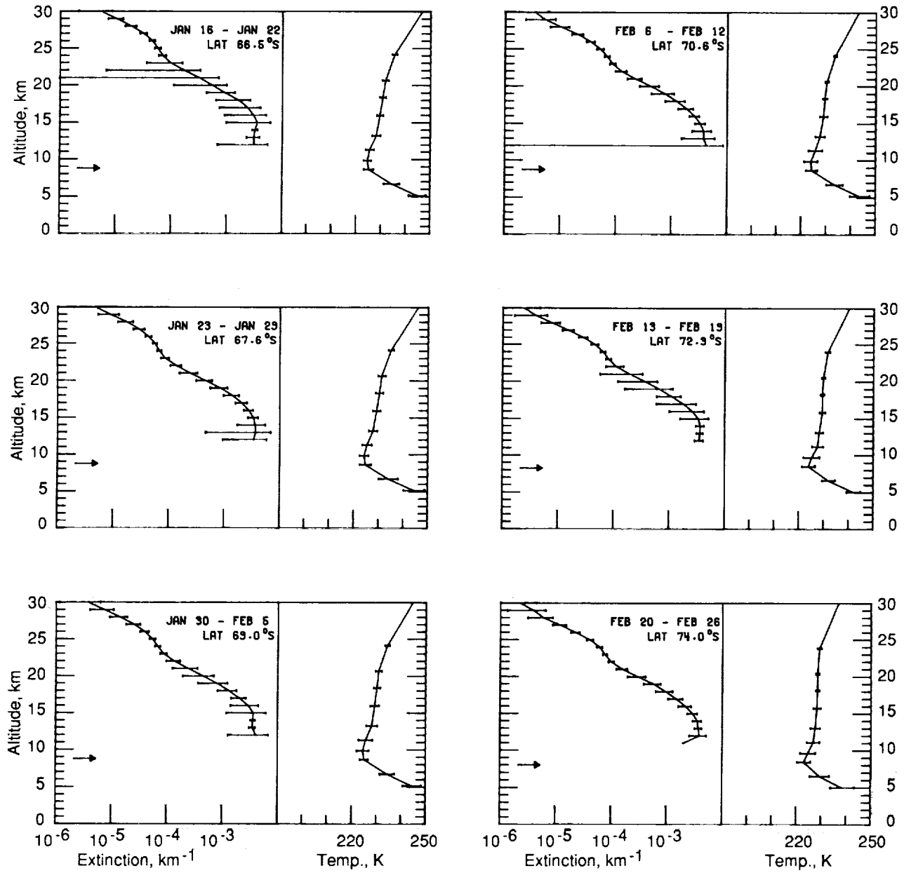
Figure 9. Antarctic extinction and temperature profiles for January 16 to February 26, 1983.
