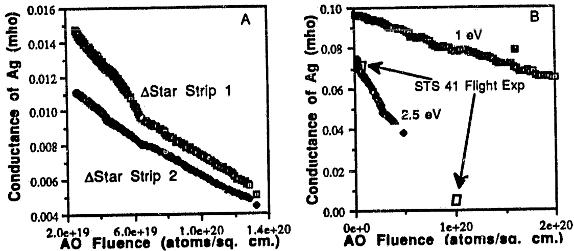
Figure 3. Panel A shows Delta Star SME flight results using 1 μm thick BN films over 250Å Ag film on rough alumina substrates. Panel B shows STS 41 flight and laboratory results for 750Å thick BN films on smooth sapphire substrates.
