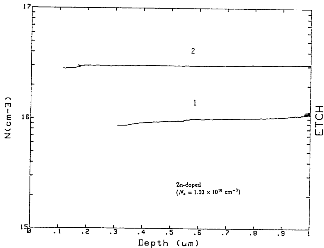
Figure 2. ECV acceptor concentration profiles before (curves 1) and after (curves 2) 3 hours heat treatment at 660°C of clean Cd- and Zn-doped InP substrates.
