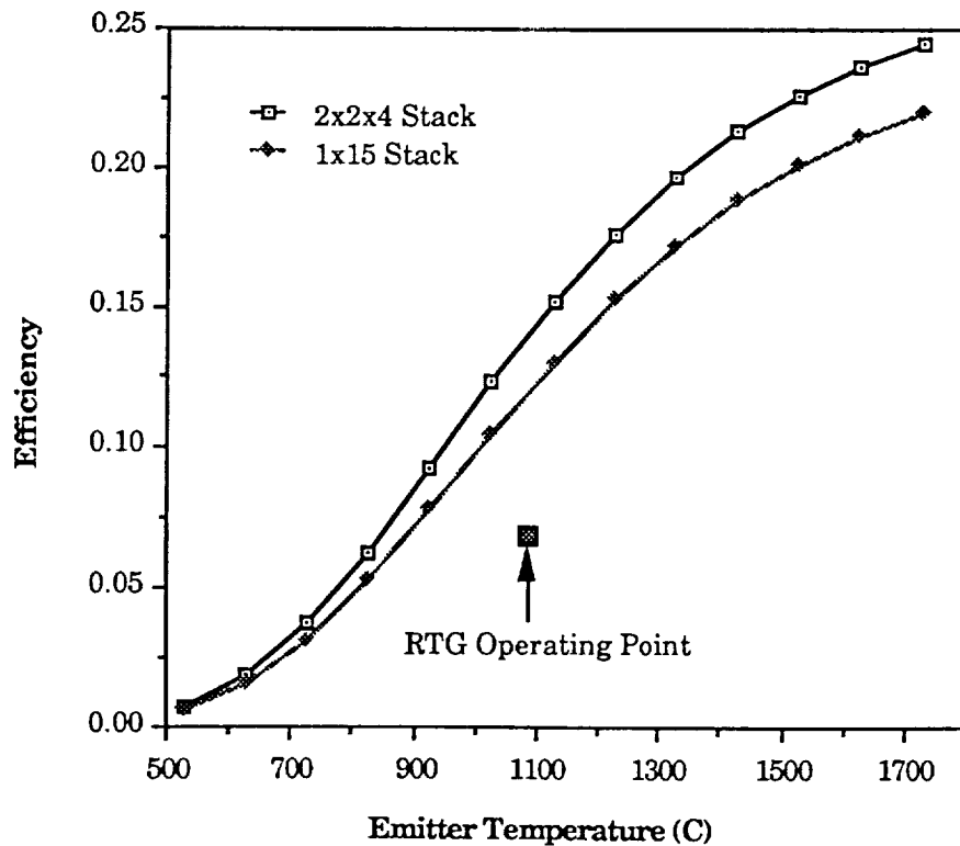
Figure 6: Efficiency of system which utilizes the GPHS versus temperature.
