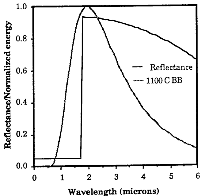
Figure 2: Predicted reflectance of GaSb cell with reflective rear contact. The emission spectrum of a 1100 C blackbody is included for reference.
