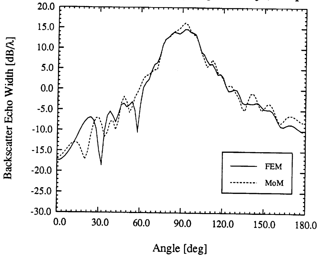
Case 2: Coated trailing edge, ( \epsilon=2-j1 ), H-pol
