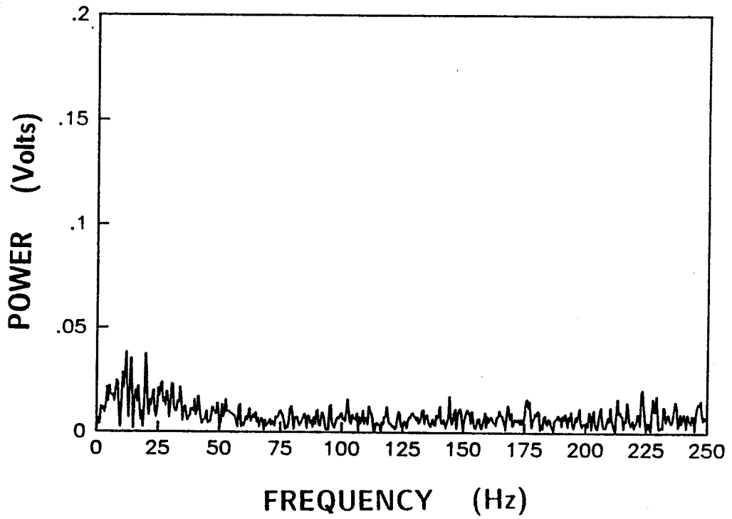
49d. U_{\infty} = 13.7 m/s, M_f = 144 Hz, \Delta P = 2.16 torr (256 Pa.)
