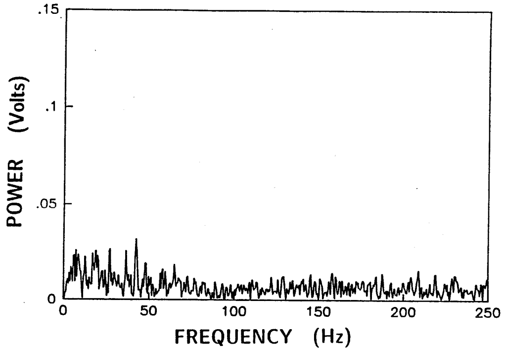
49c. U_{\infty} = 13.7 m/s, M_f = 211 Hz, \Delta P = 1.32 torr (175 Pa.)
