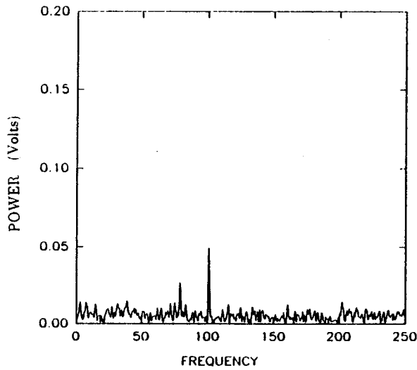
38g. U_\infty = 6.2 m/s, M_f = 81 Hz, \Delta P = .45 torr (59 Pa.), y = -17 mm.
