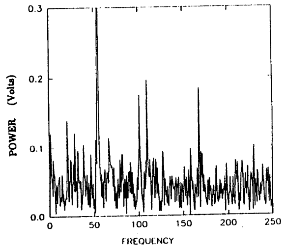
U_{\infty} = 32.0 \text{ m/s}, M_f = 54 \text{ Hz}, \Delta P = 7.94 \text{ torr (1058 Pa)}
