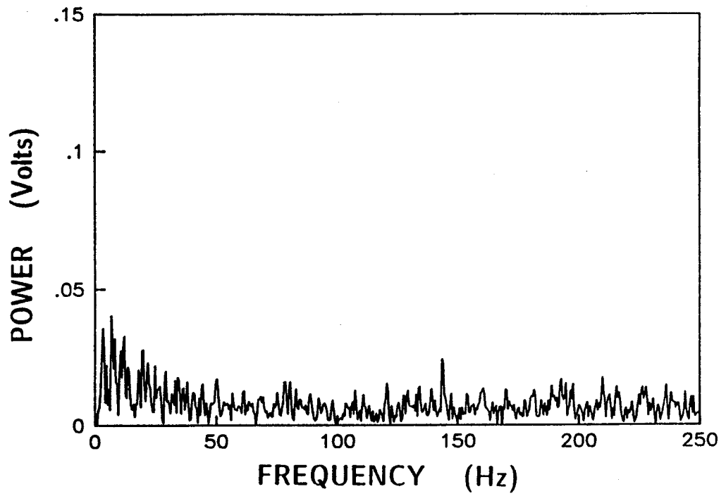
49e. U_{\infty} = 13.7 m/s, M_f = 143 Hz, \Delta P = 1.3 torr (169 Pa.)
