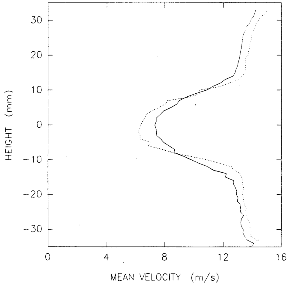
Figure 40. Mean velocity profiles, 38 mm behind the perturbation generator, U_{\infty} = 14 m/s. The dashed line is for M_f = 72 Hz, \Delta P = 2.82 torr (375 Pa), and the solid line is without perturbation.
