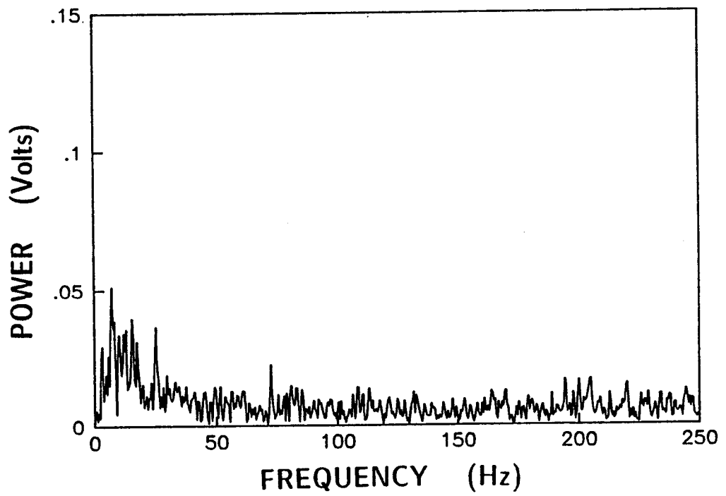
49f. U_{\infty} = 13.7 m/s, M_f = 72 Hz, \Delta P = 1.4 torr (182 Pa.)
