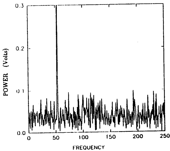
U_{\infty} = 25.5 \text{ m/s}, M_f = 55 \text{ Hz}, \Delta P = 5.87 \text{ torr (755 Pa)}
