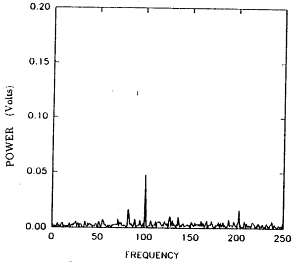
38a. U_{\infty} = 6.2 m/s, M_f = 84 Hz, \Delta P = .5 torr (66 Pa), y = +20 mm.
