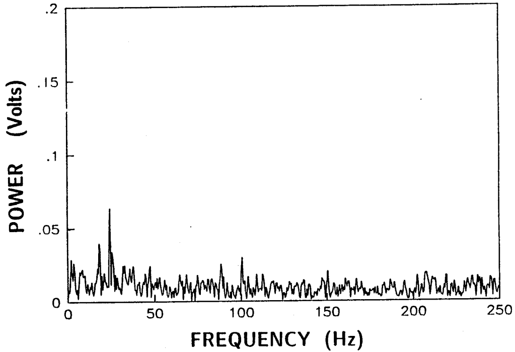
60h. Counter-rotating, U_{\infty} = 42 m/s, M_f = 164 Hz, \Delta P = 400 Pa
