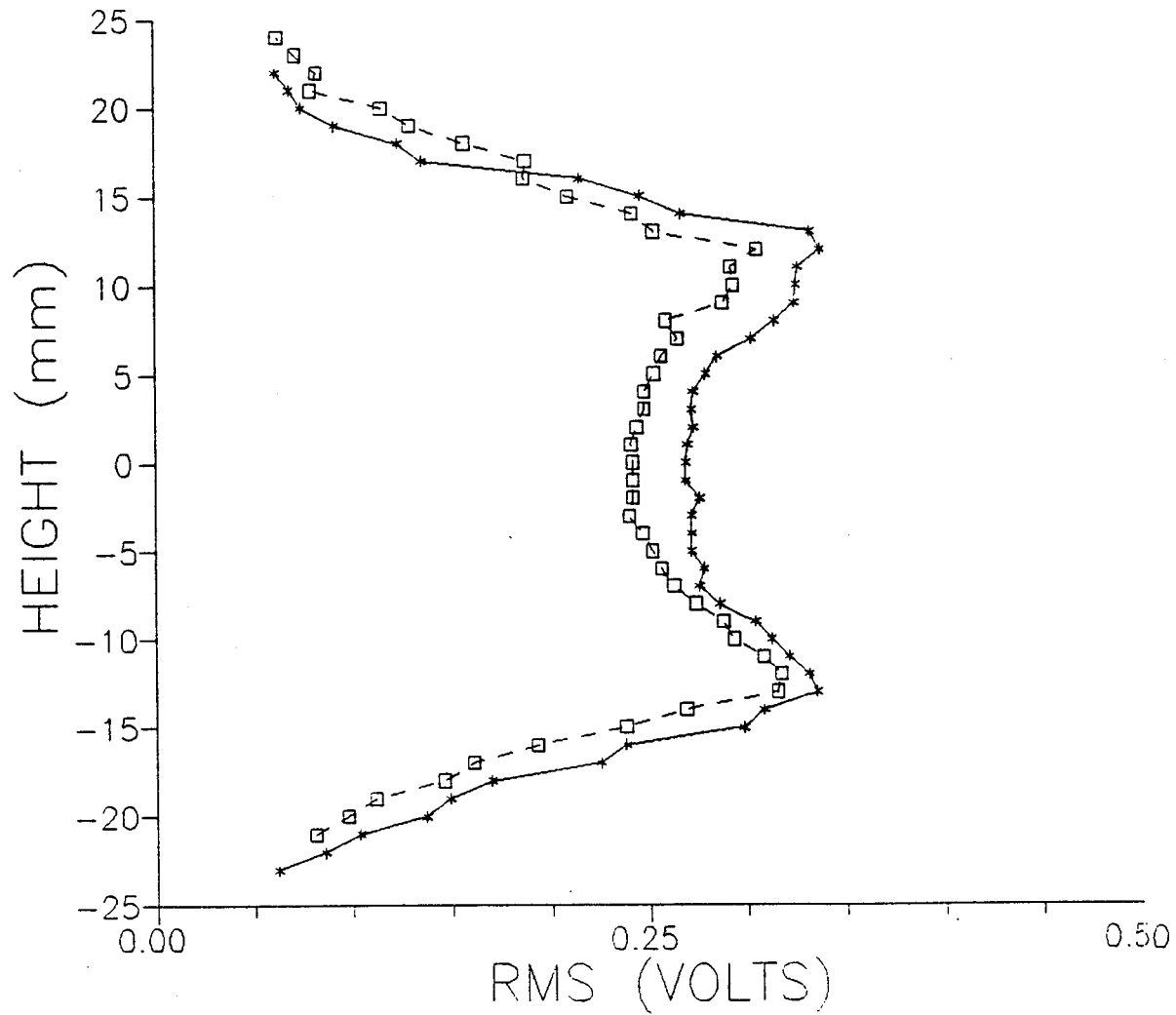
Figure 42. RMS profile of the wake, 38 mm behind the perturbation generator, U_{\infty} = 6 m/s. The dashed line is for M_f = 67.4 Hz, \Delta P = .316 torr (42 Pa), and the solid line is without perturbation.
