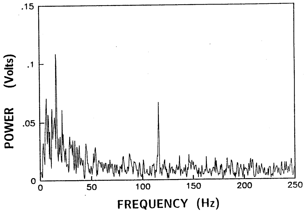
53d. U_{\infty} = 20.7 m/s, M_f = 116 Hz (co-rotating), \Delta P = 206 Pa
