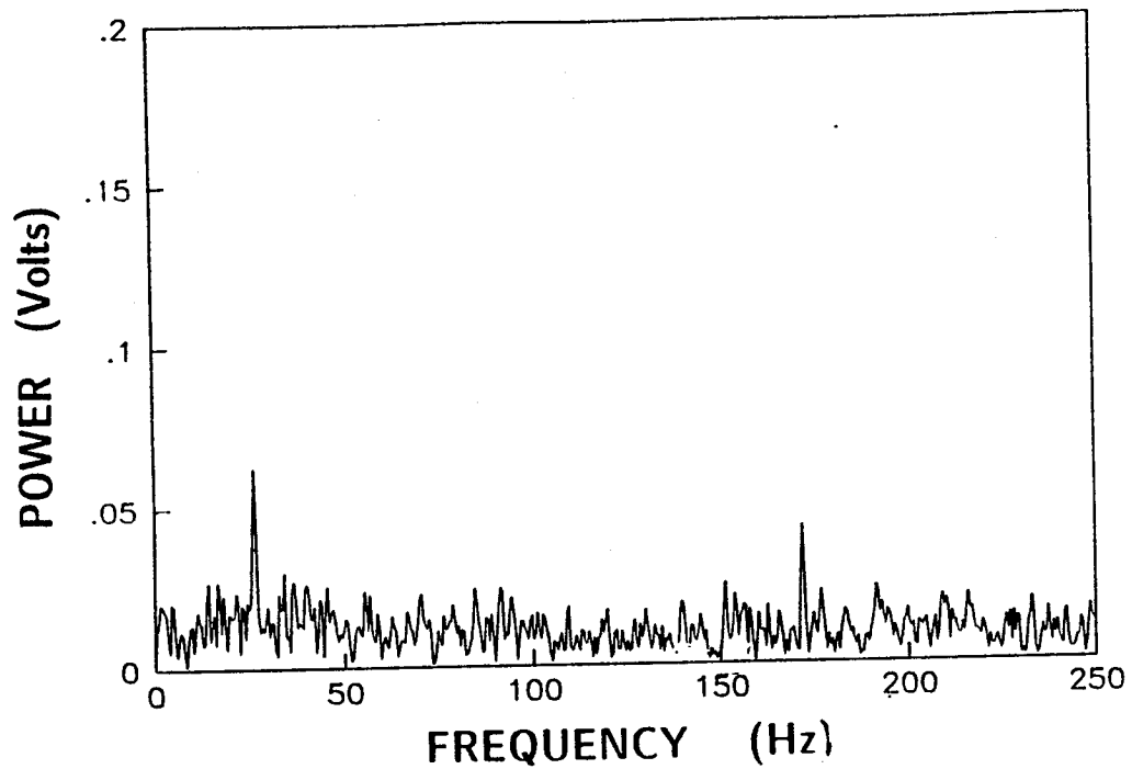
60g. Co-rotating, U_{\infty} = 42 m/s, M_f = 171 Hz, \Delta P = 430 Pa.
