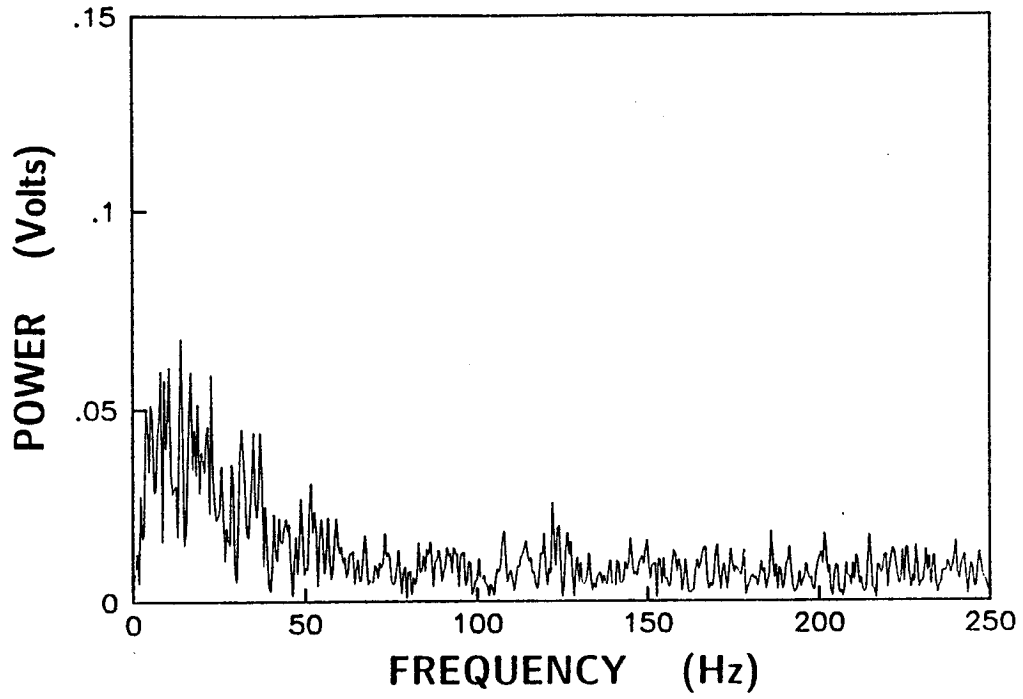
53c. U_{\infty} = 20.7 m/s, M_f = 122 Hz, (counter-rotating), \Delta P = 202 Pa
