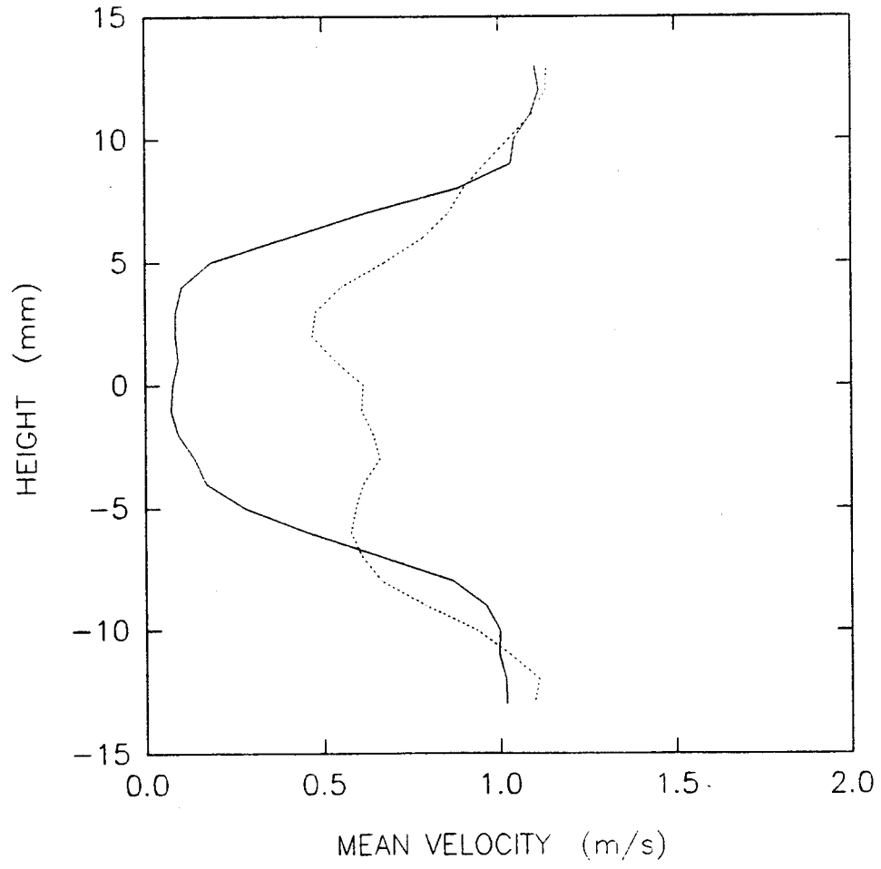
Figure 41. Mean velocity profiles, 38 mm behind the perturbation generator, U_{\infty} = 1 m/s. The dashed line is for M_f = 74 Hz, \Delta P = .33 torr (50 Pa), and the solid line is without perturbation.
