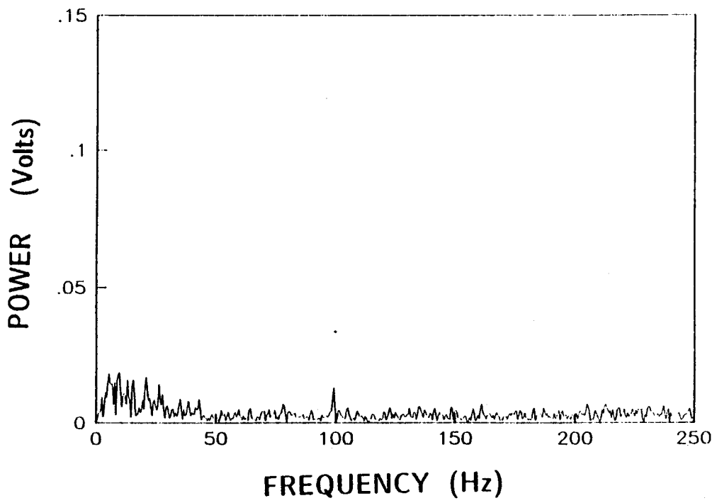
58d. X = 4.27 m, U_{\infty} = 13.7 m/s, M_F = 98.6 Hz (counter rotating), \Delta P = 178 Pa.
