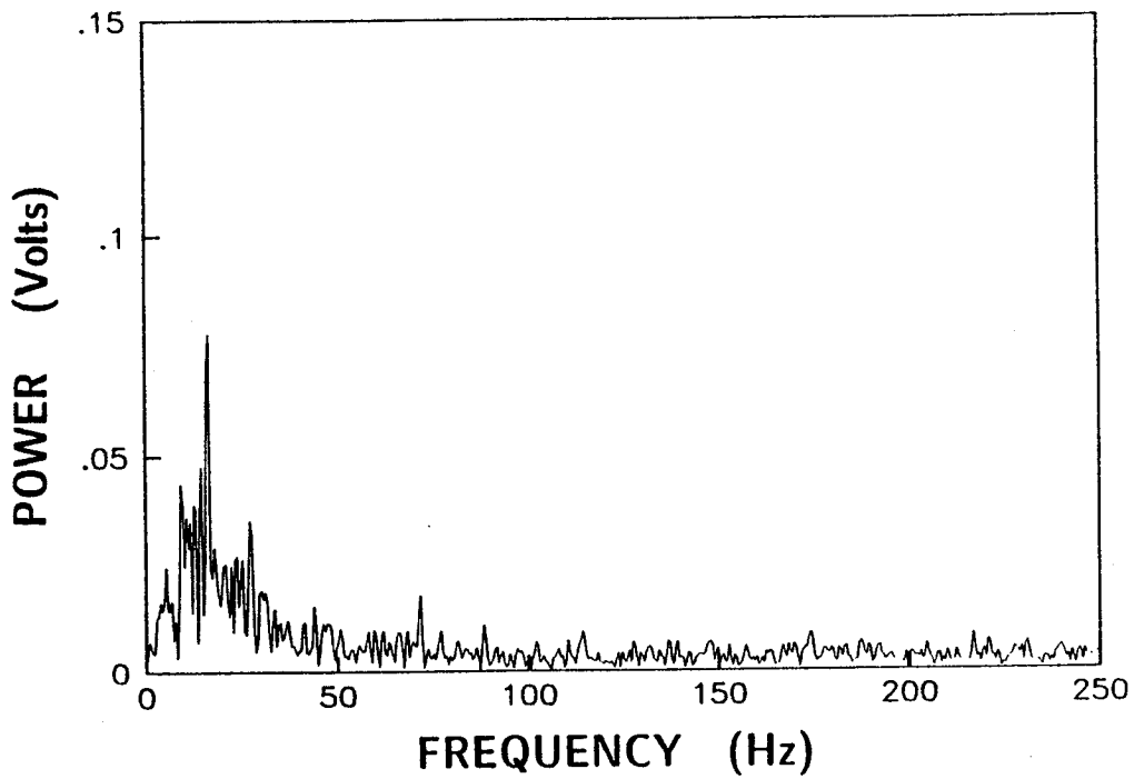
59b. X = 4.27 m, U_{\infty} = 20.7 m/s, M_f = 72.3 Hz (counter-rotating)
