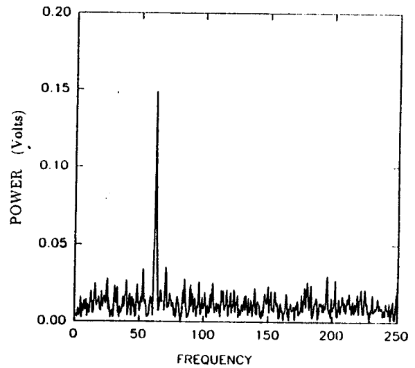
38d. U_{\infty} = 6.2 m/s, M_f = 61.5 Hz, \Delta P = .45 torr (59 Pa), y = 0 .
