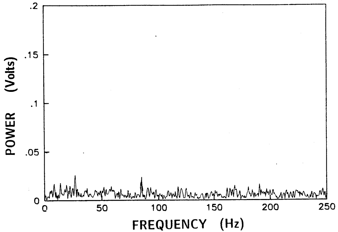
60a. Co-rotating, U_{\infty} = 13.7 m/s, M_f = 85 Hz, \Delta P = 203 Pa
