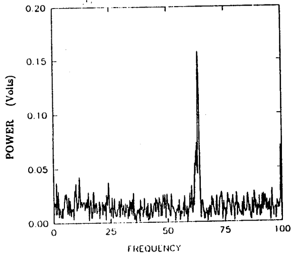
U_{\infty} = 7.8 \text{ m/s}, M_f = 64 \text{ Hz}, \Delta P = 0.76 \text{ torr (101 Pa)}
