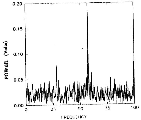
U_{\infty} = 11.8 \text{ m/s}, M_f = 57 \text{ Hz}, \Delta P = 1.39 \text{ torr (185 Pa)}
