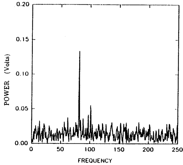
38e. U_\infty = 6.2 m/s, M_f = 81 Hz, \Delta P = .45 torr (59 Pa.), y = -5 mm.
