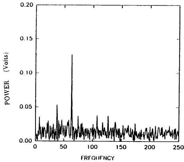
38c. U_{\infty} = 6.2 m/s, M_f = 64 Hz, \Delta P = .45 torr (59 Pa), y = +5 mm.
