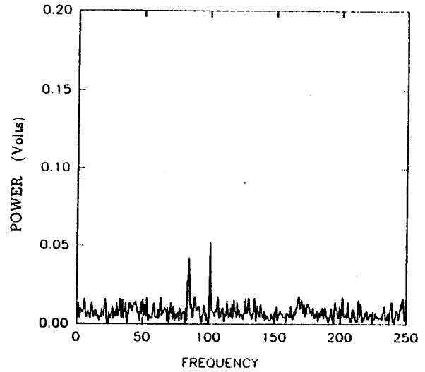
38f. U_\infty = 6.2 m/s, M_f = 86 Hz, \Delta P = .45 torr (59 Pa.), y = -10 mm.
