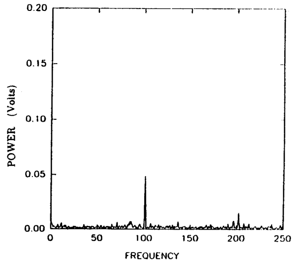
38h. U_\infty = 6.2 m/s, M_f = 83 Hz, \Delta P = .45 torr (59 Pa.), y = -20 mm.
