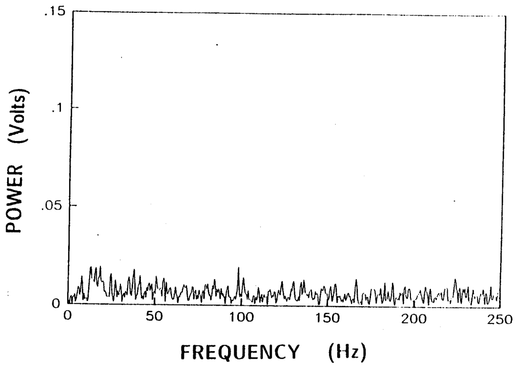
58c. X = 1.73 m, U_{\infty} = 13.7 m/s, M_F = 99 Hz (counter rotating), \Delta P = 176 Pa.
