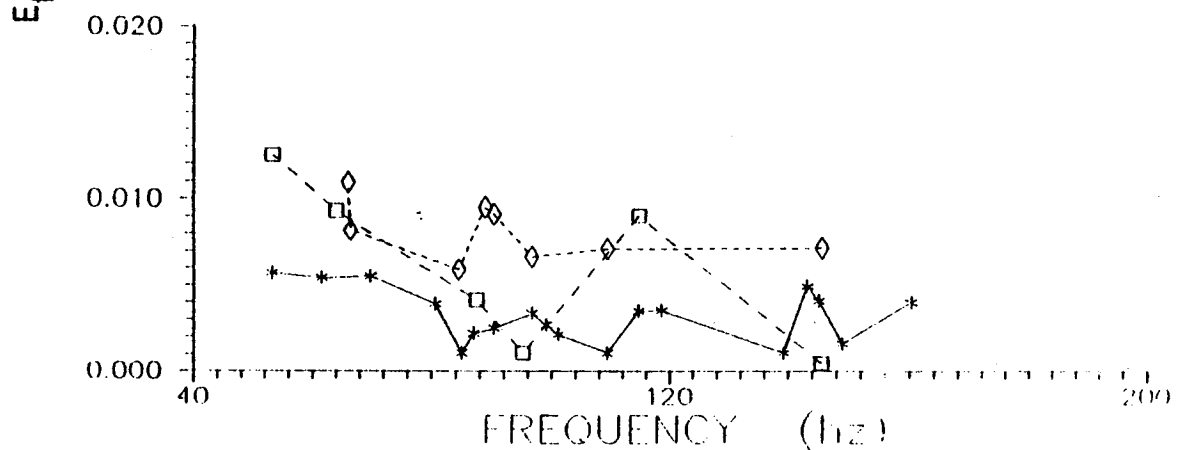
Figure 63. Comparison of co-rotating and counter rotating perturbation energy levels vs frequency at the upstream and downstream probe locations, U_{\infty} = 14 m/s, frequency bandwidth \pm 0.5 Hz.
