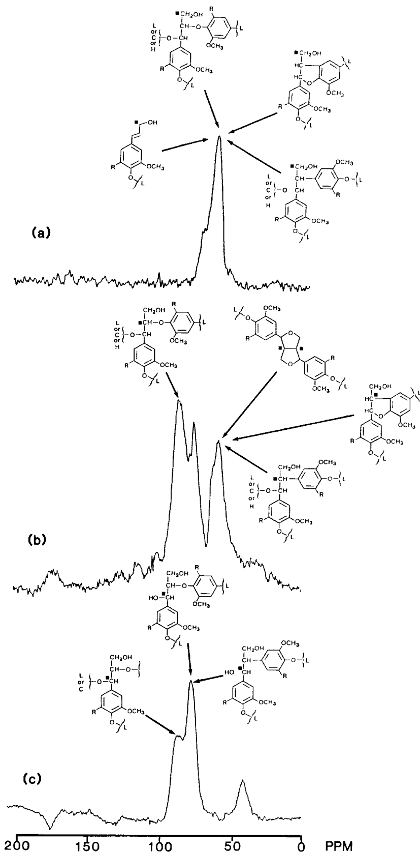
Figure 1. Incorporation of (a) [1- 13 C], (b) [2- 13 C], and (c) [3- 13 C] phenylalanine into L. leucocephala stems. L=lignin; C=carbohydrate
