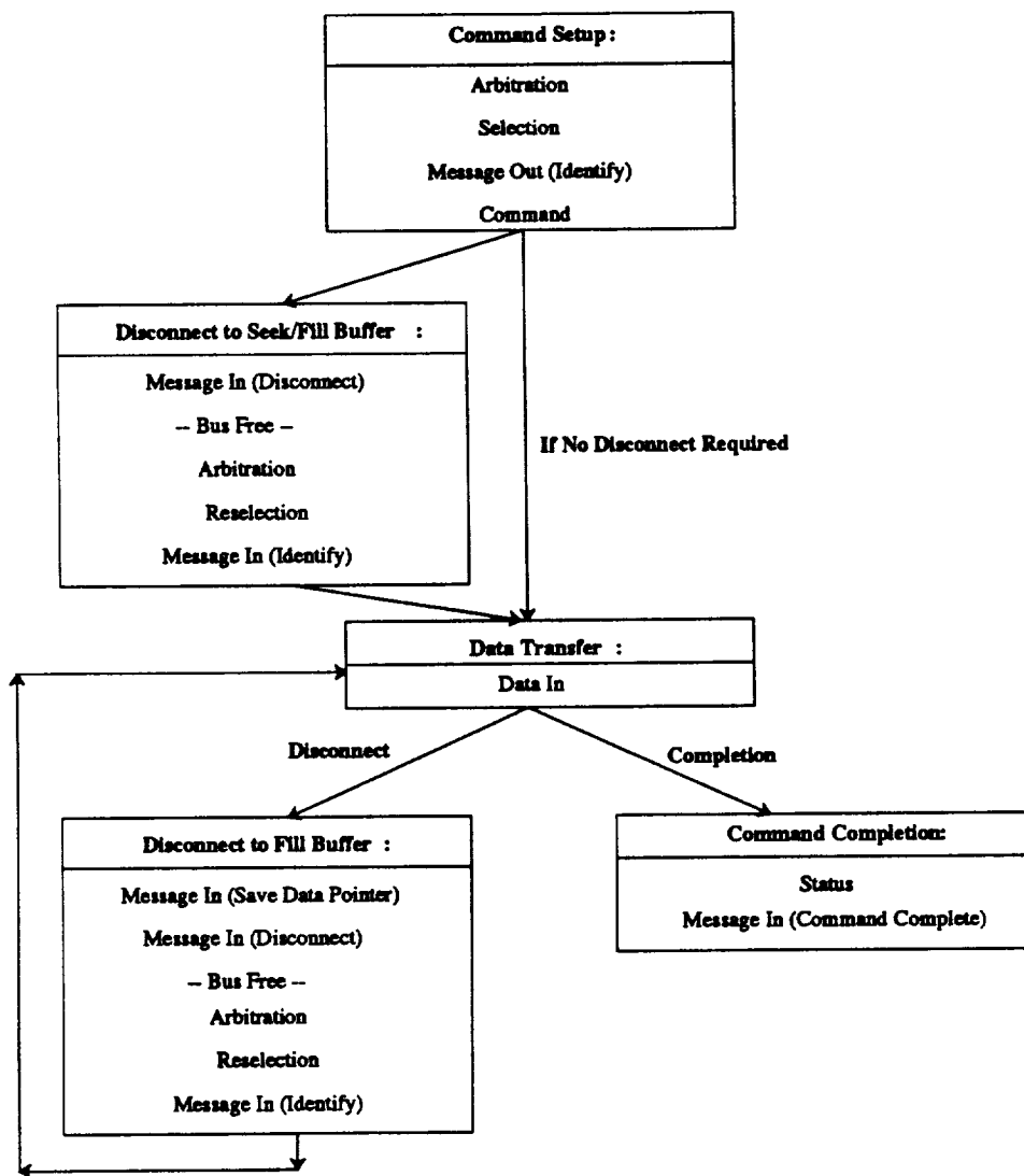
Figure 2: SCSI phase transitions for read operations.
