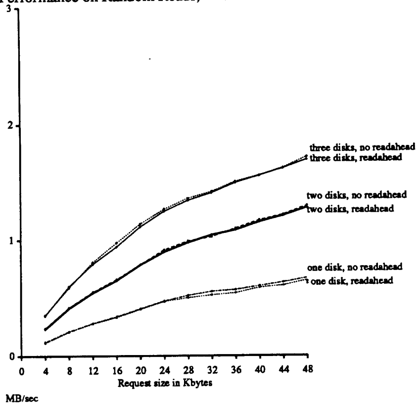
Figure 14: I/O Rates with and without readahead enabled for random reads generated using the no-copy system call to three disks on a string. A separate process issues requests to each active disk.
