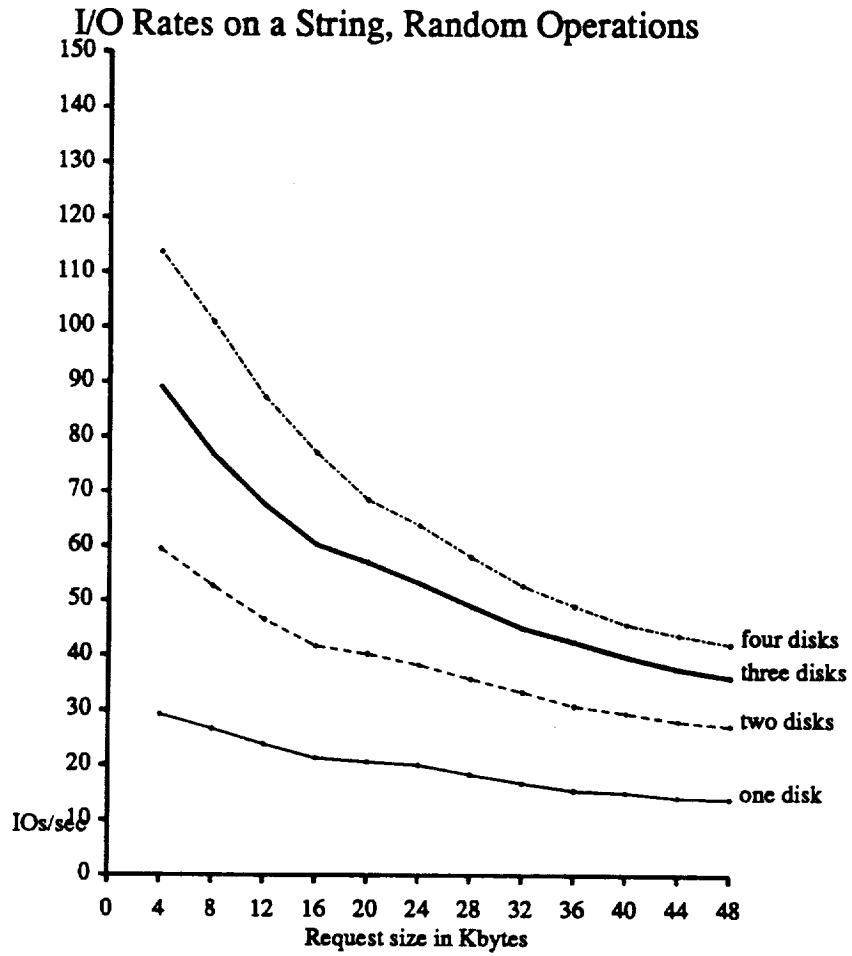
Figure 5: I/O Rates for random operations generated using the no-copy system call. A separate process issues requests to each active disk.
