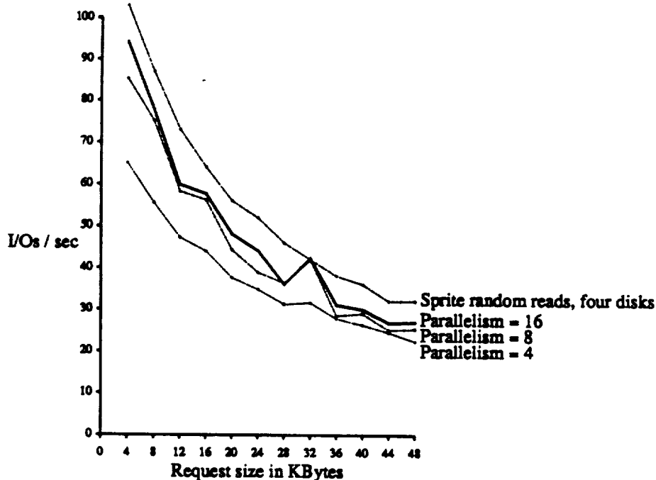
Figure 11: I/O Rates of four disks on one string configured as a single-row RAID device performing random read operations. Parallelism of 4, 8 and 16 indicates the number of independent processes issuing requests to the array. The top line in the graph shows small random reads issued from Sprite user level; it is included for comparison.
