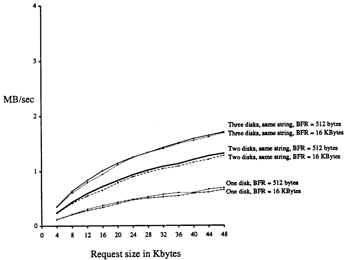
Figure 16: Bandwidth for random reads generated from the no-copy system call for BFR = 512 bytes and BFR = 16 KBytes.
