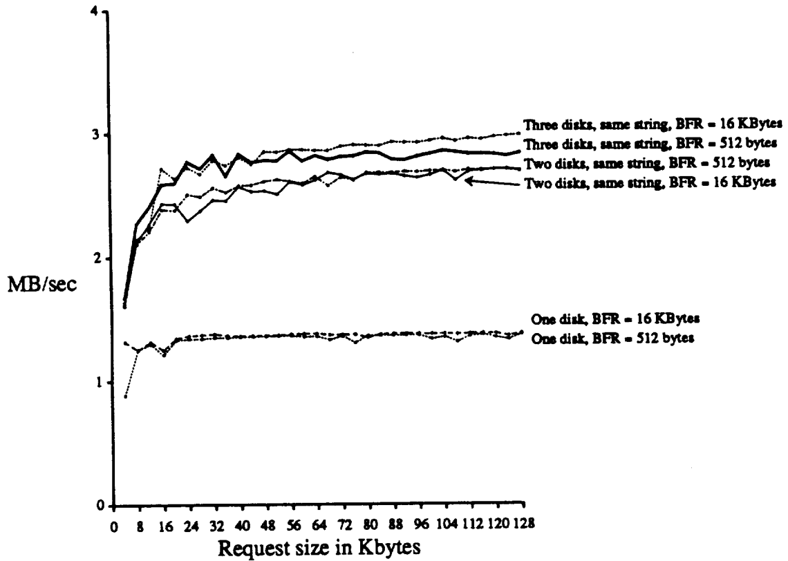
Figure 15: Bandwidth for sequential reads generated using no-copy system call for BFR = 16 KBytes and BFR = 512 bytes.
