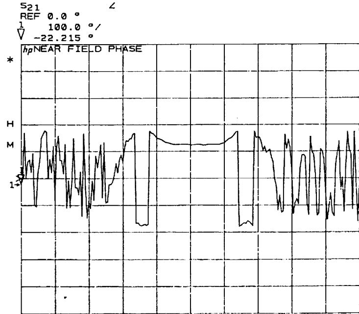
Figure 4.—Near-field phase for AUT.
