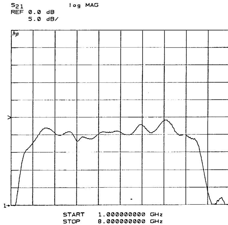
Figure 2.—Fiber optic LO link response.
