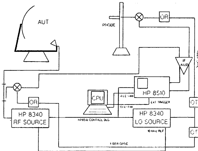
Figure 1.—HP8510 near-field receiver configuration.
