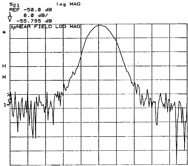
Figure 3.—Near-field amplitude for AUT.
