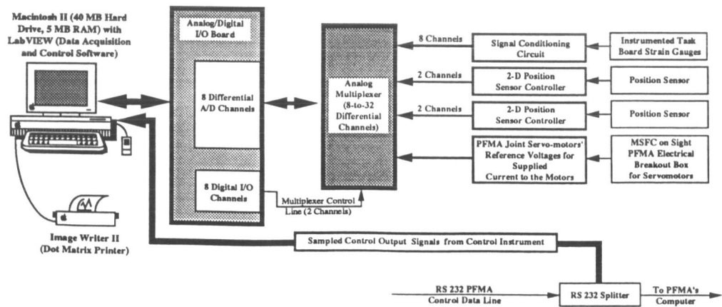
Figure 4 Electronic Data Acquisition System
