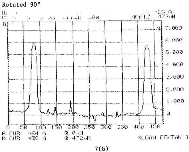
Figure 7 - Polycarbonate Depth Profile
