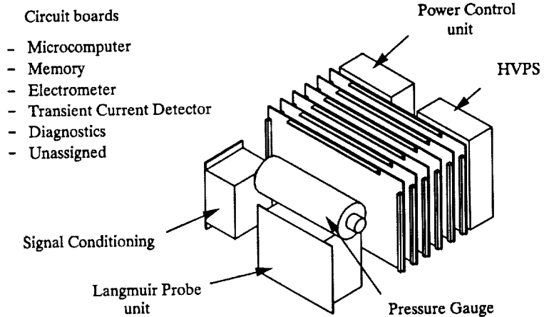
Figure 1 - Current design of experiment package
