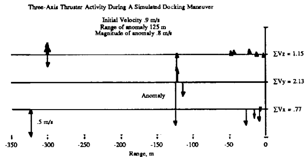
Figure 2: Thruster commands, expert pilot
