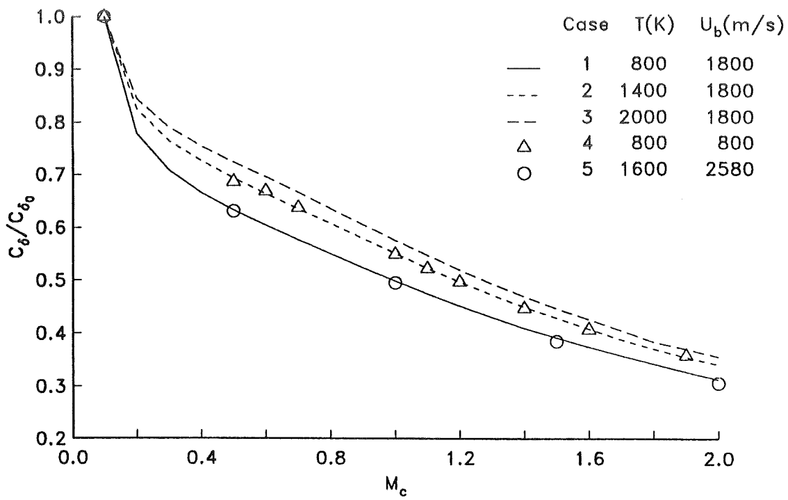
Fig.9 Effect of Temperature on Growth Rate
