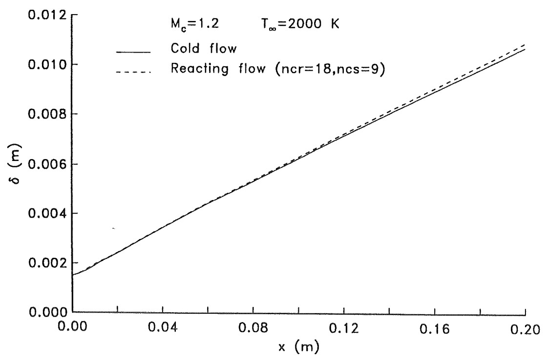
Fig.10 Effect of Reactions on Mixing Layer Growth
