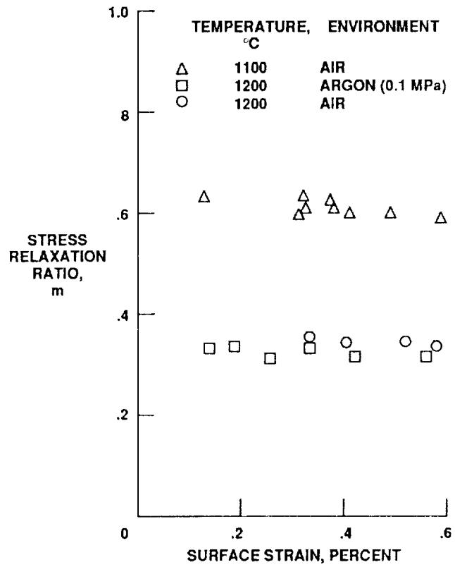
Figure 3.—One hour stress relaxation ratio values versus applied surface strain for SCS-6 fibers.
