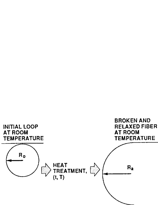
Figure 1.—Schematic representation of BSR test using fiber loops.
