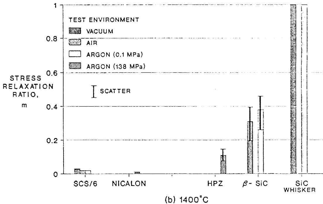
Figure 5.—One hour stress relaxation ratio comparison for various fibers and environments at 1200 °C (a) and 1400 °C (b). Between 4 and 8 fibers were treated for each bar. Surface strain was ~0.3 percent for all fibers except for the SiC whisker (0.05 to 0.15 percent).
