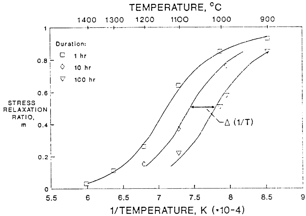
Figure 4.—Stress relaxation ratio versus reciprocal temperature for SCS-6 fibers in air for 1, 10, and 100 hour tests. ( \epsilon_0 \sim 0.3 percent)
