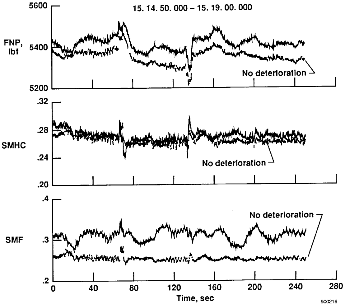
Fig. 19 Sensitivity of CEM estimates to deterioration parameters for PLA = 83°.
