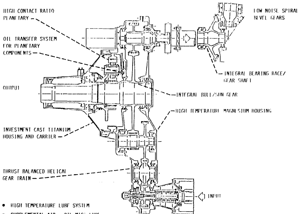
FIGURE 6. - SPLIT TORQUE MAIN GEAR BOX SELECTED BY McDONNELL DOUGLAS HELICOPTER COMPANY.
