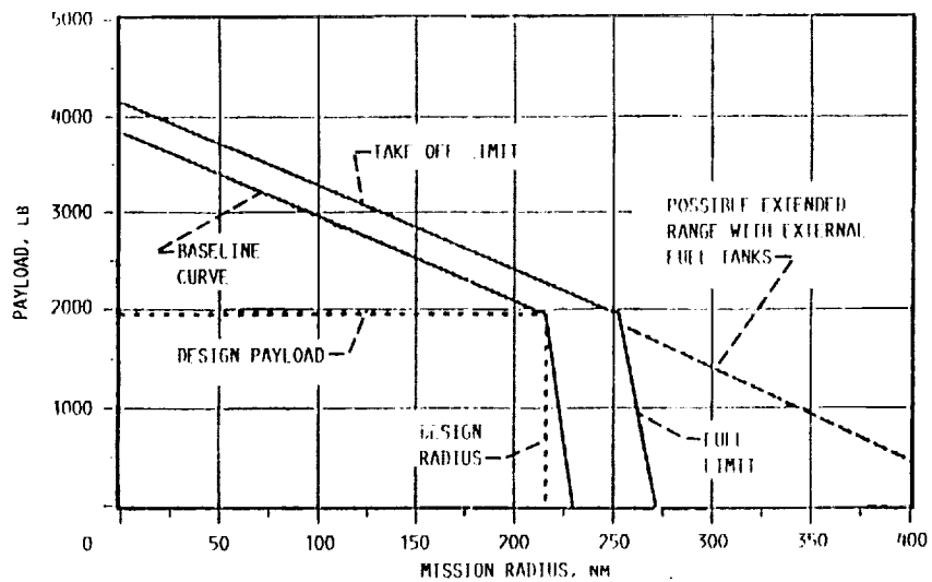
FIGURE 9. - RANGE - PAYLOAD IMPACT OF ART DRIVETRAIN ON BOEING HELICOPTER COMPANY'S FAHV TTR.
