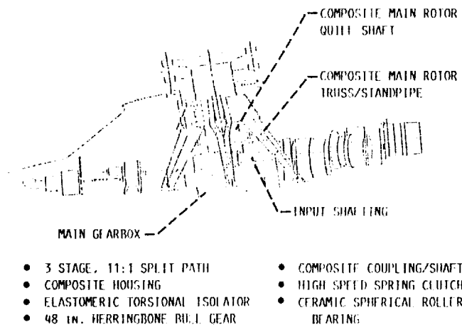
FIGURE 4. - SPLIT PATH MAIN GEAR BOX SELECTED BY SIKORSKY.
