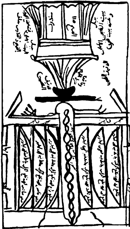
Figure 1-2. A Persian vertical-axis windmill in Sīstān, according to al-Dimashqī, c. A.D. 1300 [Wulff 1966]. The grinding stones are above the rotor with its belying cloth sails. The walls have openings to let the wind in and out. (Reprinted by permission of MIT Press; ©1966, MIT Press)
