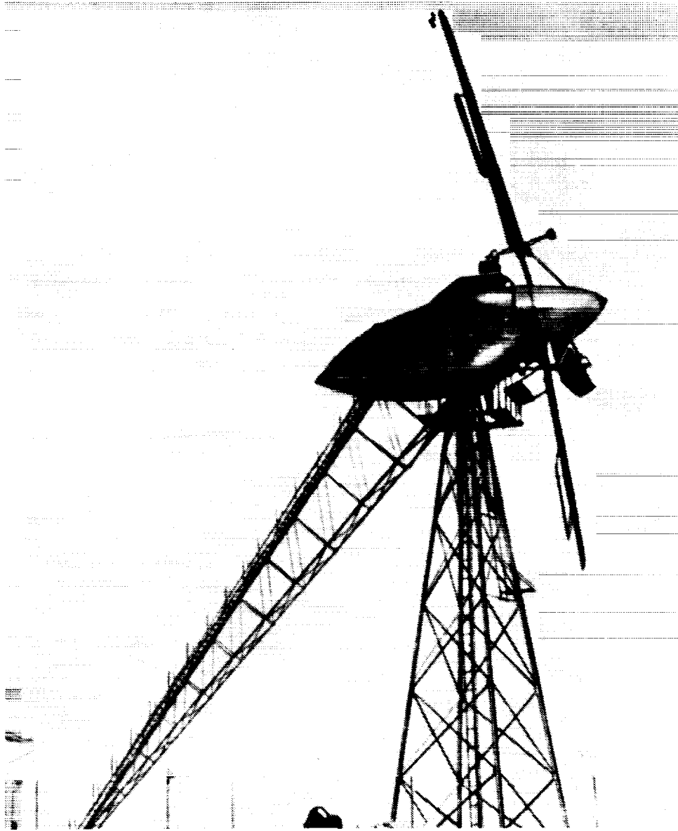
Figure 1-20. Russian wind turbine at Balaclava
