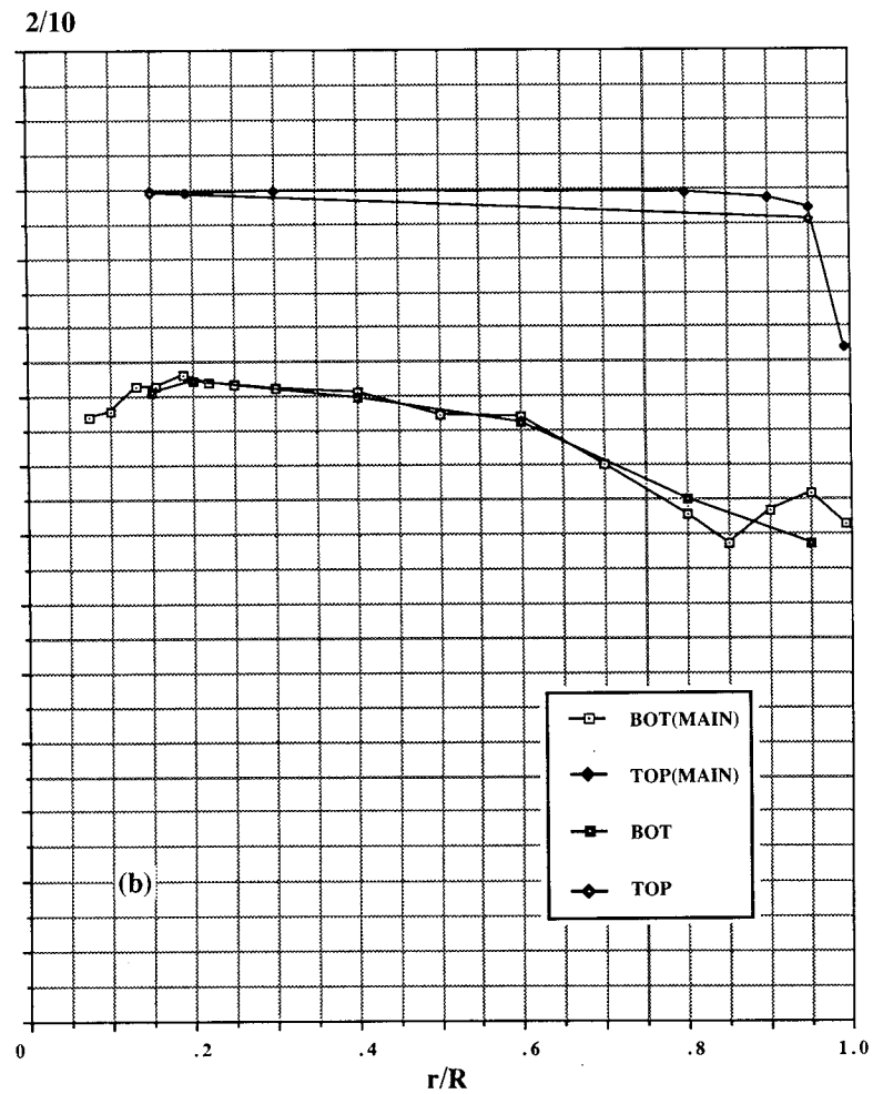
Figure 27. Pressures induced on 20-in. circular plate in ground effect, NPR = 4.0, T = 72 lb, large room. (a) h/d_e = 2.4 , (b) h/d_e = 3.3 .
