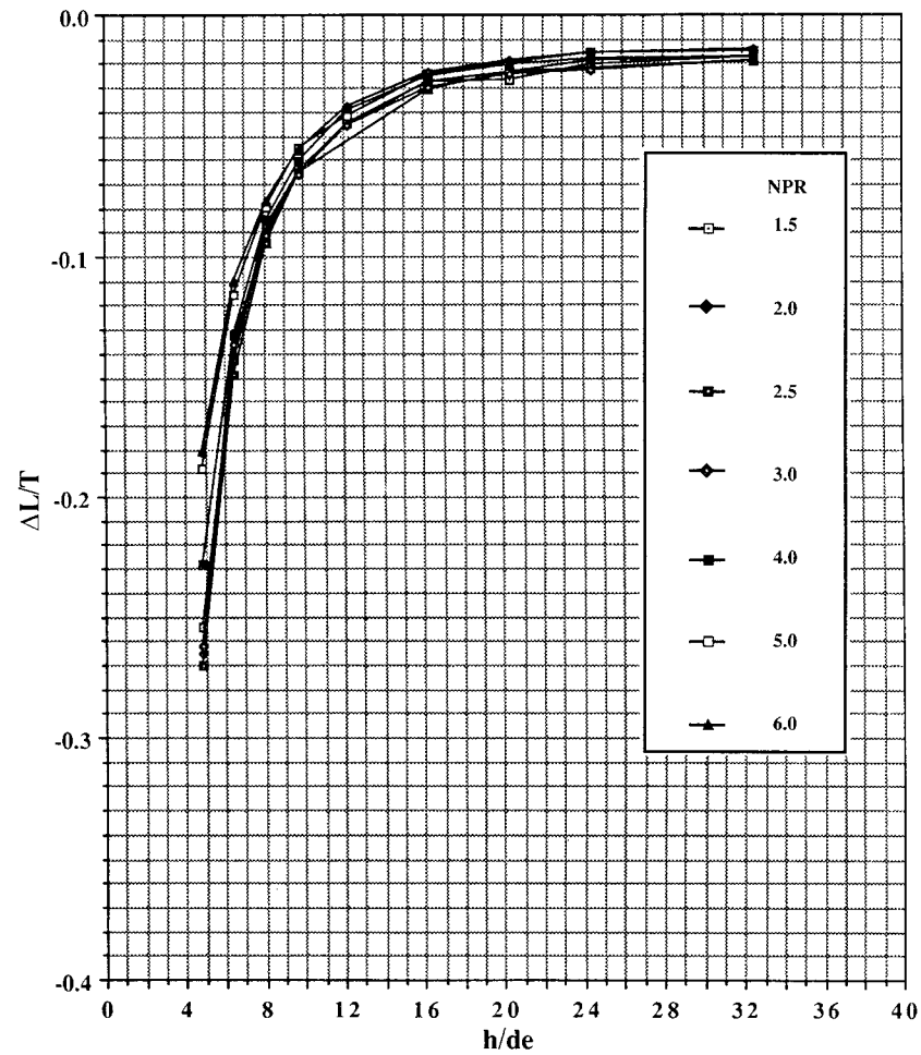
Figure 45. Lift-loss, 20-in. circular plate (Rye), test cell, test cell door half open.
