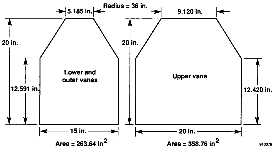
Fig. 3 Dimensions for flight vanes.
