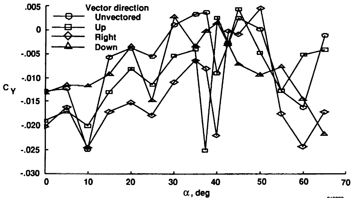
Fig. 26 Side force coefficient as a function of angle of attack, with thrust vectoring varying direction. \delta_{lef} = 34^\circ , \delta_{tef} = 0^\circ , \delta_e = -12^\circ , \delta_a = 0^\circ , \delta_r = 0^\circ , and C_t = 0.8 .
