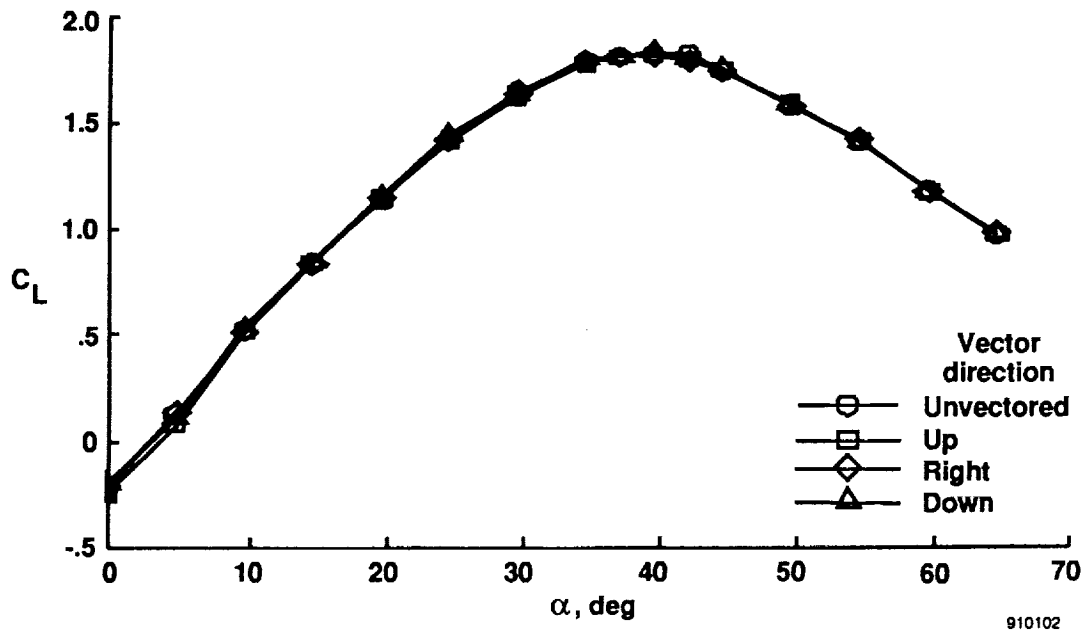
Fig. 29 Lift coefficient as a function of angle of attack, with thrust vectoring vanes set to varying directions and no thrust. \delta_{lef} = 34^\circ , \delta_{tef} = 0^\circ , \delta_e = -12^\circ , \delta_a = 0^\circ , and \delta_r = 0^\circ .
