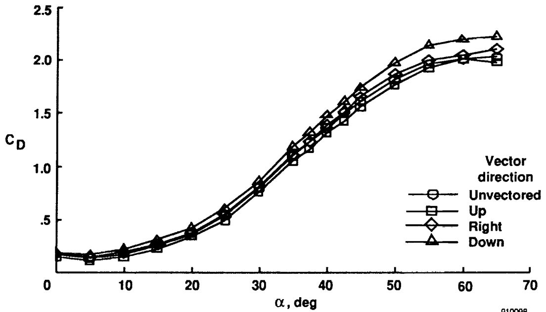
Fig. 25 Drag coefficient as a function of angle of attack, with thrust vectoring varying direction. \delta_{lef} = 34^\circ , \delta_{tef} = 0^\circ , \delta_e = -12^\circ , \delta_a = 0^\circ , \delta_r = 0^\circ , and C_t = 0.8 .
