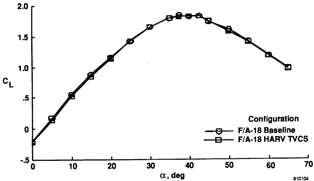
Fig. 31 Lift coefficient as a function of angle of attack, with TVCS installed compared to baseline F/A-18 (no TVCS installed) and no thrust. \delta_{\ell ef} = 34^\circ , \delta_{tef} = 0^\circ , \delta_e = -12^\circ , \delta_a = 0^\circ , and \delta_r = 0^\circ .
