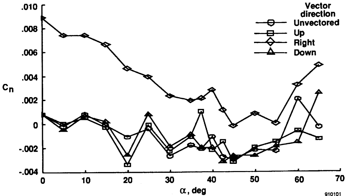
Fig. 28 Yawing moment coefficient as a function of angle of attack, with thrust vectoring varying direction. \delta_{tef} = 34^\circ , \delta_{lef} = 0^\circ , \delta_e = -12^\circ , \delta_a = 0^\circ , \delta_r = 0^\circ , and C_t = 0.8 .
