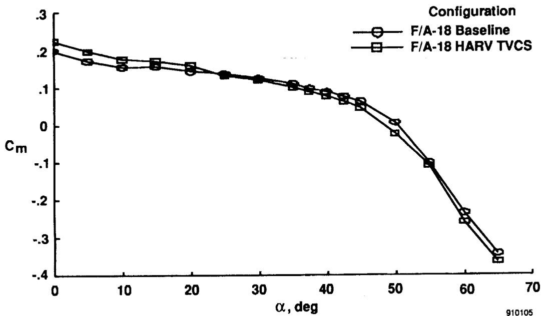
Fig. 32 Pitching moment coefficient as a function of angle of attack, with TVCS installed compared to baseline F/A-18 (no TVCS installed) and no thrust. \delta_{\ell ef} = 34^\circ , \delta_{tef} = 0^\circ , \delta_e = -12^\circ , \delta_a = 0^\circ , and \delta_r = 0^\circ .
