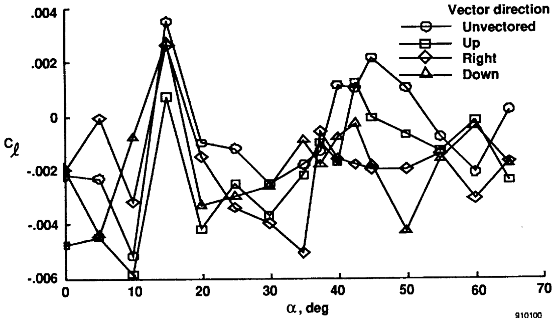
Fig. 27 Rolling moment coefficient as function of angle of attack, with thrust vectoring varying direction. \delta_{tef} = 34^\circ , \delta_{lef} = 0^\circ , \delta_e = -12^\circ , \delta_a = 0^\circ , \delta_r = 0^\circ , and C_t = 0.8 .
