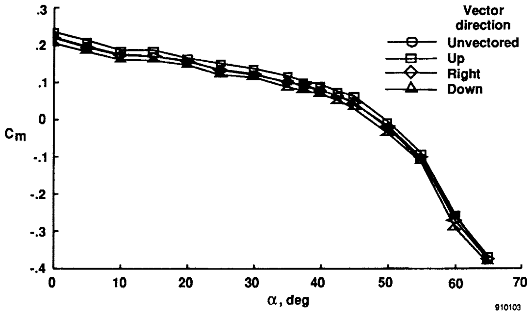
Fig. 30 Pitching moment coefficient as a function of angle of attack, with thrust vectoring vanes set to varying directions and no thrust. \delta_{lef} = 34^\circ , \delta_{tef} = 0^\circ , \delta_e = -12^\circ , \delta_a = 0^\circ , and \delta_r = 0^\circ .
