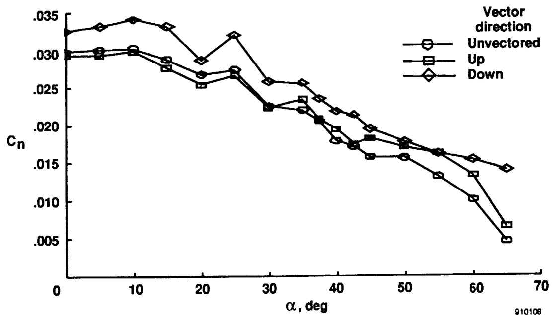
Fig. 35 Yawing moment coefficient as a function of angle of attack, with varying vectoring directions and rudders set to 30^\circ . \delta_{lef} = 34^\circ , \delta_{tef} = 0^\circ , \delta_e = -12^\circ , \delta_a = 0^\circ , and C_l = 0.8 .
