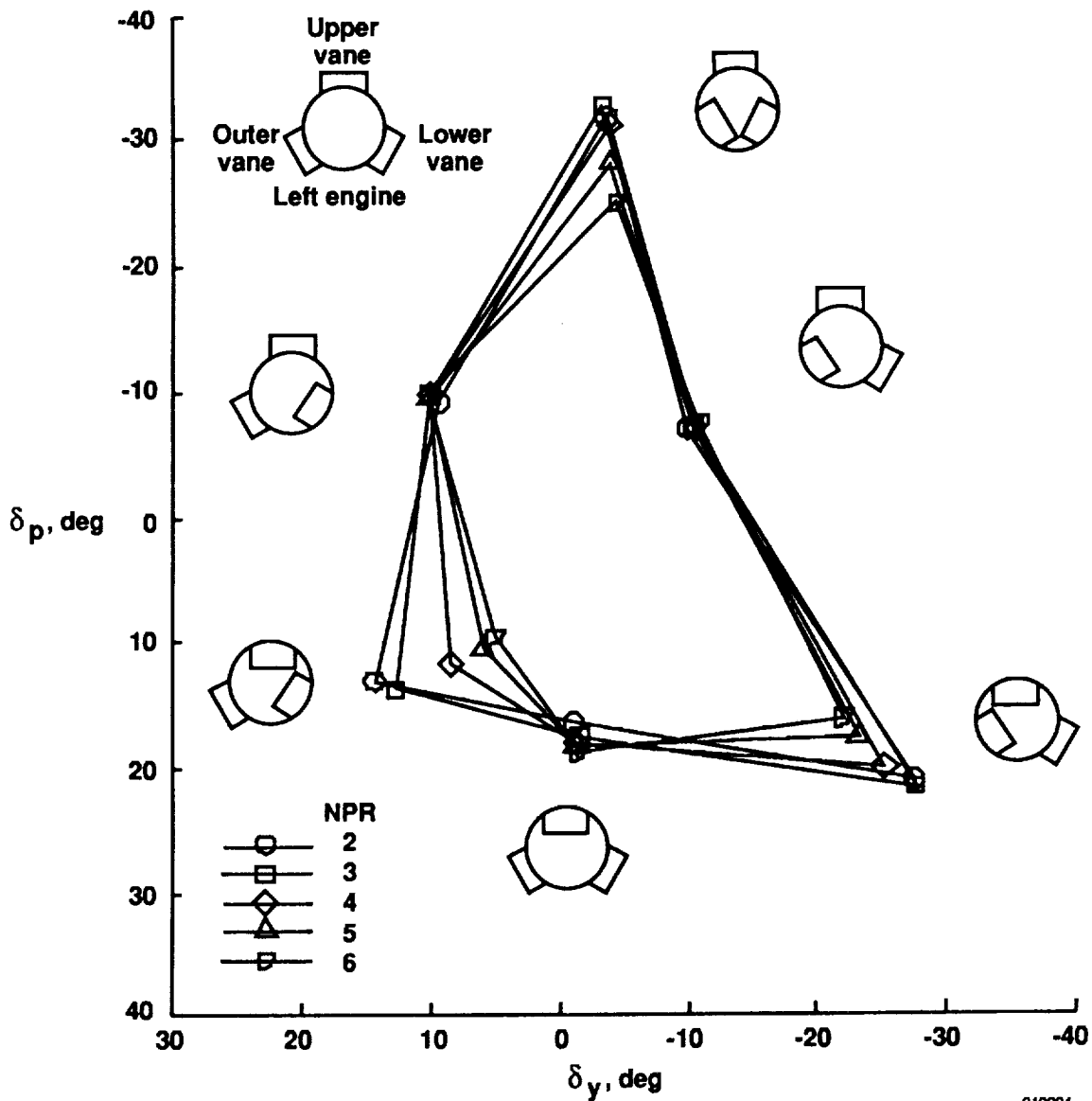
Fig. 21 Maximum jet deflection turning angle envelope, in pitch and yaw, where at least one vane is deflected 30°. Military power nozzle and varying NPR showing retracted vane interference near corners with two-vane equal deflections.
