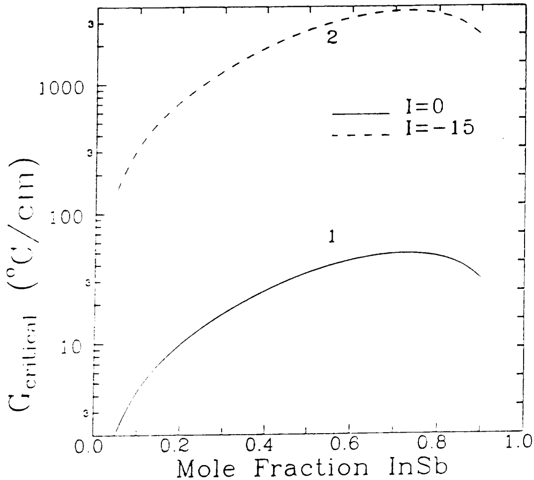
Figure 4.55: A semi-log plot of critical temperature gradient versus liquid composition for InSb-GaSb system with current-induced Peltier cooling. These parameters were used D=2 \times 10^{-5} cm^2/s , H_{GaSb}=1300 J/cm^3 , \rho=0.001 \Omega \cdot cm , V_{nc}=9.25 \times 10^{-6} cm/s (8 mm/day), and \pi_{GaSb}=0.06 volt. Only the Peltier term was considered. The electromigration term was neglected. The curves represent the cases for; 1) I=0 no current-induced effect, 2) I=-15 amp/cm^2 current density (Peltier cooling effect). Above the curves, interface is stable and below the curve, it is unstable.
