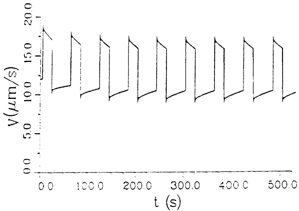
Figure 4.56: Plot of calculated interfacial velocity as a function of time for InSb during periodic application of 9.5 \text{ amp/cm}^2 current for 20 sec on and 40 sec off [91].
