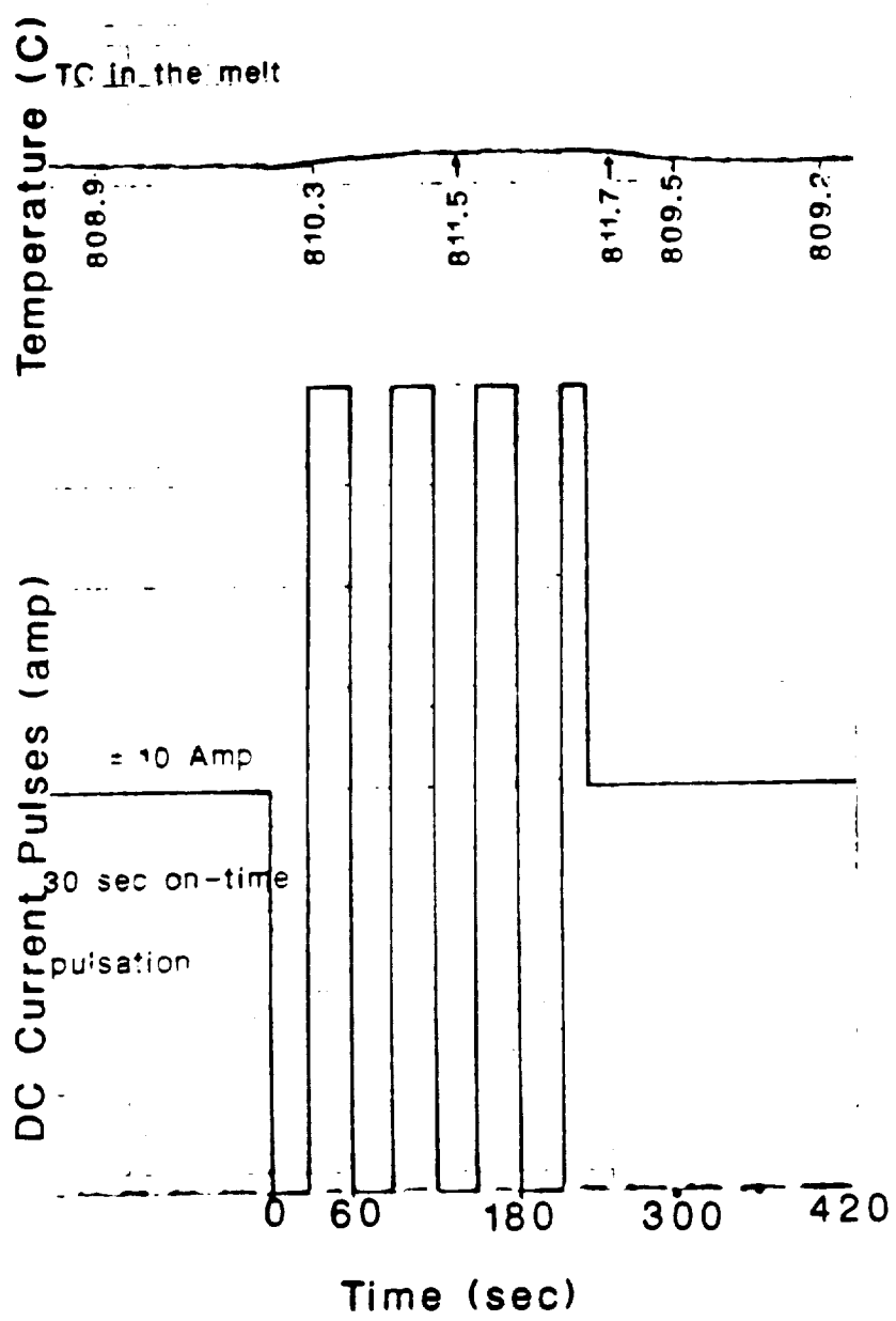
Figure 4.62: Thermocouple readings in molten In_{0.2}Ga_{0.8}Sb during passage of 10 amp current alternating for 30 sec (+) followed by 30 sec (-). The tip of the thermocouple was situated 3.5 cm into the 7 cm long charge.
