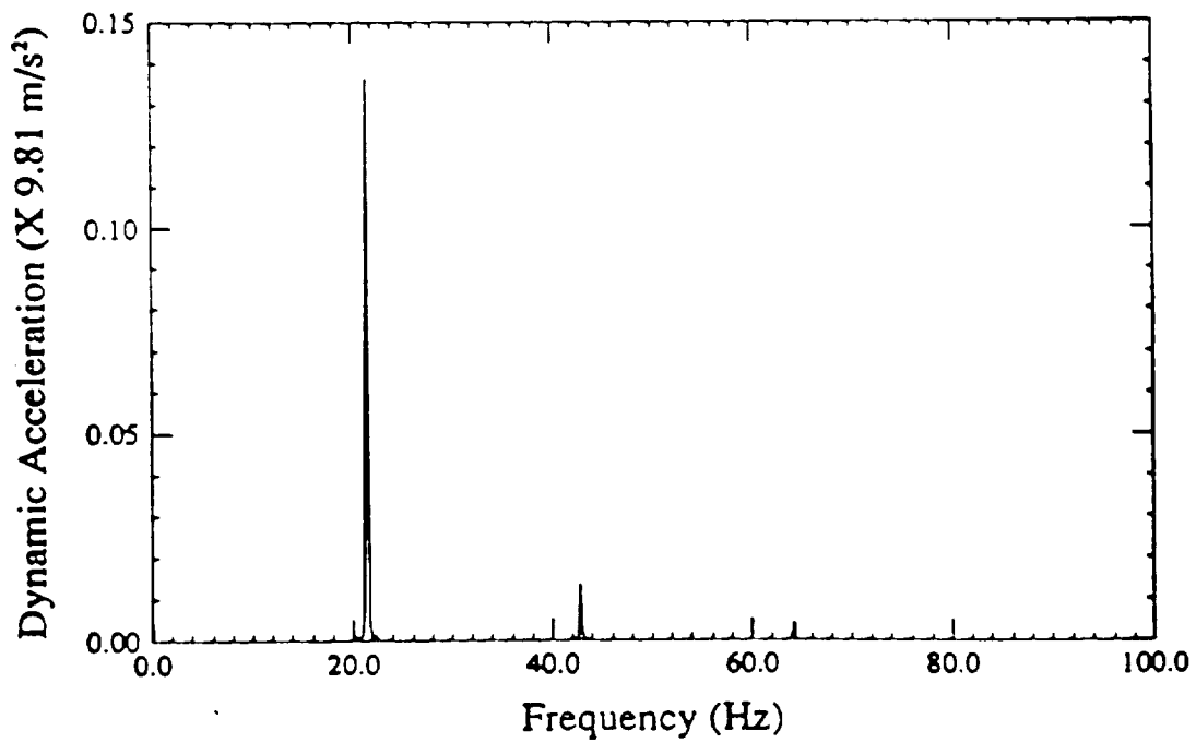
Figure 4.24: Power spectrum of dynamic acceleration at 20 Hz frequency and 0.5 mm amplitude vibration.
