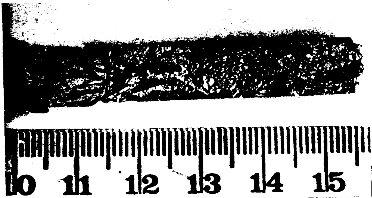
Figure 4.46: Longitudinal section of an ingot with feed composition \text{In}_{0.2}\text{Ga}_{0.8}\text{Sb} frozen at a translation rate of 8 mm/day with application of alternating 15 \text{ amp/cm}^2 current. The ingot was sandblasted to reveal the microstructure. The microstructure exhibits a fine grain structure with microcracks. The growth direction was from left to right.
