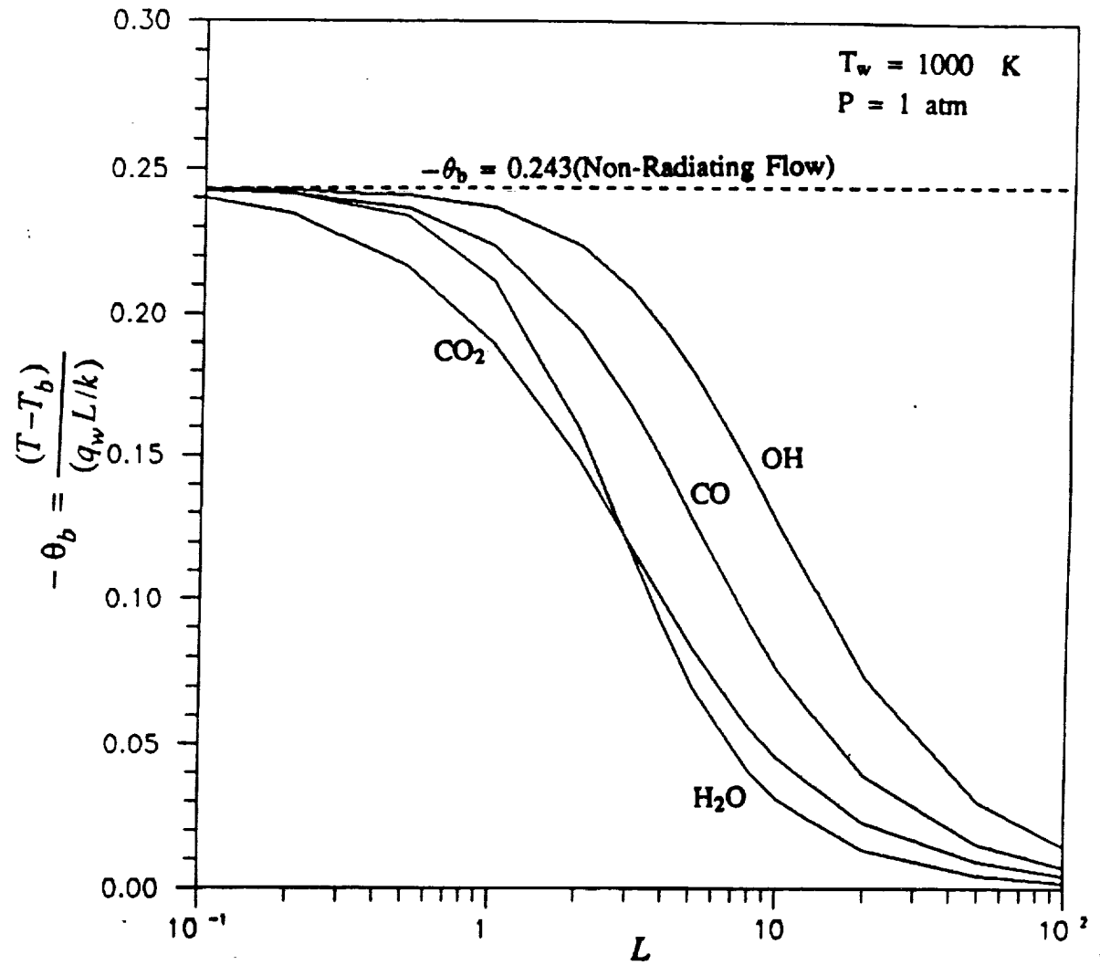
Figure 6.9 Variation of bulk temperature with plate spacing for various species; T_w = 1000 \text{ K} and P = 1 \text{ atm} .
