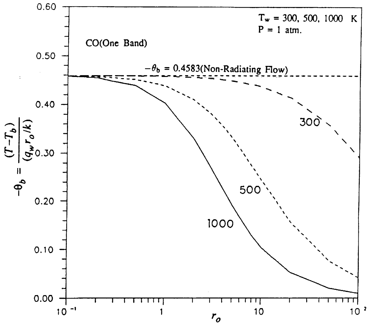
Figure C.7 Variation of bulk temperature with radius for CO;
