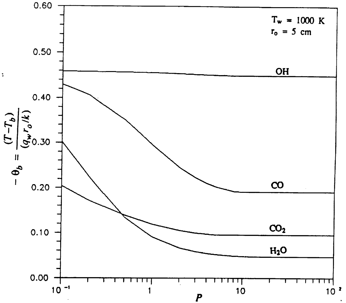
Figure 6.22 Variation of bulk temperature with pressure for various species;
