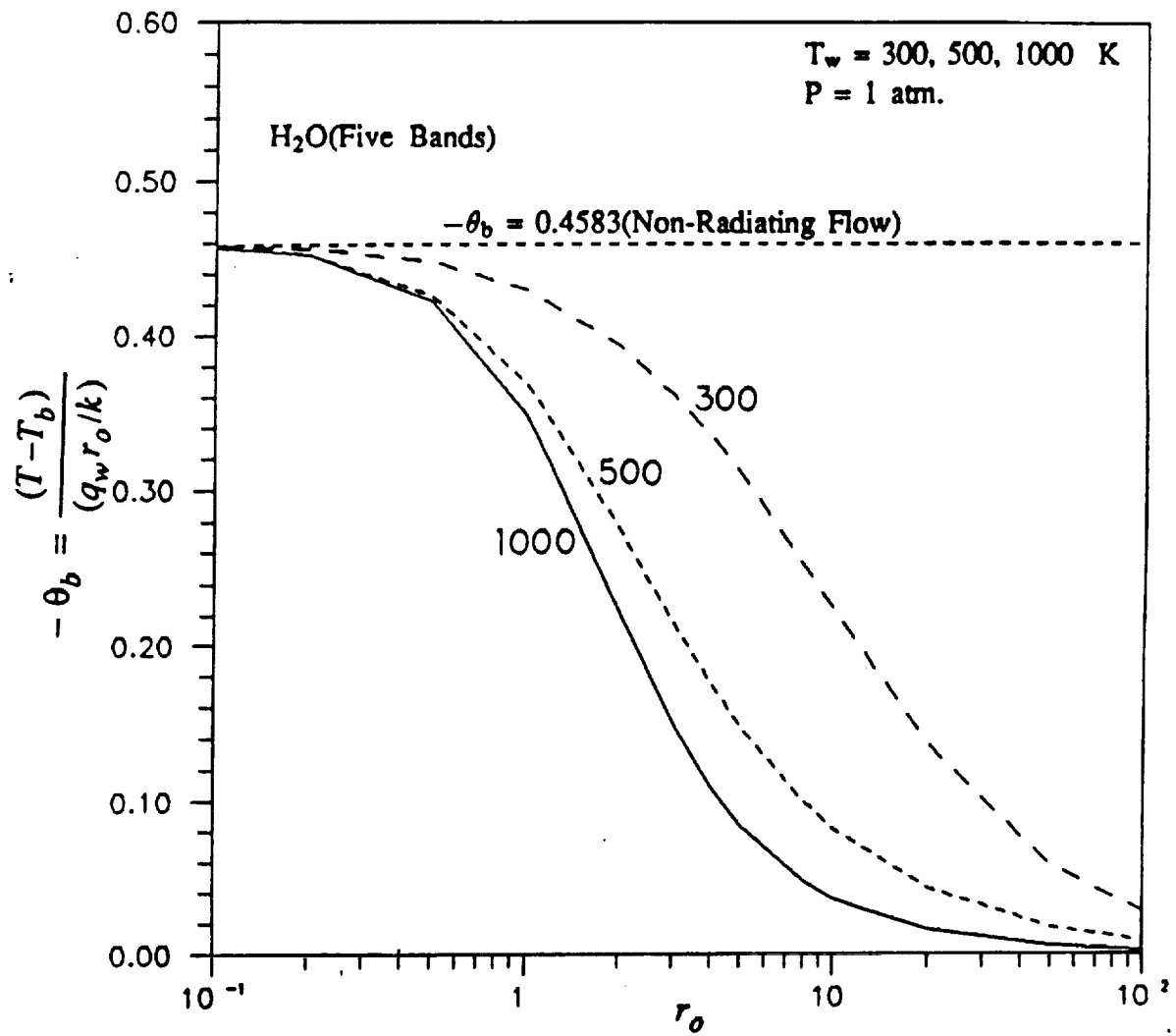
Figure 6.17 Variation of bulk temperature with radius for H 2 O;
