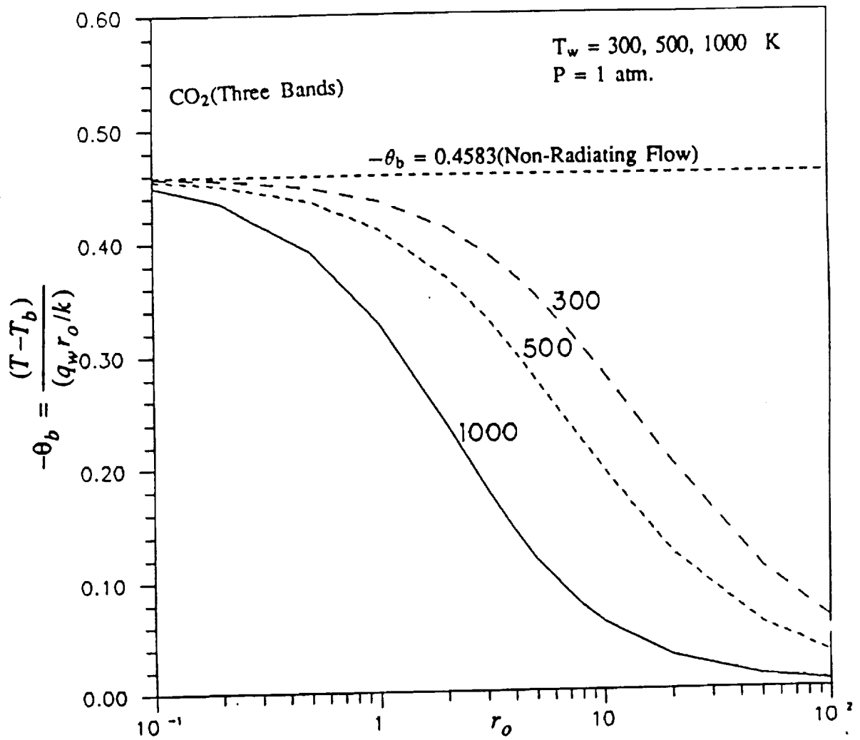
Figure C.4 Variation of bulk temperature with radius for CO 2 ; P = 1 \text{ atm.}
