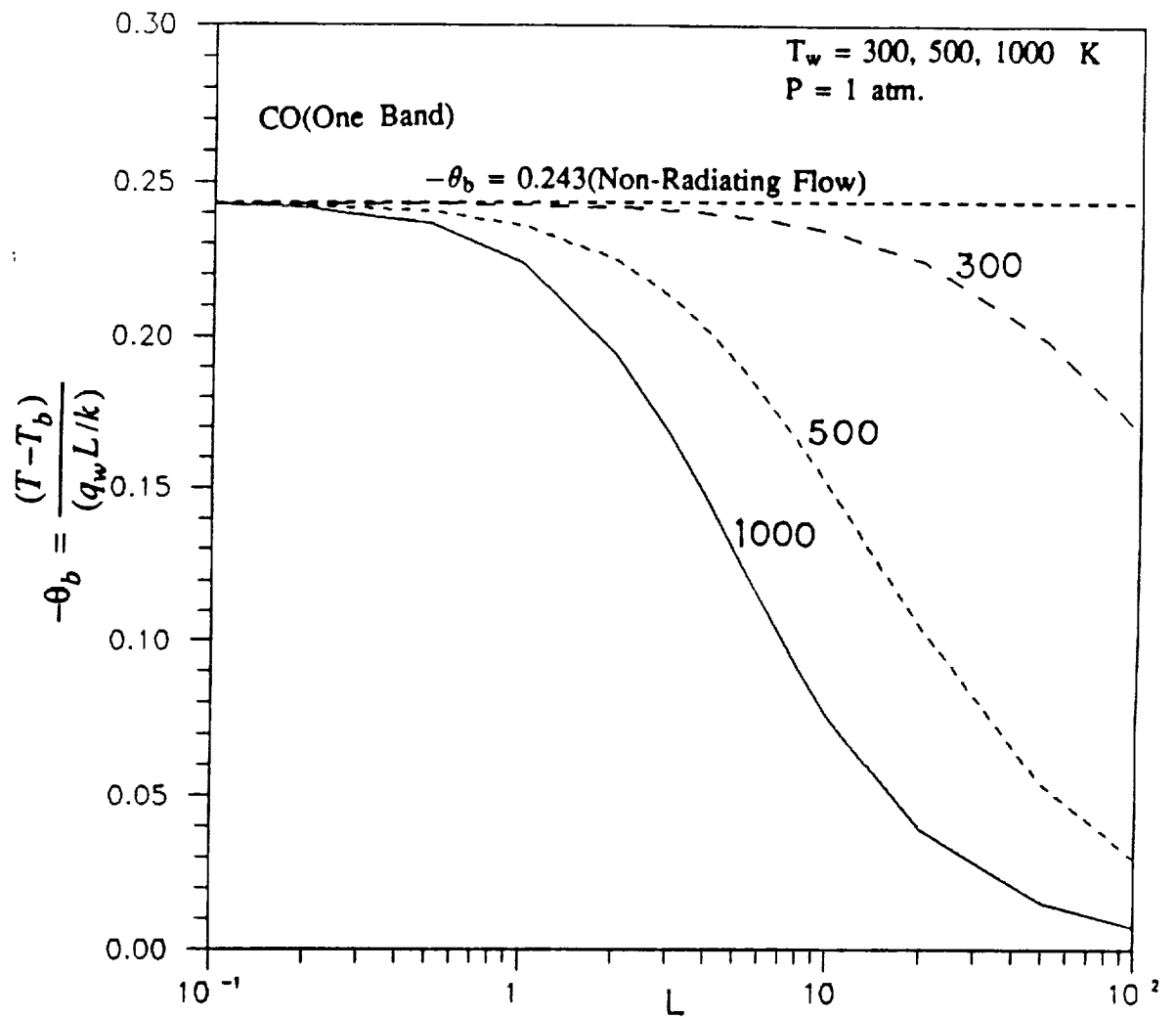
Figure B.8 Variation of bulk temperature with plate spacing for CO; P = 1 \text{ atm.}
