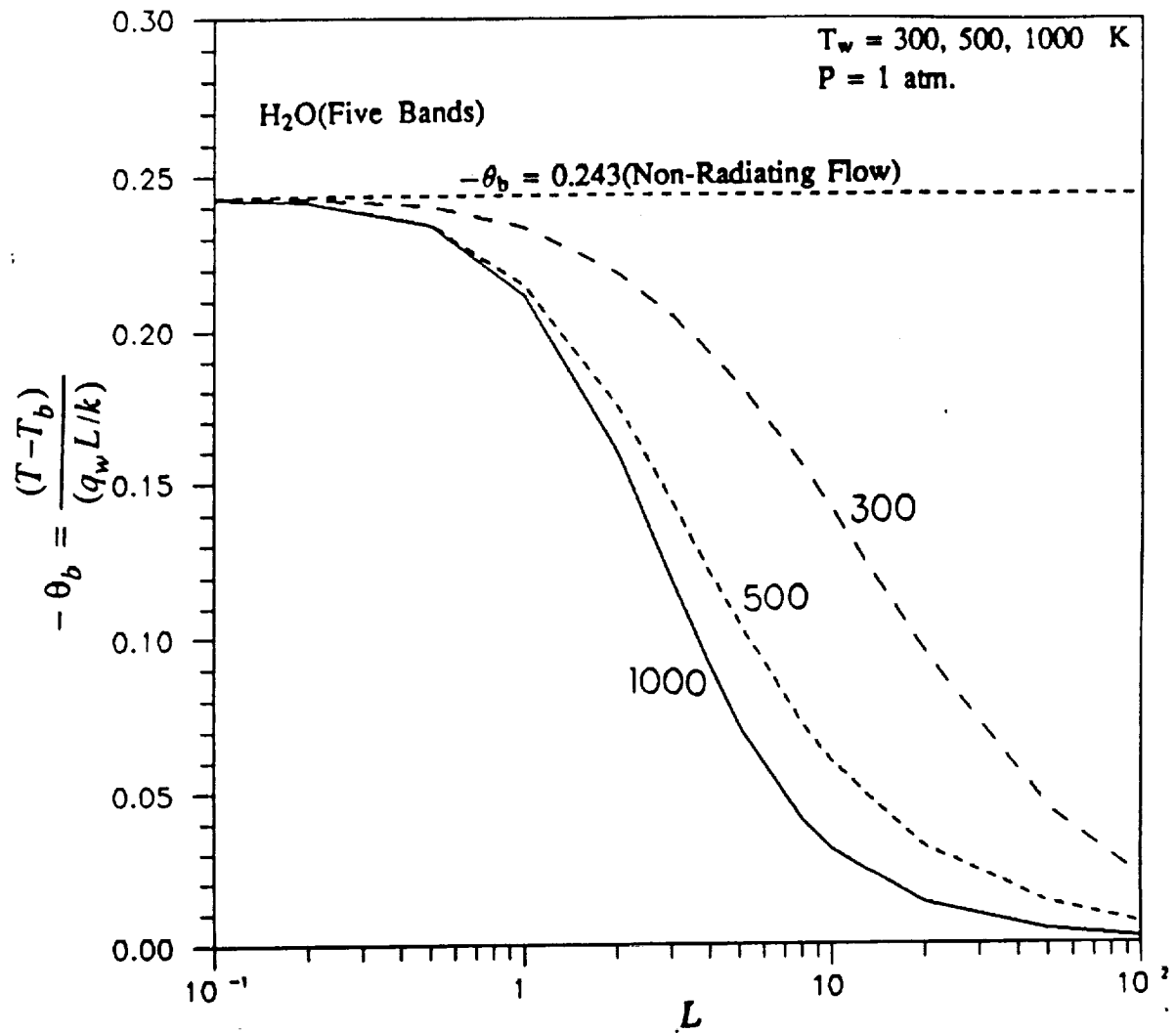
Figure 6.6 Variation of bulk temperature with plate spacing for H_2O ;
