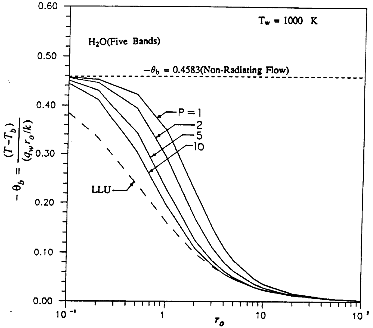
Figure 6.16 Variation of bulk temperature with radius for H_2O ; T_w = 1000\text{ K} .
