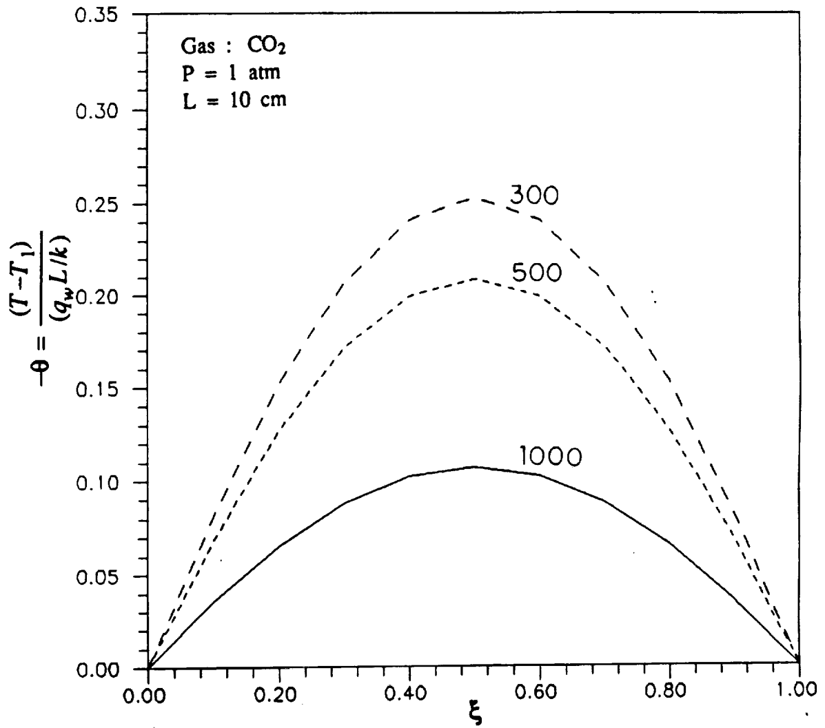
Figure B.1 Comparison of temperature variation across the duct for CO 2 ; T w = 300, 500, 1000 K, P = 1 atm and L = 10 cm.
