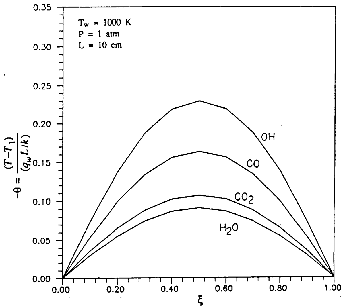
Figure 6.4 Comparison of temperature variations across the duct for various species; T_w = 1000 \text{ K} , P = 1 \text{ atm} and L = 10 \text{ cm} .
