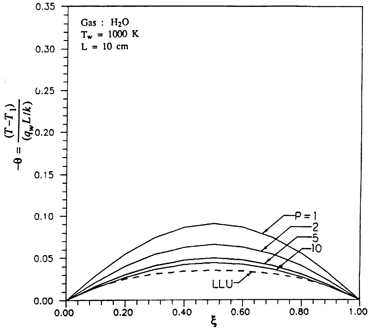
Figure 6.3 Comparison of temperature variations across the duct for H 2 O;
