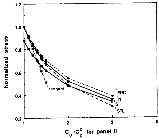
Figure 5. Approximations to von Mises stress at node 59.
