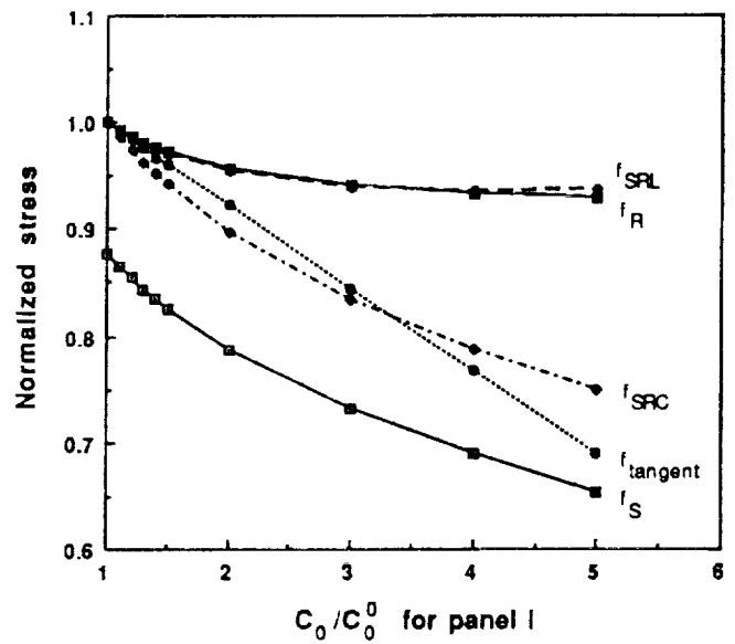
Figure 4. Approximations to von Mises stress at node 59.
