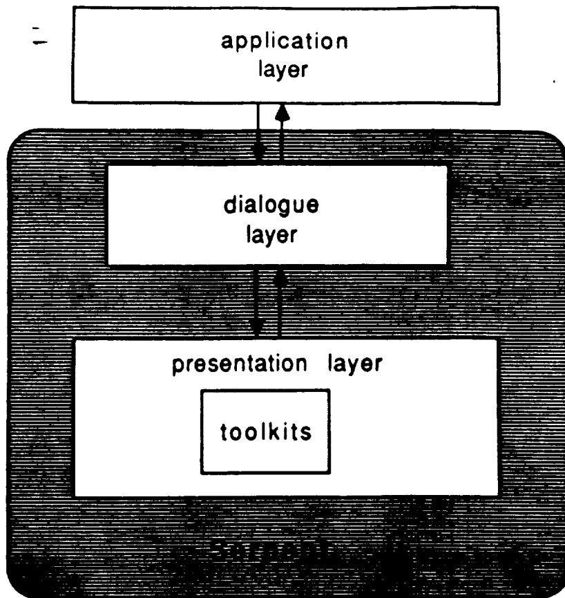
Figure 1: Serpent Architecture
