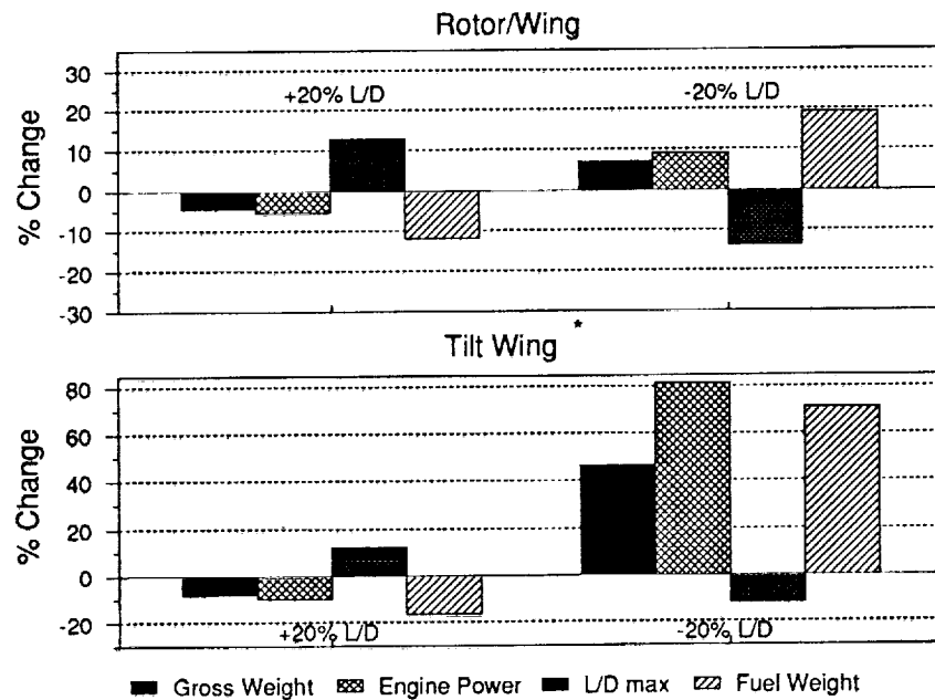
FIGURE 2-33. SENSITIVITY TO CHANGES IN LIFT-TO-DRAG RATIO
