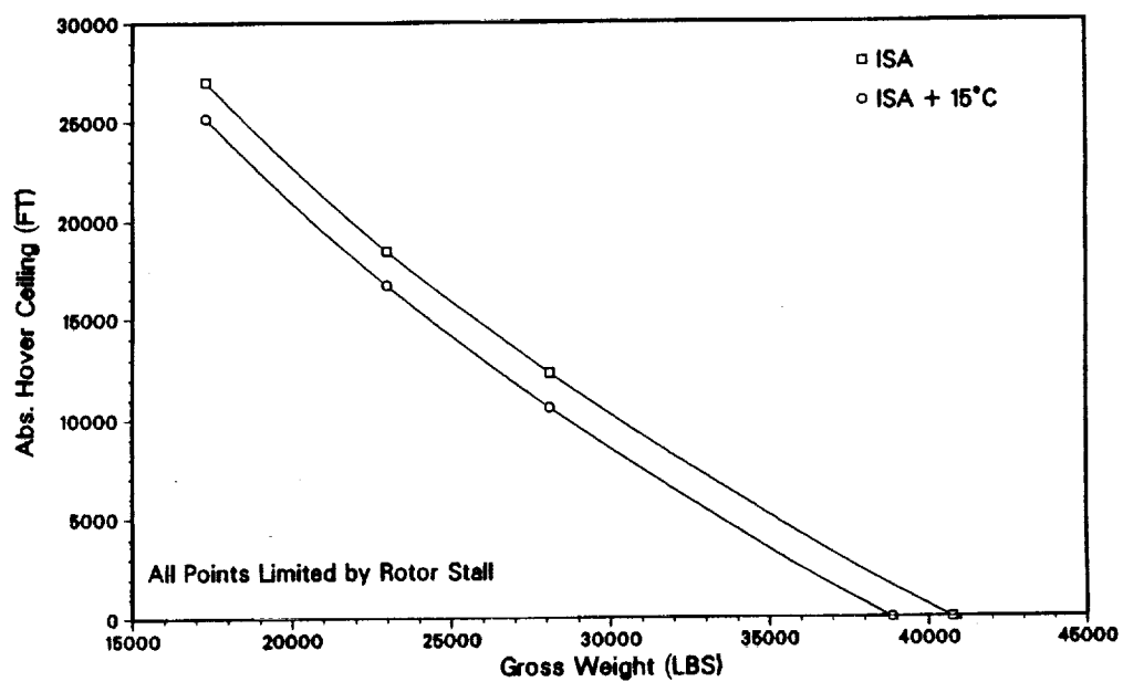
FIGURE 2-20. ROTOR/WING HOVER CEILING
