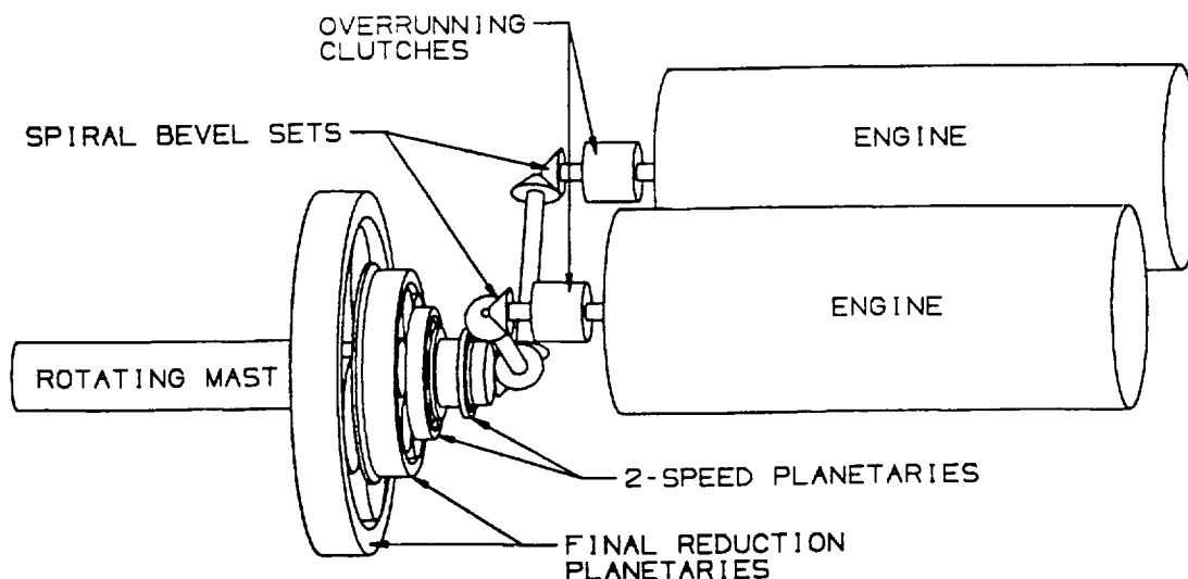
FIGURE 2-26. TILT WING DRIVE SYSTEM
