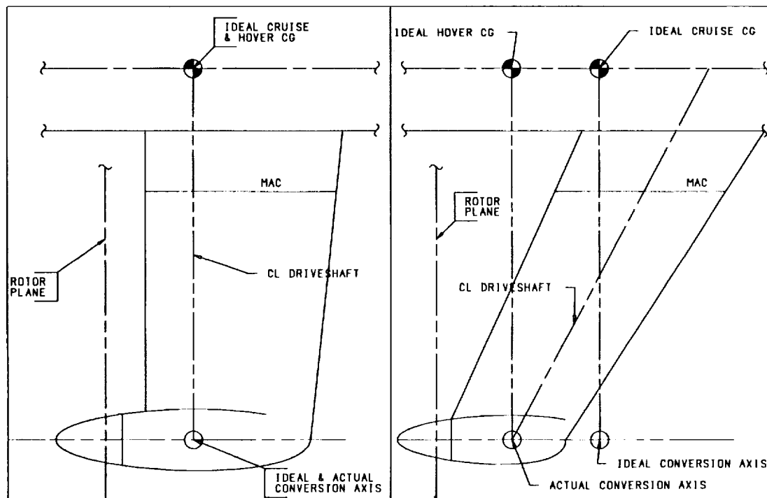
FIGURE 1-27. CONVERSION AXIS - CENTER OF GRAVITY RELATIONSHIP (geometry exaggerated for purposes of illustration)
