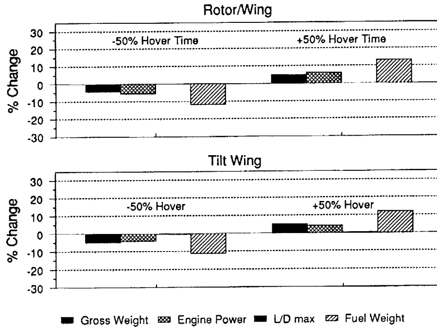
FIGURE 2-32. SENSITIVITY TO CHANGES IN MISSION HOVER TIME
