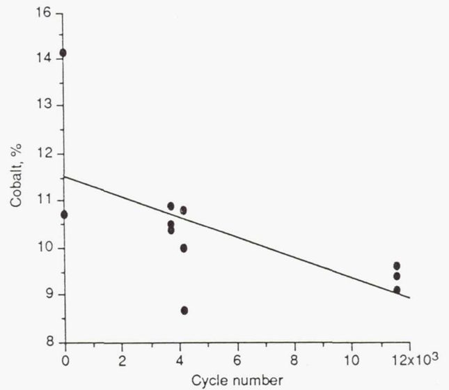
Figure 10.—Co content in the active material against the number of cycles. (See comments for Fig. 9)
