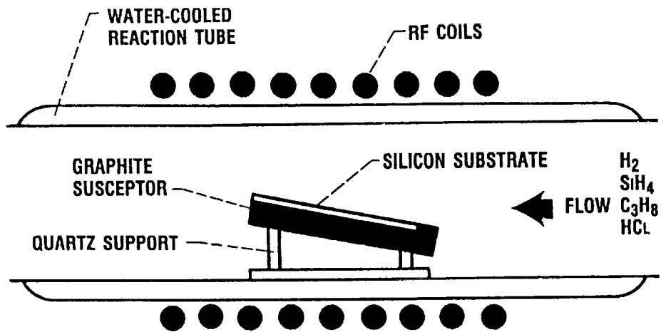
FIGURE 1. SCHEMATIC DIAGRAM OF REACTION CHAMBER FOR EPITAXIAL \text{SiC} CRYSTAL GROWTH
