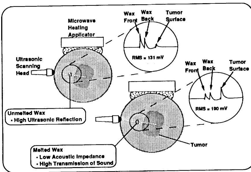
FIGURE 9 ULTRASONIC TUMOR TEMPERATURE MONITOR CONCEPTUAL DIAGRAM
