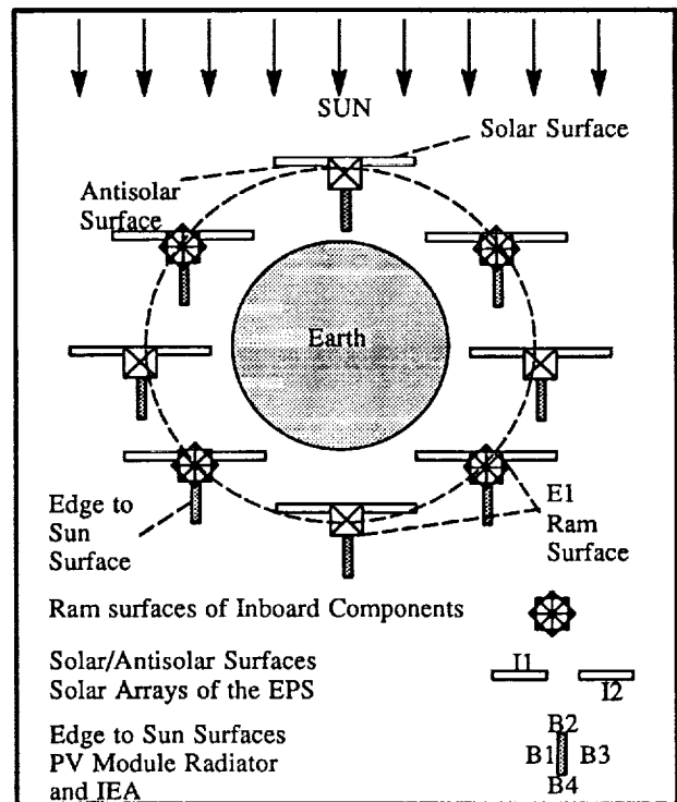
Figure 3. Schematic of EPS Component Surfaces and their Rotations Through One Orbit
