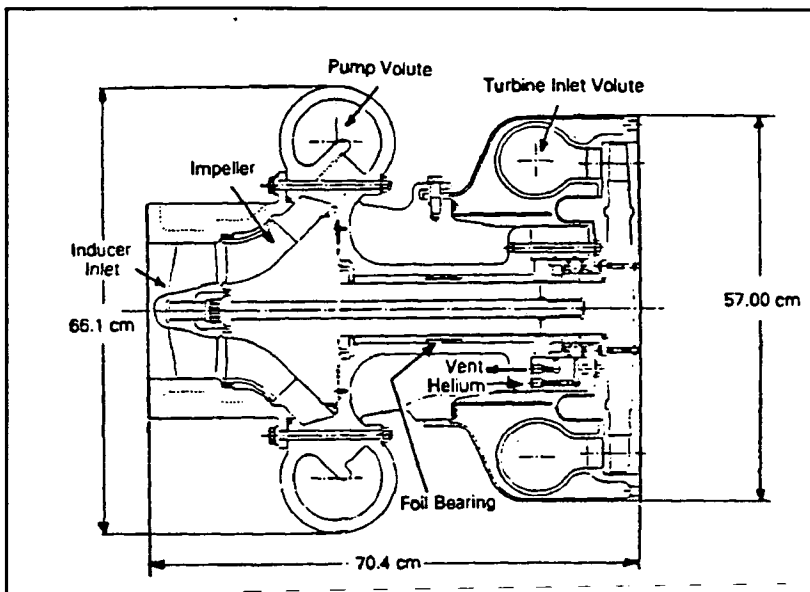
Figure 10 LOX Turbopump
