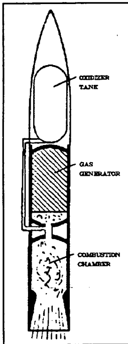
Figure 2 Gas Generator Hybrid
