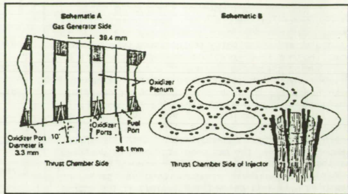
Figure 8 Propellant Injector Manifold
