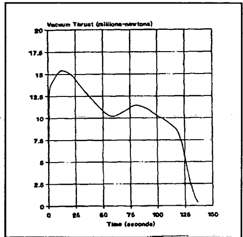
Figure 3 Required Vacuum Thrust Profile
