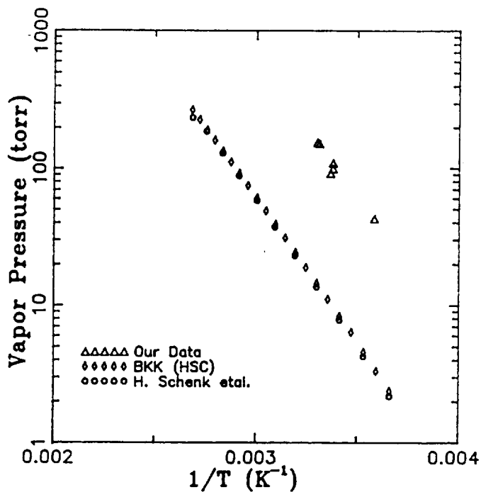
Figure 7 - Comparison of vapor pressure measurements for \text{TiCl}_4 .
