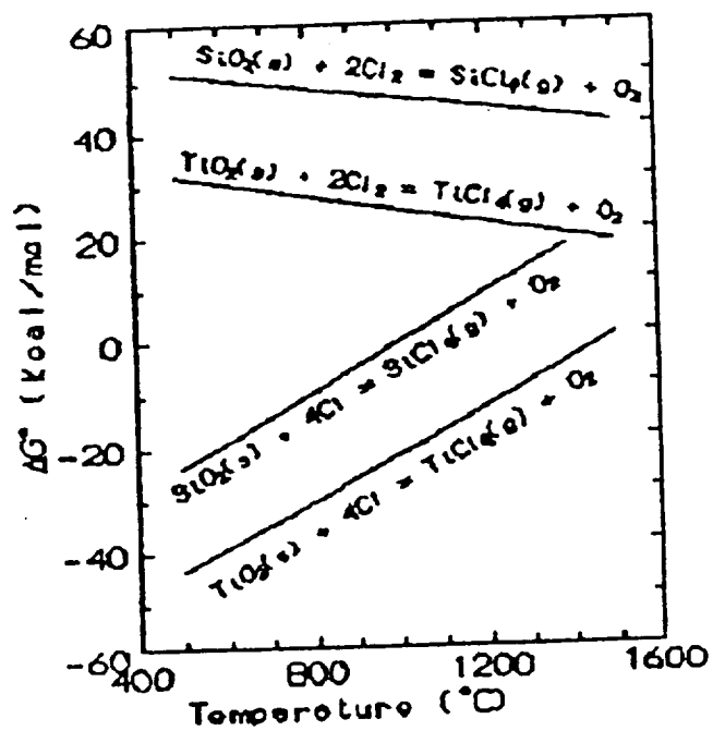
Figure 4 - Standard Gibbs energy data for formation of chlorides.
