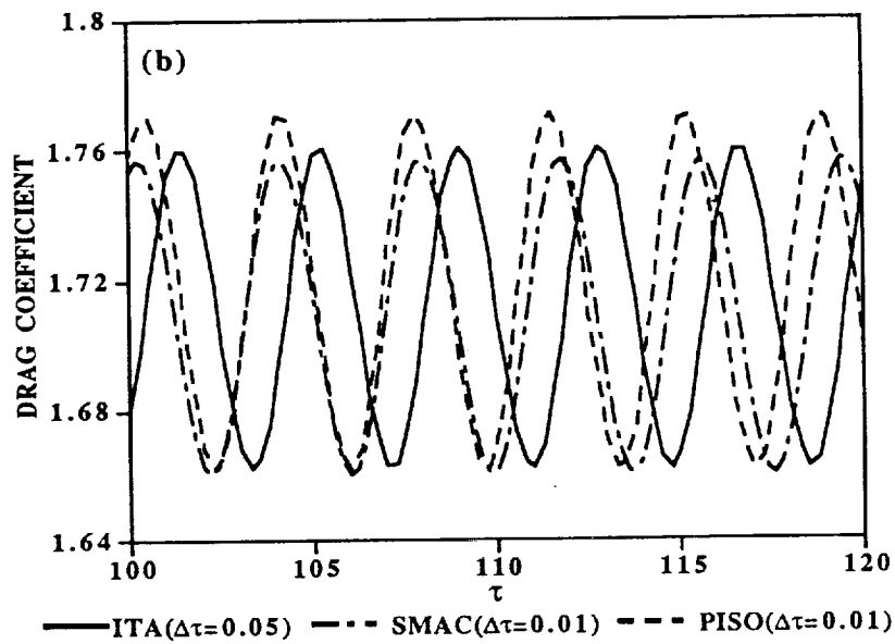
(b) Comparison of ITA, SMAC and PISO.
