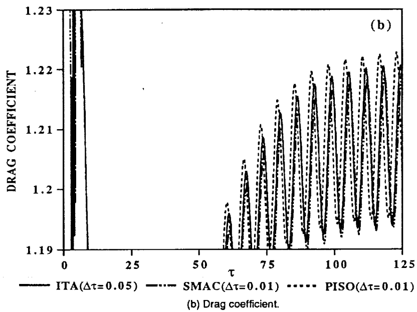
Figure 8.— Lift and drag for flow over a circular cylinder.
