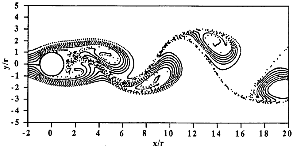
Figure 3.— Streaklines for flow over a circular cylinder.
