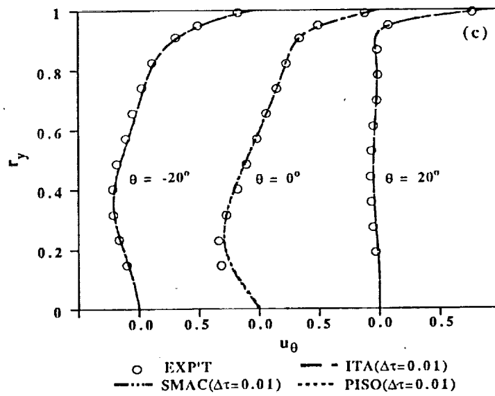
(c) u_\theta velocity profiles.
