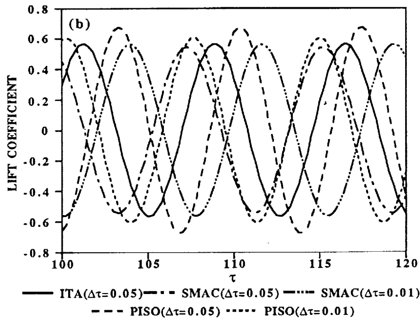
(b) Comparison of ITA, SMAC and PISO.
