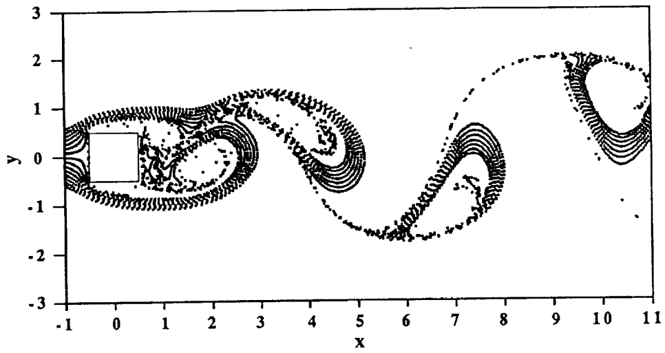
Figure 9.— Streaklines for flow over a square cylinder.
