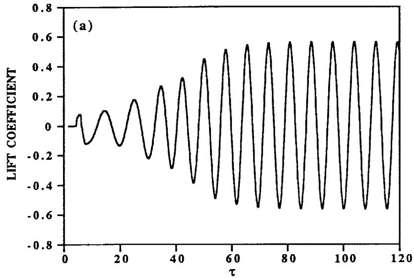
(a) SMAC ( \Delta\tau = 0.01 ).
