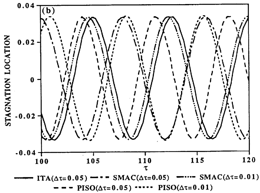
Figure 11.— Stagnation location for flow over a square cylinder.
