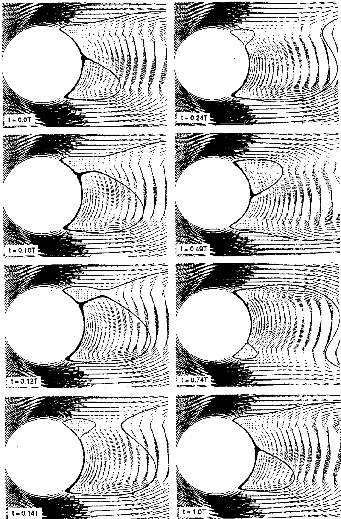
Figure 4.— Velocity vectors and instantaneous streamline contours passing through the separation and reattachment locations.
