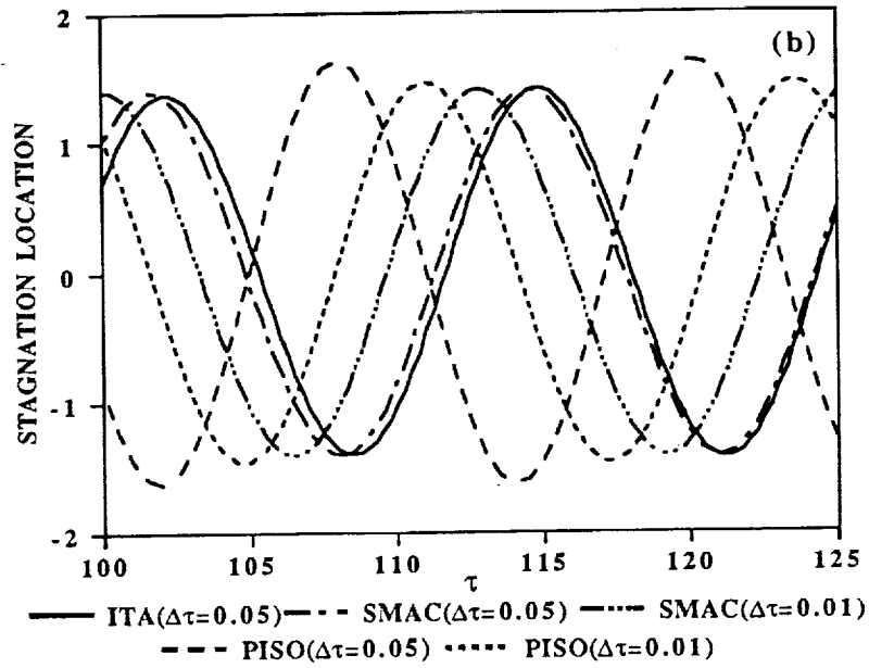
Figure 6.— Stagnation location for flow over a circular cylinder.
