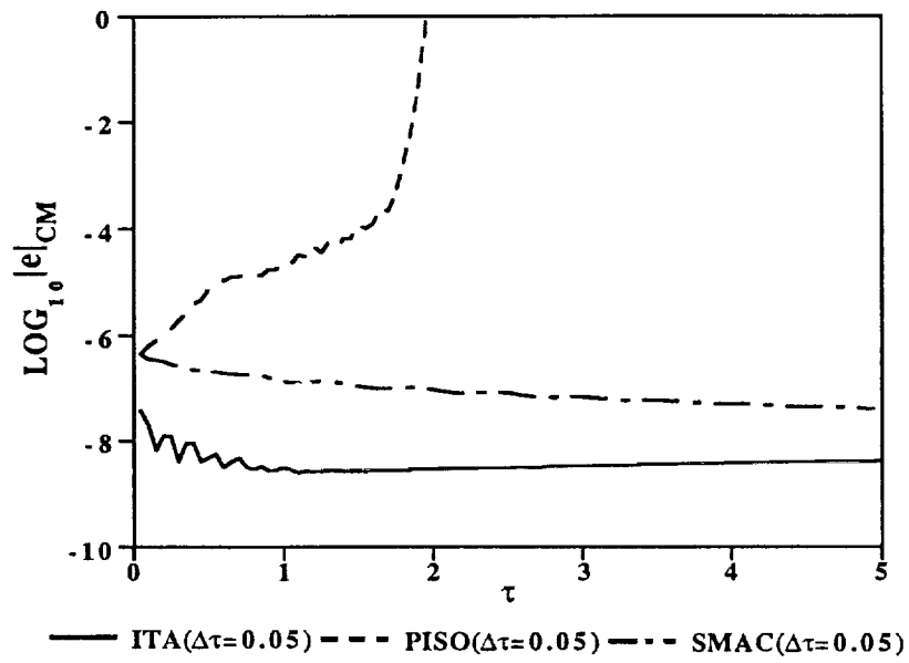
Figure 2.— Mass imbalance.
