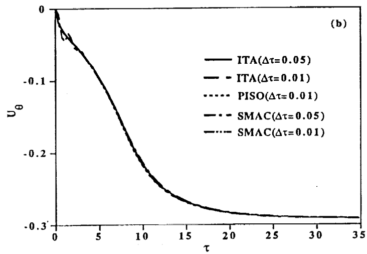
(b) Evolution of u_\theta at (r_y, \phi) = (0.246, 0) .
