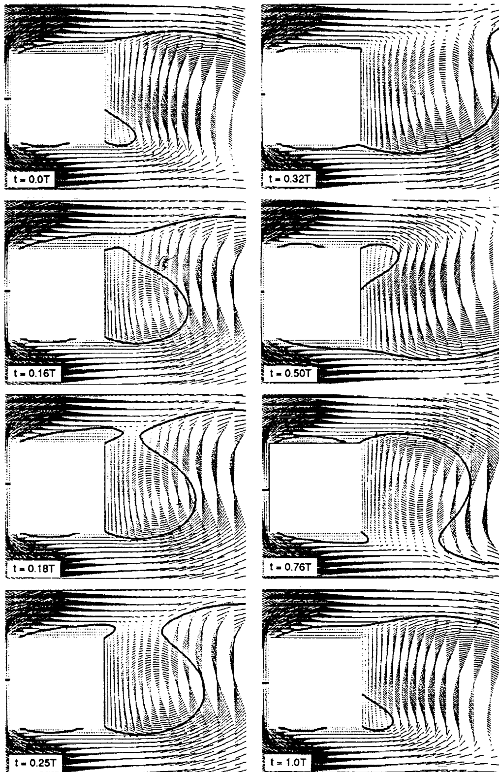
Figure 10.— Velocity vectors and instantaneous streamlines passing through the separation and reattachment locations.
